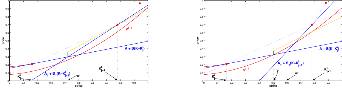
Figure 6: On the left: the case described in Step 1.3.a, where the yellow line represents the function \tilde{A}(\hat{\sigma}) + \tilde{B}(\hat{\sigma})(K - w) , for K \geq w , and the vertical interval in green represents the range of values of \tilde{A}(\sigma) , for \sigma \geq \hat{\sigma} . On the right: the case described in Step 1.3.b, where the yellow line represents the function \tilde{A}(\bar{\sigma}) + \tilde{B}(\bar{\sigma})(K - y) , for K \geq y , and the vertical interval in green represents the range of values of \tilde{A}(\sigma) , for \sigma \geq \bar{\sigma} .
