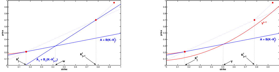
Figure 5: Visualization of the points w (on the left) and y (on the right). Red circles represent market time values for the current maturity. Red lines represent the already constructed time value interpolations.
