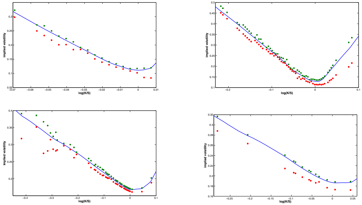
Figure 2: Implied volatility fit for the times to maturity: 2 (top left), 7 (top right), 47 (bottom left), and 67 (bottom right) working days. Blue lines represent the interpolated implied volatilities, red circles and green squares correspond to the bid and ask quotes, respectively.
