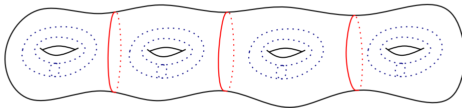
FIGURE 4: An S -compression body that has g(S) interior boundary components, all of which are tori. A compressing system is drawn in red, and the interior boundary is blue. All such compression bodies are isomorphic, although not all compressing systems look like the above.
