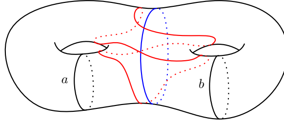
FIGURE 6: The two curves above are both meridians in only a single handlebody, while there are infinitely many separating curves that are disjoint from both.
