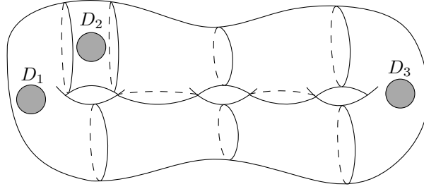
FIGURE 5: A handlebody with spots D_1, D_2, D_3 corresponding to the attachment of 1-handles. The non-separating meridians shown on the surface give a pants decomposition of the punctured surface obtained by deleting the spots from the boundary of the handlebody.
