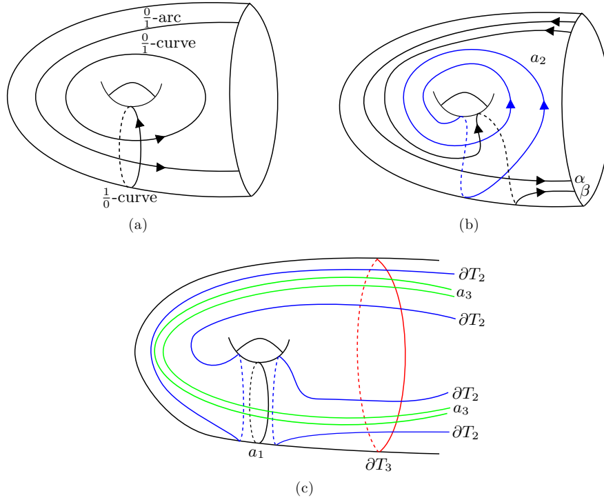
FIGURE 9: (a) A reference torus. (b) Drawn here is a_2, \alpha , and \beta with a_2 given an arbitrary orientation. As a_1 and a_3 live in a torus, the orientations of the intersections of \alpha and \beta with the \frac{1}{0} -curve must agree. (c) The region containing a_1 that is bounded by the blue and red curves is the intersection T_2 \cap T_3 .
