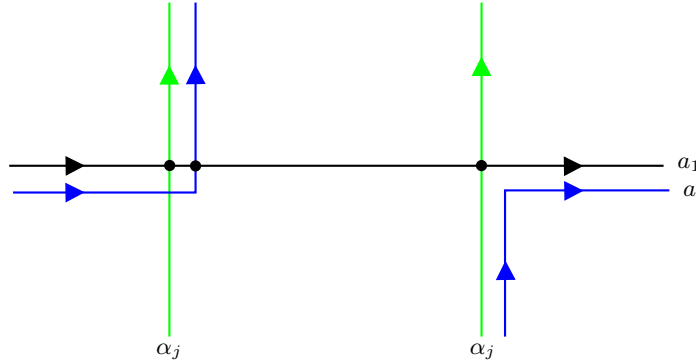
FIGURE 8: Shown here are two consecutive intersections between a_1 (black) and \alpha_j (green) and the curve a (blue) resulting from the following surgery: Begin at the intersection on the left, follow \alpha_j to the second intersection, and then following a_1 back to the first intersection. Notice that i(a_1, a) = 1 .
