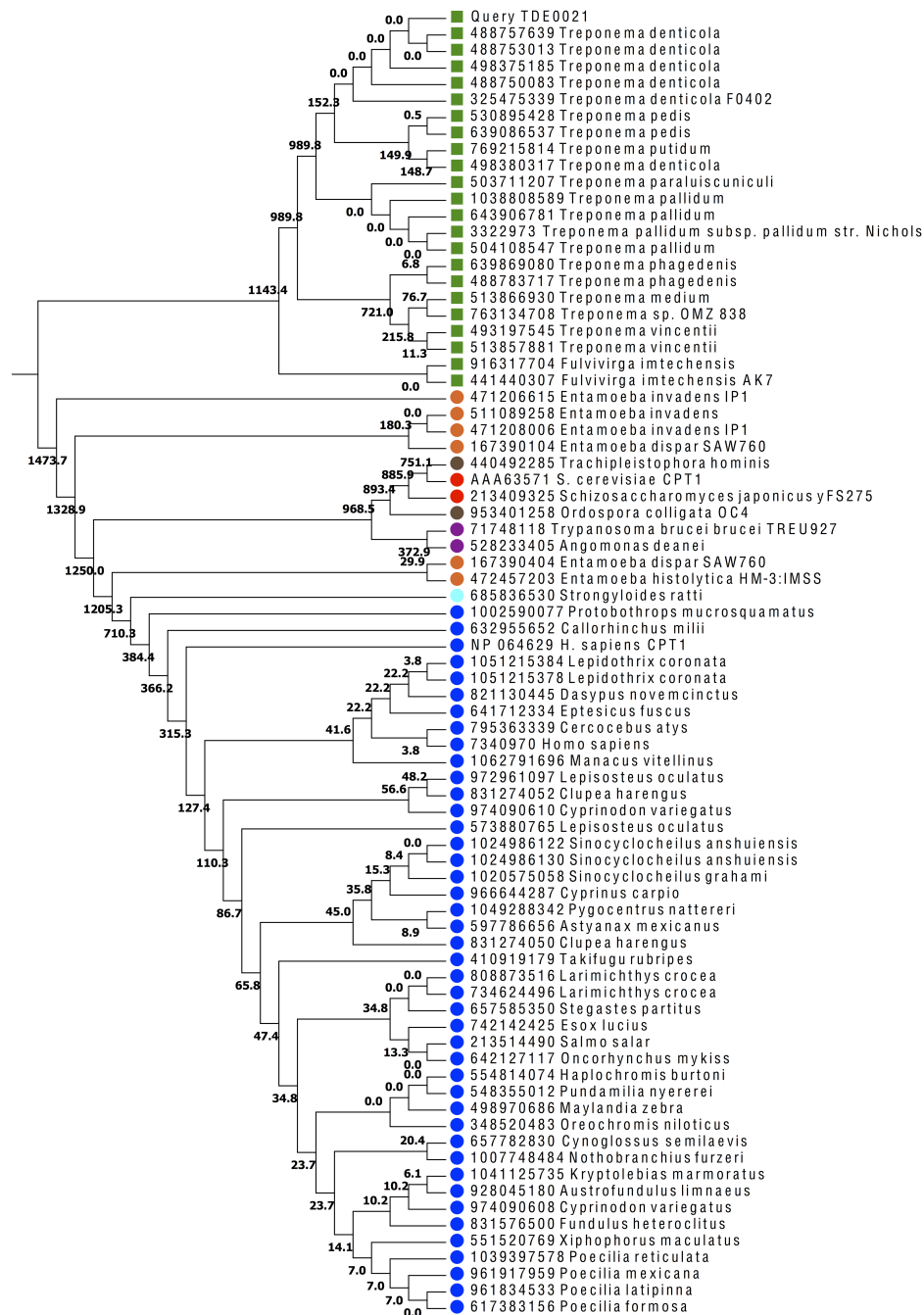
Fig. 8. Molecular dating analysis of TDE0021 homologues. The molecular dating analysis was carried out on an alignment generated by Maximum Likelihood (ML) phylogeny analysis as described in Experimental Methods. The bacterial sequences are marked with small circles before the tip labels (red: TDE0021 BLAST query; green: homologous sequences from other Treponema .) The numbers at the branches are the divergence time estimates for the nodes in millions of years. The color coding is as follows: green squares, Bacteria sequences; orange circles, Amoebozoa; brown circles, Microsporidia; purple circles, Euglenozoa; red circles, Ascomyceta; cyan (light blue) circles, Nematoda; blue circles, Chordata.
