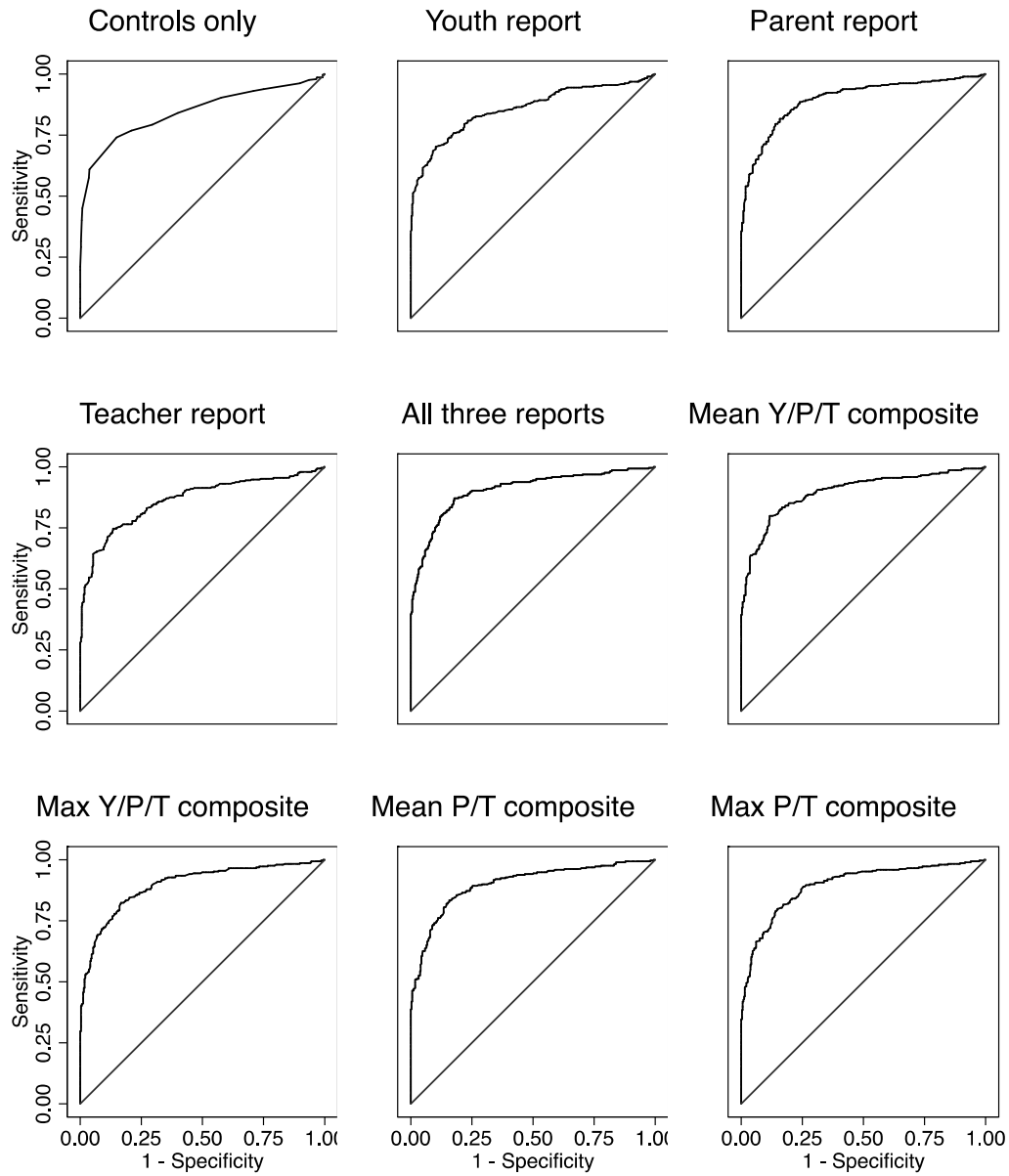
Figure 1. Receiver operating characteristic (ROC) curves for nine different logistic regression models predicting detained status from controls (age, binary sex, and binary race; included in all models) and various reports and composites of CU traits.
