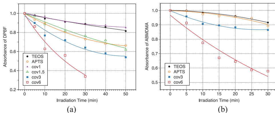
Figure 2. a) The ROS generation of different samples as indicated by the decay of absorbance of DPBF at 410 nm, and b) the ^1\text{O}_2 generation of different samples as indicated by the decay of absorbance of ABMDMA.
