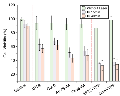
Figure 9. The viability of HeLa cells incubated with samples APTS and Cov6 with different surface modifications in dark, and under 15 min and 40 min irradiations, respectively.
