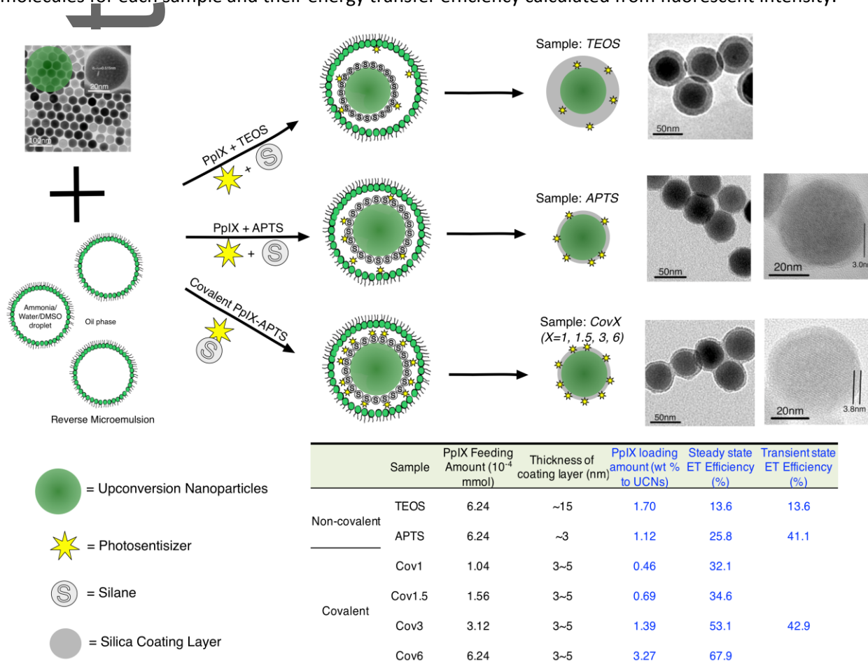
Figure 1. Schematic illustration of modified microemulsion approaches for coating silica and PS on upconversion nanoparticles. The inset table shows the feeding and loading amounts of PpIX molecules for each sample and their energy transfer efficiency calculated from fluorescent intensity.
