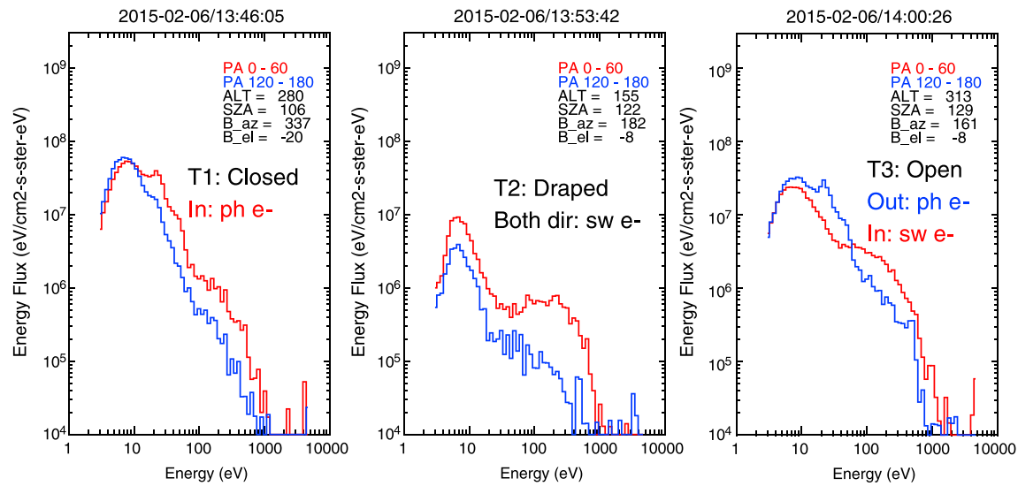
Figure 6. Electron energy spectra for parallel (red) and antiparallel (blue) directions measured by SWEA. The red spectrum is averaged over pitch angle 0–60° and the blue spectrum over pitch angle 120°–180°. The three plots corresponding to the time marked out by the three dotted vertical lines in Figure 5.
