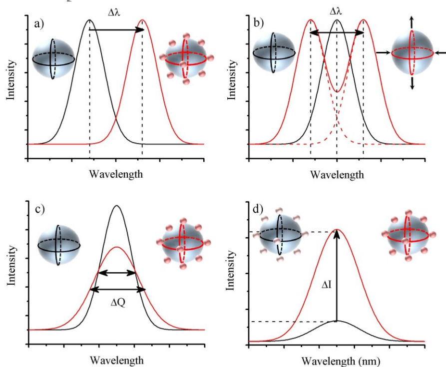
Figure 7. Sensing modalities used by fluorescent WGM resonators. (a) Resonance wavelength shift, (b) Mode-splitting, whereby applied stress to the resonator causes the degeneracy in the modes to be lost resulting in a broadening of the WGM peak, (c) variation in the Q-factor, and (d) Change in the mode intensity ( I ).
