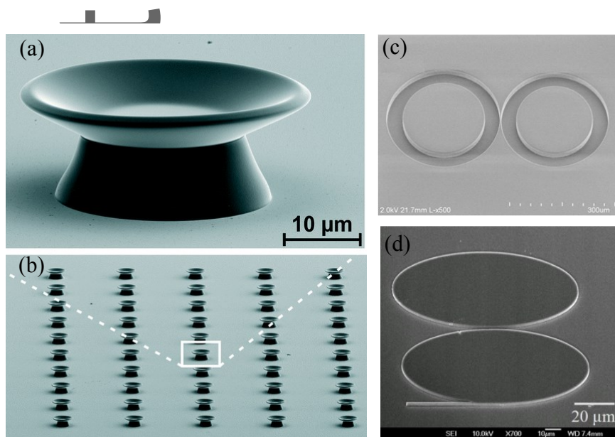
Figure 5. (a), (b) Fluorescent PMMA goblet resonators on a chip.[45] (c) Coupled ring resonators etched on fused silica and coated with a fluorescent dye-doped high refractive index polymer [31] and (d) coupled disk resonator with a protruding waveguide for directional emission.[35] (a), (b) Reproduced with permission from.[45] Copyright (2015), Royal Society of Chemistry. (c) Reproduced with permission from.[31] Copyright (2015), Nature Publishing Group. (d) Reproduced with permission from.[35] Copyright (2015), Elsevier.
