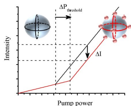
Figure 8. Variation of lasing characteristic induced molecular adsorption resulting in change of lasing threshold ( P_{\text{threshold}} ) and mode intensity ( I ).
