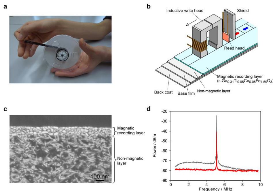
Figure 4. a) Picture of the manufactured magnetic recording tape composed of \epsilon\text{-Ga}_{0.31}\text{Ti}_{0.05}\text{Co}_{0.05}\text{Fe}_{1.59}\text{O}_3 . b) Schematic illustration of the LTO-3 AMR head composed of an inductive write head, a read head, and a shield. c) Cross section SEM image of the manufactured magnetic tape. d) Power spectrum of the signal of the \epsilon\text{-Ga}_{0.31}\text{Ti}_{0.05}\text{Co}_{0.05}\text{Fe}_{1.59}\text{O}_3 tape (red line) and cobalt-iron alloy tape (grey line) measured with the LTO-3 AMR head.
