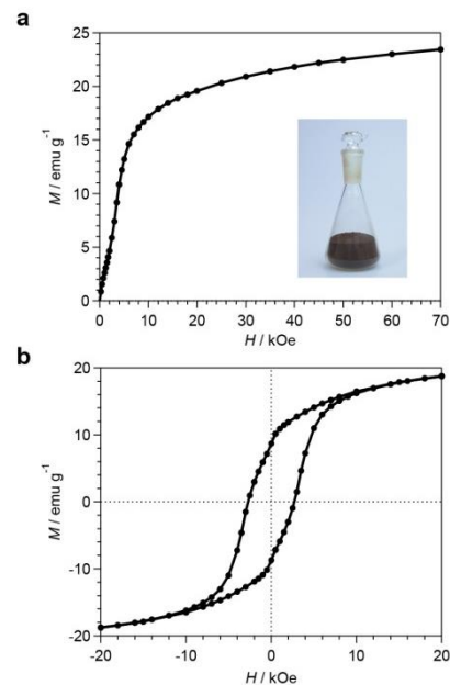
Figure 2. a) Initial magnetization curve and b) magnetic hysteresis loop of \epsilon - \text{Ga}_{0.31}\text{Ti}_{0.05}\text{Co}_{0.05}\text{Fe}_{1.59}\text{O}_3 measured at 300 K. Inset of (a) is a picture of the powder sample.
