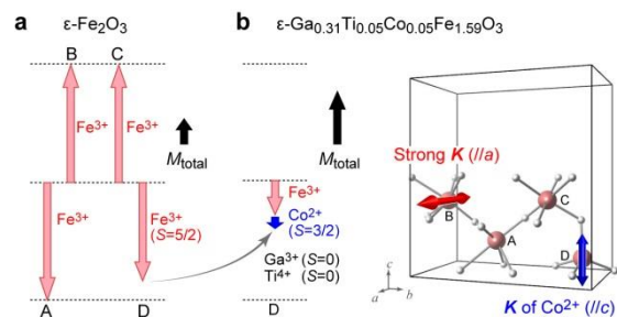
Figure 3. Magnetic structure of \epsilon - \text{Fe}_2\text{O}_3 (a) \epsilon - \text{Ga}_{0.31}\text{Ti}_{0.05}\text{Co}_{0.05}\text{Fe}_{1.59}\text{O}_3 (b, left). Red and blue arrows denote the sublattice magnetizations of \text{Fe}^{3+} and \text{Co}^{2+} , respectively. Upward (downward) arrows denote the positive (negative) sublattice magnetization. Black arrows show the total magnetization. Right figure in (b) shows the asymmetric unit in the unit cell denoting the direction of the single ion anisotropies ( K , red and blue arrows) for \text{Fe}^{3+} at the B site along a -axis and \text{Co}^{2+} at the D site along c -axis.
