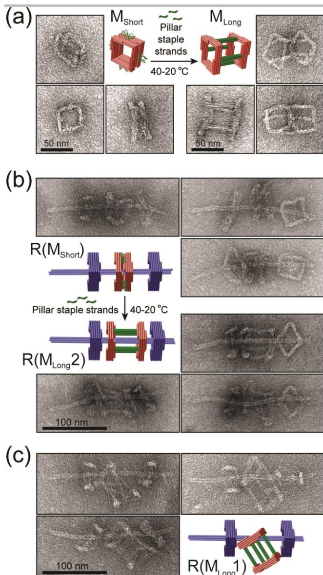
Figure 4. Assembling DNA origami rotaxanes with a tubular macrocycle. (a) Structural reconfiguration of a macrocycle by folding its unpaired scaffold loops into rigid 4-helix bundle pillars. Close-up TEM images show the typical appearances of monomeric macrocycles before and after reconfiguration. (b) Elongating a macrocycle of a complete DNA rotaxane. Close-up TEM images show the typical appearances of rotaxanes before and after reconfiguration. (c) Rotaxanes assembled using an elongated tubular macrocycle as a starting component. Note the different topologies of rotaxanes shown in (b) and (c).
