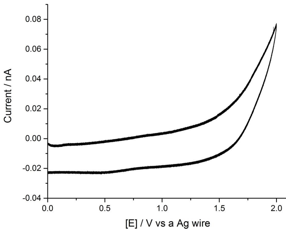
Figure S1: A Cyclic Voltammogram of 2000 MW PEG Ag NPs after a 10 min wait period – measured at 10 mVs -1 on a microcarbon electrode with a silver wire (pseudo-reference and counter electrode).
