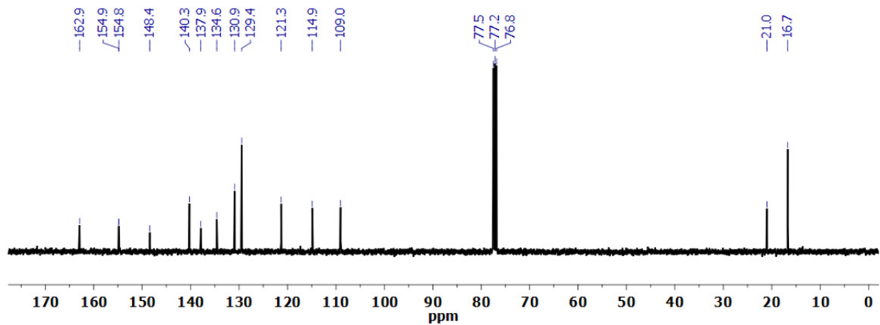
Figure S9: 100 MHz ^{13}\text{C} NMR spectrum of \text{Tpy}^{0\text{Mes}} collected at 25^\circ\text{C} in \text{CDCl}_3 .
