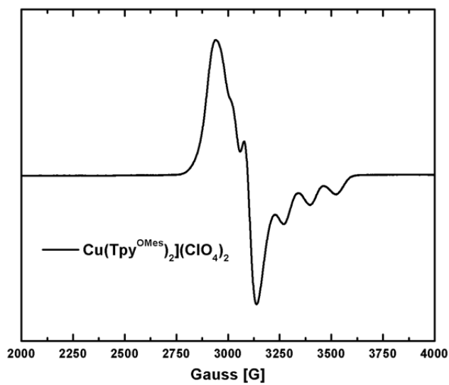
Figure S26: EPR spectrum of 6 collected in CH 2 Cl 2 at 120K.
