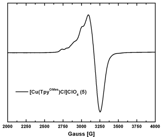
Figure S25: EPR spectrum of 5 collected in CH 2 Cl 2 at 120K. Sample was prepared by dissolving 5 in CH 2 Cl 2 , quickly filtering, and freezing in liquid N 2 .
