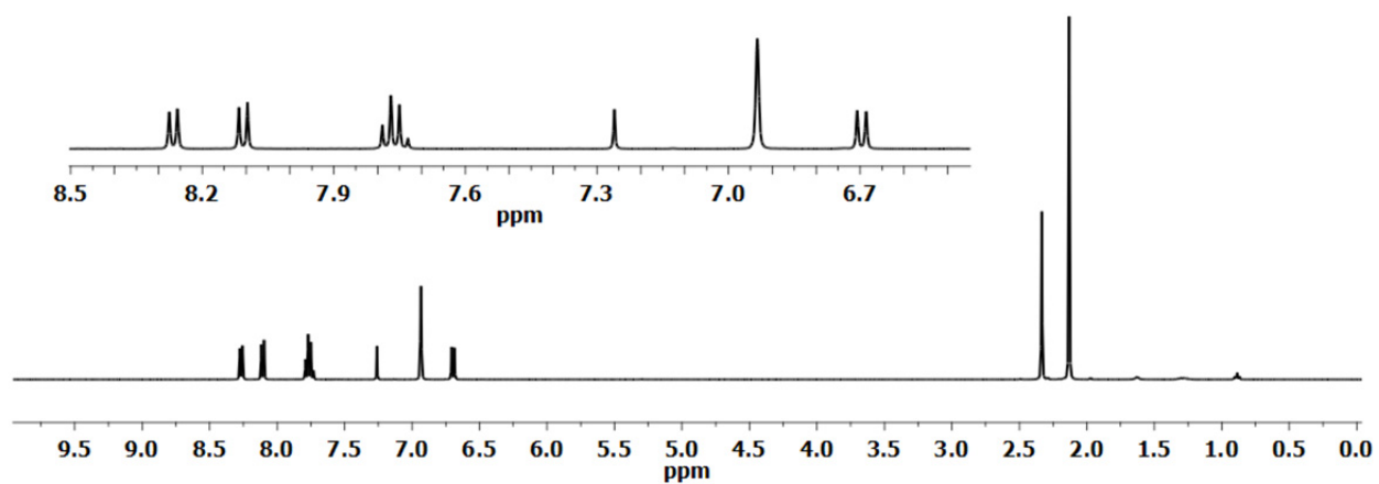
Figure S8: 400 MHz ^1\text{H} NMR spectrum of \text{Tpy}^{0\text{Mes}} collected at 25^\circ\text{C} in \text{CDCl}_3 .
