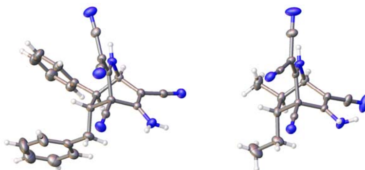
Figure 5. ORTEP view of molecular structure of polysubstituted isoquinuclidines anti-3a' and anti-3b' .
