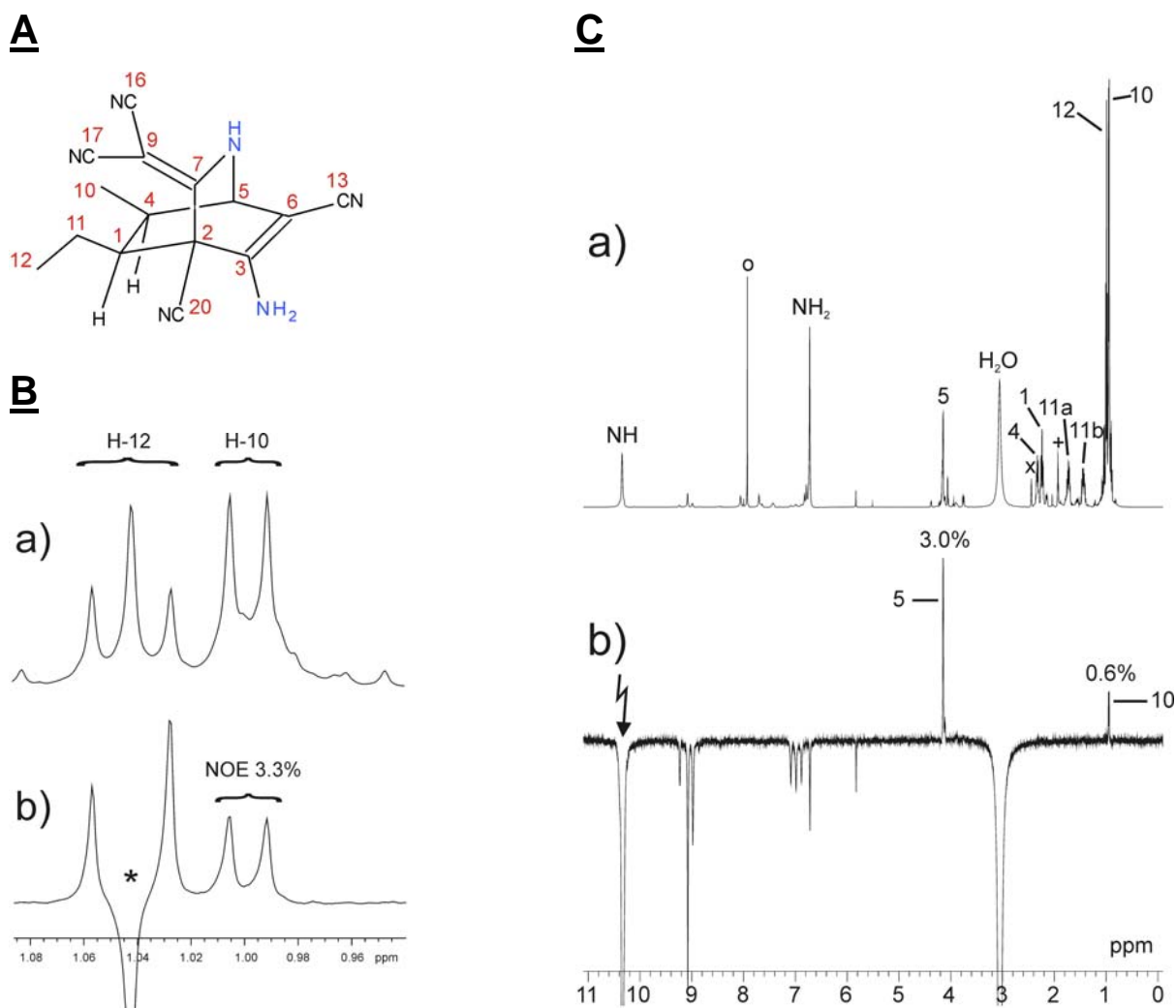
Figure 6. A Numbering of syn-3b'' as automatically suggested by the NMRPredict software and as is employed for the depicted/described NMR spectra. B ^1\text{H} -NMR spectrum (500 MHz) of syn-3b'' , zoomed signals of H-12 (ethyl- \text{CH}_3 ) and H-10 (methyl) in \text{DMSO-d}_6/\text{CD}_3\text{CN} 1:2, r.t. a) normal ^1\text{H} -spectrum; b) DPFGE-NOE spectrum under irradiation of H-11b (one of the diastereotopic \text{CH}_2 -protons). The percentage number is relative to the intensity of the irradiated signal = -100%. The * denotes a selective population transfer (SPT) effect from vicinal coupling. Measuring time for the NOE spectrum: 5 hrs. C ^1\text{H} -NMR spectrum (500 MHz) of syn-3b'' in \text{DMSO-d}_6/\text{CD}_3\text{CN} 1:2, r.t. a) normal ^1\text{H} -spectrum with assignments according to A o = \text{CHCl}_3 (from synthesis/workup); x = residual solvent signal ( \text{DMSO-d}_6 ); + = residual solvent signal ( \text{CD}_3\text{CN} ); b) DPFGE-NOE spectrum under irradiation of the NH signal. Negative signals are due to chemical exchange with other acidic protons from isomerization/decomposition products. Percentage numbers of positive NOE signals at H-5 and H-10 are relative to the integral sum of all negative signals = -100%. Mixing time 0.5 sec, measuring time 22 hrs.
