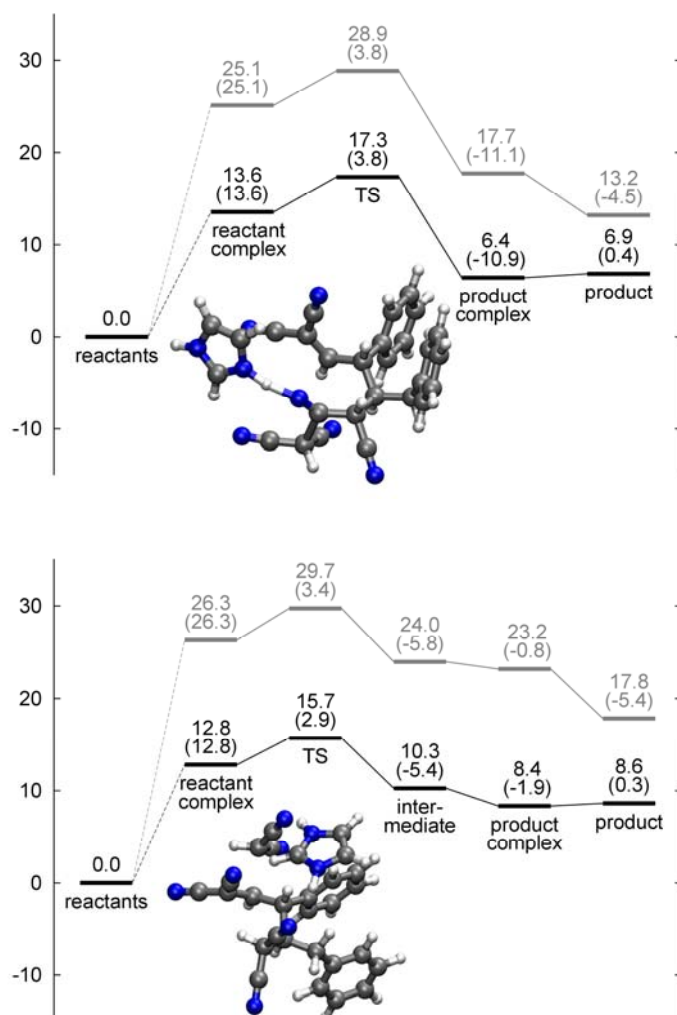
Figure 9. Reaction profiles of the nucleophilic addition reaction (upper graph) and Michael addition (lower graph), catalyzed by imidazole, respectively. Free energies (in kcal/mol) are relative to the reactants (most stable conformer 6 + imidazole + malononitrile). The free energies are also given relative to the reactant level or the previous species (in parenthesis). The black line represents the profile including, the grey line without van der Waals corrections. Additionally, the structures of the respective transition states are shown.
