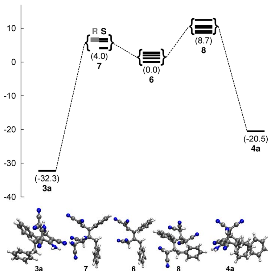
Figure 8. Free energies (in kcal/mol) of the most stable conformers relative to the most stable conformer of 6 . In case of the addition product 7 the R and S configurations on the C atom marked by an asterisk in Fig. 7 were considered.
