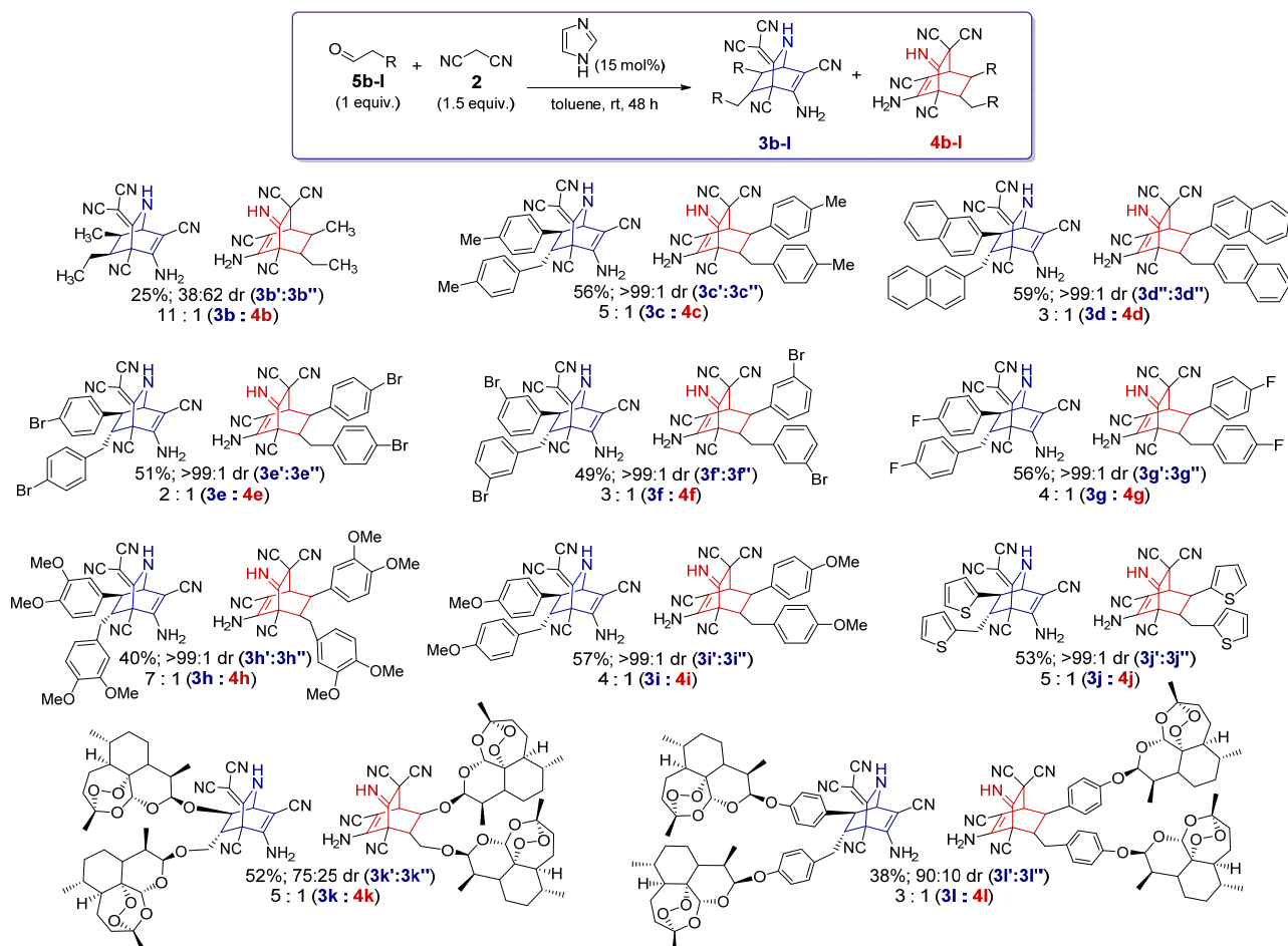
Figure 4. Substrate scope includes various aldehydes 5b-5l . Reported yields were isolated yields of products, sum of 3 and 4 . Ratio 3:4 and dr were determined by ^1\text{H} NMR analysis of the product mixture after a single column, see Supplementary Information for more details.
