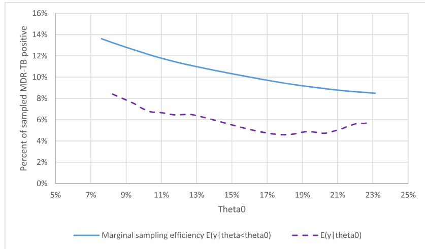
FIGURE 3 Sampling efficiency and marginal sampling efficiency at different proportions of TB+ patients being tested for MDR-TB ( \theta ). MDR-TB = multidrug resistant TB; TB = tuberculosis. [Colour figure can be viewed at wileyonlinelibrary.com ]
