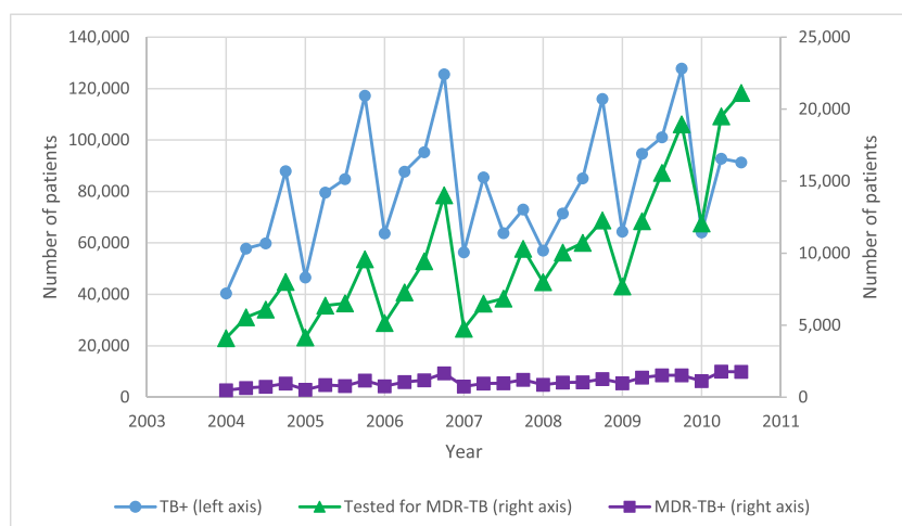
FIGURE 1 Number of patients who are TB-positive, tested for MDR-TB, and MDR-TB-positive by quarter over time. MDR-TB = multidrug resistant TB; TB = tuberculosis. [Colour figure can be viewed at wileyonlinelibrary.com ]
