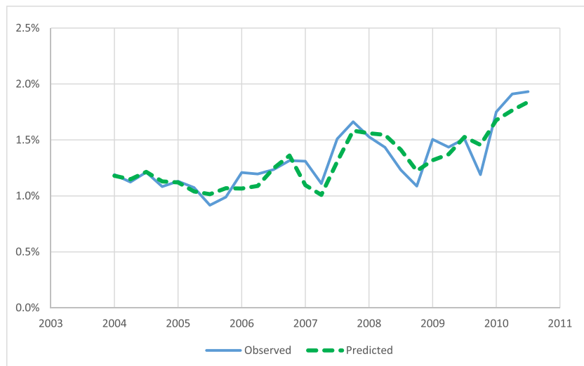
FIGURE 5 Observed MDR-TB prevalence over time in National Health Laboratory Service data compared to MDR-TB prevalence estimated from maximum likelihood estimation. MDR-TB = multidrug resistant TB; TB = tuberculosis. [Colour figure can be viewed at wileyonlinelibrary.com ]
