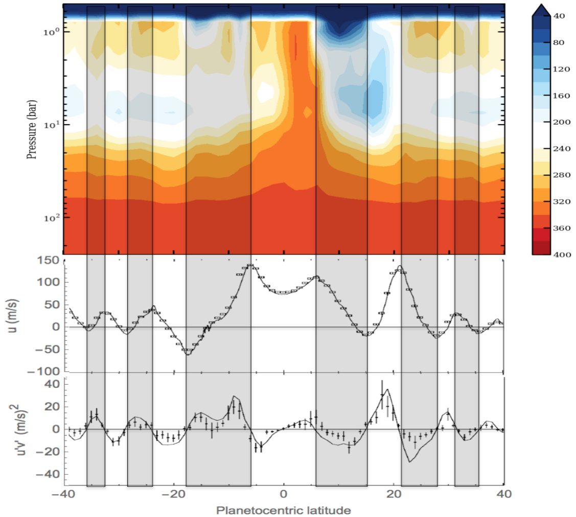
Figure 1. Top: molar mixing ratio of ammonia in parts per million with color code at right [Bolton et al. , 2017; Janssen et al. , 2017; Li et al. , 2017]. Middle: zonal wind profile \bar{u}(y) , where y is the northward coordinate [Salyk et al. , 2006]. Bottom: eddy velocity covariance \overline{u'v'} (points, units \text{m}^2 \text{s}^{-2} ) and velocity gradient d\bar{u}/dy (smooth curve, units 10^{-6} \text{s}^{-1} ), from Salyk et al. [2006]. The gray bands are where the zonal winds are cyclonic ( d\bar{u}/dy < 0 in the north and d\bar{u}/dy > 0 in the south). The white bands are anticyclonic.
