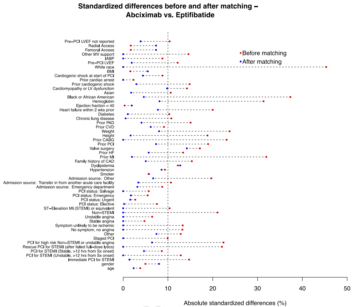
Figure 2: Plot of absolute standardized differences before and after matching.
