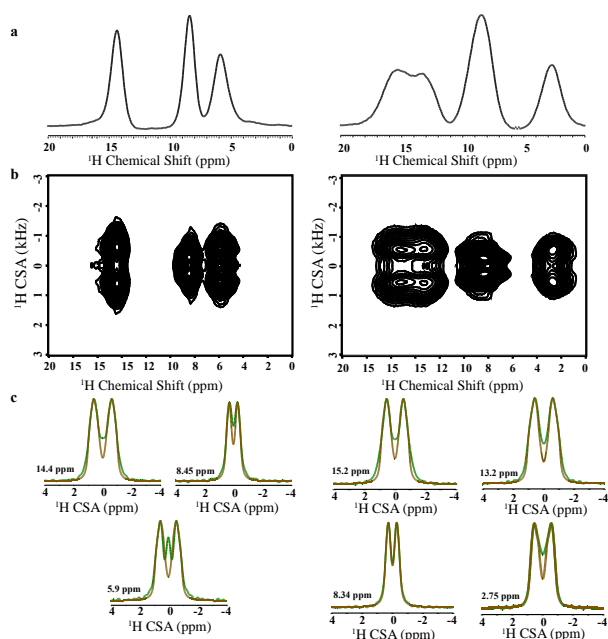
Figure 2. 1 H chemical shift anisotropy spectra of monohydrate (left) and hemihydrate (right) of mercaptopurine. (a) 1D isotropic 1 H spectra collected under 90 kHz MAS. (b) 2D 1 H CS/CSA correlation spectra obtained using the RF pulse sequence given in ESI Figure S1. (c) 1 H CSA lineshapes, extracted from 2D 1 H CS/CSA spectra (green), associated with the indicated isotropic chemical shift values, and their simulated best fits obtained using SIMPSON (brown). All other experimental details are given in the Supporting Information.
