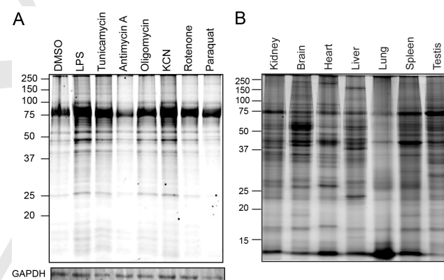
Figure 4. Profiling S-sulfination in stimulated cells and tissues. (A) Stimulus-dependent induction of protein S-sulfination in RAW 264.7 cells (24 hr); LPS (100 ng / mL), tunicamycin (10 \mu M), antimycin A (50 \mu M), oligomycin (5 \mu Mds), KCN (1 mM), rotenone (1 \mu M), and paraquat (40 \mu M). (B) S-sulfination profile across different mouse tissues.
