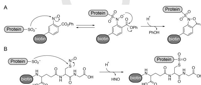
Scheme 1. Nitroso-directed methods for labeling endogenous S-sulfinated cysteine residues in proteins. (A) Aryl-nitroso probes react with protein sulfinic acids to form a stable benzoxazolone ring. (B) S-nitrosoglutathione probes react with protein sulfinic acids to form a thiosulfonate linkage.
