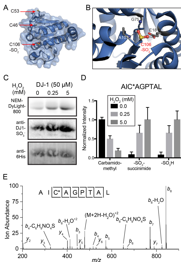
Figure 3. Analysis of sulfonyl succinimide formation on recombinant human DJ-1. (A) Structure of DJ-1 (PDB: 1SOA) highlighting the three encoded cysteines. Cys46 and Cys53 are surface exposed, while Cys106 is buried in the putative active site. (B) DJ-1 Cys106 forms a stabilized sulfenic acid through a network of hydrogen bonds. (C) Profiling S-sulfination of DJ-1 by sequential alkylation with IAM and maleimide-DyLight 800. Recombinant DJ-1 was pretreated hydrogen peroxide, followed by DTT, IAM, and maleimide-DyLight 800 to detect sulfenic acids. (D) Label-free mass spectrometry quantitation of DJ-1 Cys106 oxidation summed and normalized from the pepsin digested peptides AICAGPTAL AND AICAGPTALL. Error bars represent standard deviations from 4 biological replicates. (E) Collision-induced dissociation MS/MS spectra of the DJ-1 N -ethyl-3-(sulfonyl-Cys106)succinimide conjugated peptide (AIC*AGPTAL). (* = sulfonyl-succinimide).
