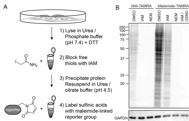
Figure 2. Sequential alkylation strategy for detection endogenous S -sulfination. (A) Schematic of sequential alkylation strategy for labeling endogenous S -sulfinated proteins. Proteins are denatured in 6 M urea / PBS buffer (pH 7.4) for IAM labeling, then precipitated and resuspended in 6 M urea / citrate-phosphate buffer (pH = 4.5) for maleimide labeling. (B) IAM-TAMRA and Maleimide-TAMRA (50 \mu M) labeling of HEK-293T cell lysates after pre-treatment (30 min) with various electrophiles. IAM-TAMRA (50 \mu M), IAM (50 mM), NEM (50 mM), and GSNO (200 \mu M).
