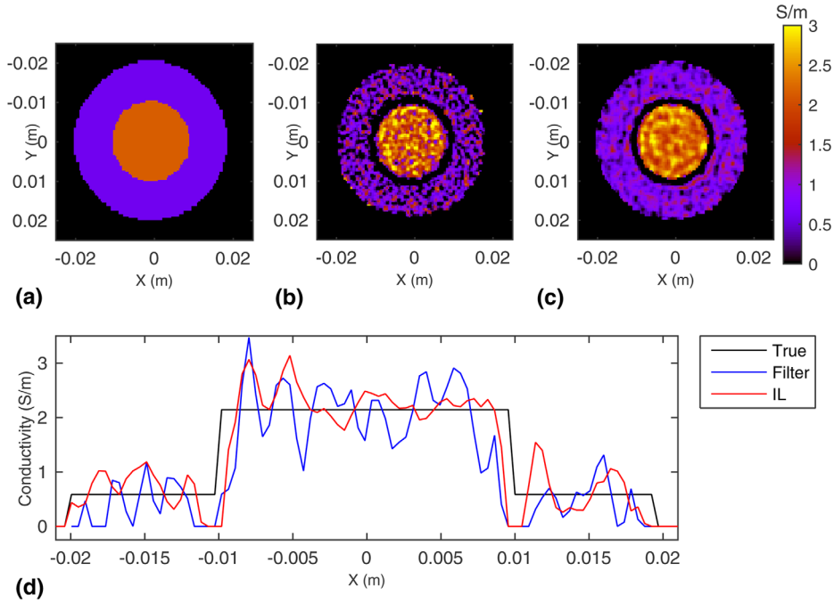
FIG. 2. Conductivity maps for the simulation experiments. AWGN was added to the complex data with standard deviation = 5 \times 10^{-4} . a : True conductivity. b : Restricted Gaussian filter reconstruction. c : Inverse Laplacian reconstruction. d : Profiles through y=0 .
