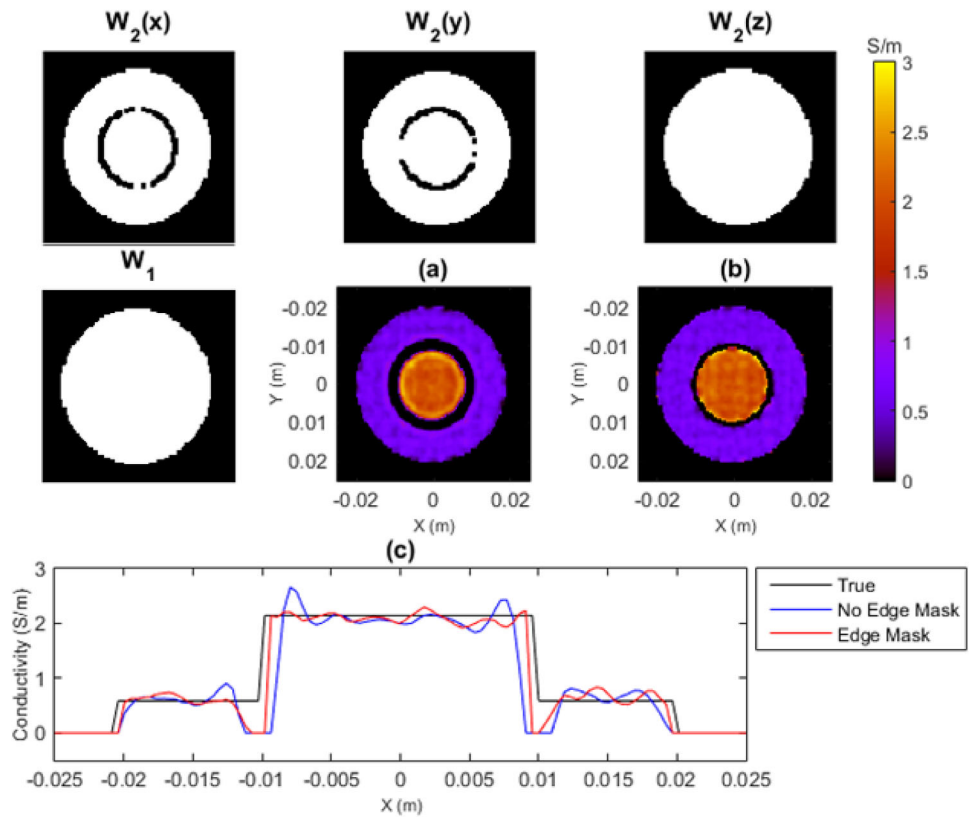
FIG. 4. Conductivity maps reconstructed with the Inverse Laplacian method for the simulation experiments. AWGN was added to the complex data with standard deviation = 10^{-4} . Masks W_1 and W_2 are shown, where W_2 provides weightings for regularization in three dimensions independently. a: Only support mask, W_1 , used in the reconstruction. b: Both masks, W_1 and W_2 , used in the reconstruction. c: Profiles through y = 0 .
