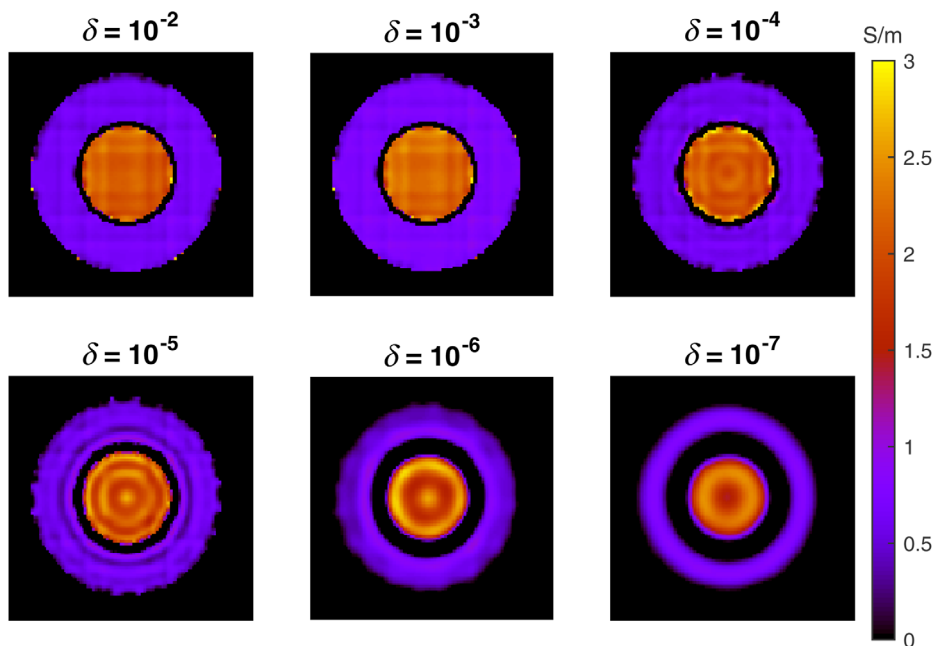
FIG. 3. Conductivity maps reconstructed with the Inverse Laplacian method for the simulation data with varying values for the offset added to the DC coefficient. No noise was added to the simulation data. The DC offset was varied between 10^{-2} and 10^{-7} .
