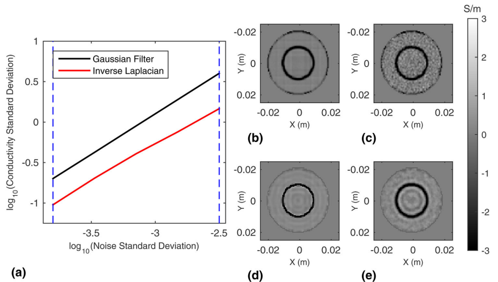
FIG. 5. Measures of error due to noise and bias in both reconstruction methods. a: Standard deviation of conductivity map error as a function of the standard deviation of the AWGN added to the complex simulated B_1^+ fields. b–e: Mean conductivity map error over all realizations for two noise standard deviation levels to show the bias of the Gaussian filter, (b) and (c), and Inverse Laplacian method, (d) and (e). Mean values are calculated for the lowest, (b) and (d), and highest, (c) and (e), noise levels as denoted by blue dashed lines in (a).
