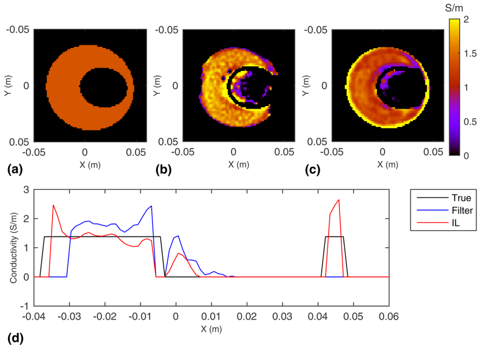
FIG. 6. Conductivity maps for the experimental phantom. a: True conductivity. b: Restricted Gaussian filter reconstruction. c: Inverse Laplacian reconstruction. d: Profiles through y=0 .
