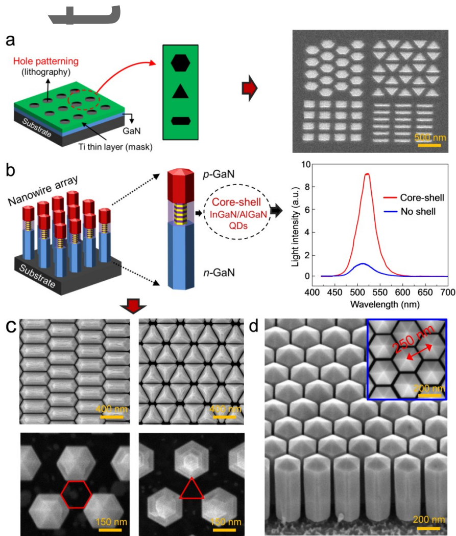
Figure 1. a) Schematic illustration of hole patterned Ti thin film mask for the selective area epitaxy of InGaN photonic crystals. SEM image of various nanoscale patterns formed on the Ti mask is shown in the right panel. b) Illustration of bottom-up InGaN/AlGaN core-shell dot-in-nanowire array grown on patterned
