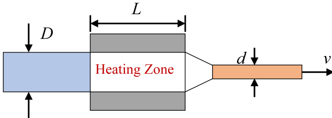
Figure 4: Heating zone for the plastics extrusion process (sometimes called fused deposition modeling – FDM). The cylindrical filament enters as a solid with diameter D on the left, is heated by conduction from the wall in a zone of length L and exits as a molten polymer of diameter d and velocity v on the right.
