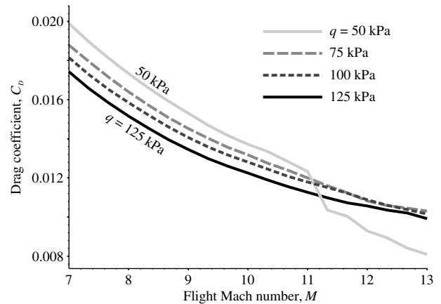
Fig. 14 Vehicle drag coefficient for the optimum trajectory at four dynamic pressures.
