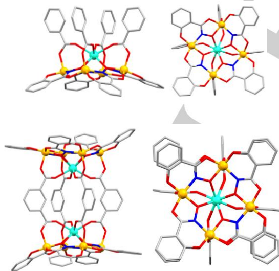
Figure 2. Structures of \text{DyGa}_4 MC (top) and [\text{DyGa}_4]_2 dimeric complexes (bottom) obtained from X-ray diffraction on single crystals: (left) side-view and (right) top-down view of the 12-MC-4 core. Color code: Ga, yellow; Dy, teal; O,
