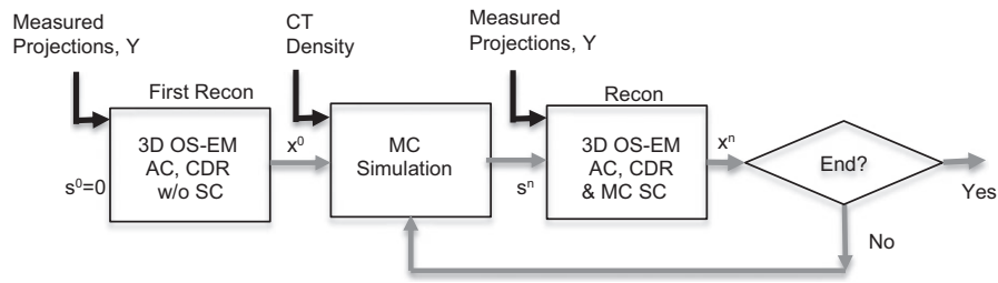
FIG. 1. Flowchart illustrating combination of Monte Carlo scatter estimation with an analytical forward projector.
