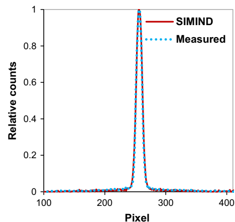
FIG. 3. Profile (10-pixel wide) across the measured and simulated line source. Profiles have been normalized to their maximum value. [Color figure can be viewed at wileyonlinelibrary.com ]
