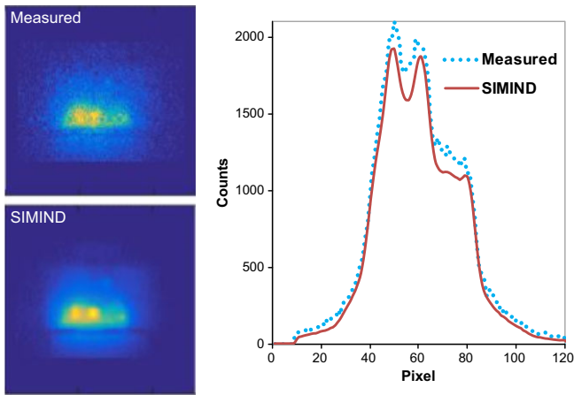
FIG. 4. Measured and simulated projection images (at 0°) of the liver phantom and corresponding line profiles. Profiles were summed over 10 bins centered on the center sphere. [Color figure can be viewed at wileyonlinelibrary.com]
