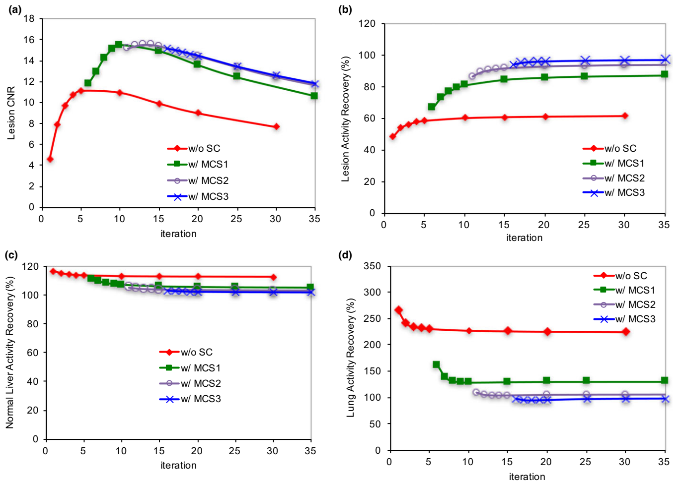
FIG. 5. (a) Lesion CNR, (b) lesion activity recovery, (c) normal liver activity recovery and (d) lung activity recovery for the different reconstructions of the phantom data. [Color figure can be viewed at wileyonlinelibrary.com]
