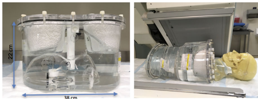
FIG. 2. The liver/lung torso phantom (left) was positioned in-between a skull and elliptical phantom for SPECT/CT imaging (right). [Color figure can be viewed at wileyonlinelibrary.com]
