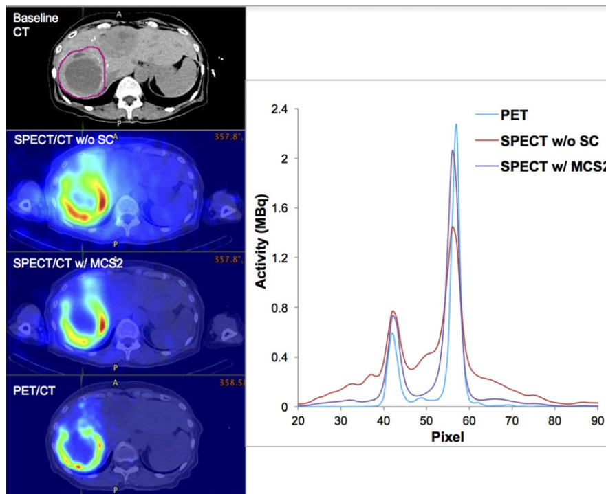
FIG. 8. For patient #3 the SPECT reconstruction without and with scatter correction is compared with 90 Y PET. Profiles are across the center of the large necrotic lesion contoured on the catheter directed selective hepatic arterial contrast enhanced CT. [Color figure can be viewed at wileyonlinelibrary.com]
