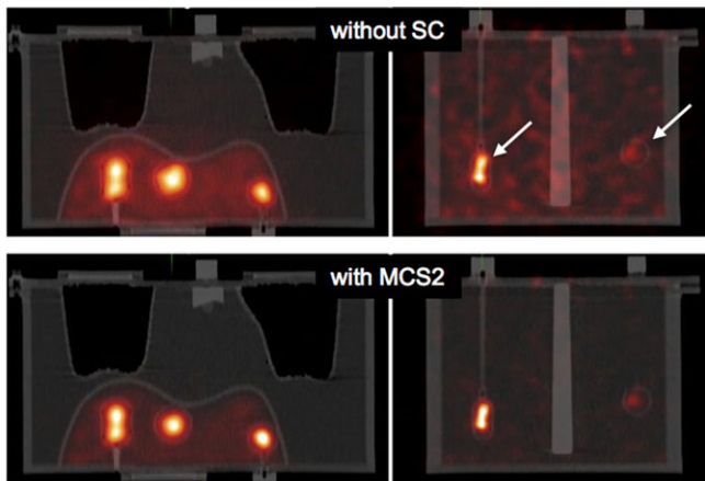
FIG. 7. Coronal SPECT/CT slices without (top row) and with (bottom row) scatter correction, demonstrating visibility of the hepatic lesions (left) and the extra hepatic objects (right). [Color figure can be viewed at wileyonlinelibrary.com ]
