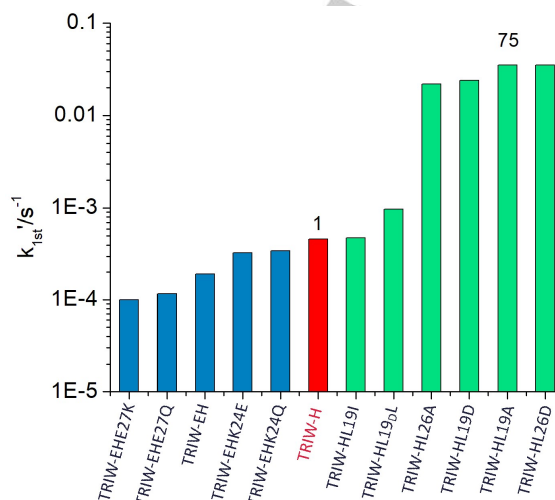
Figure 2. Pseudo-first order rate constants at pH 5.8 for the original construct TRIW-H (red), previously reported exterior mutations (blue), and currently reported interior mutations [15] (green).
