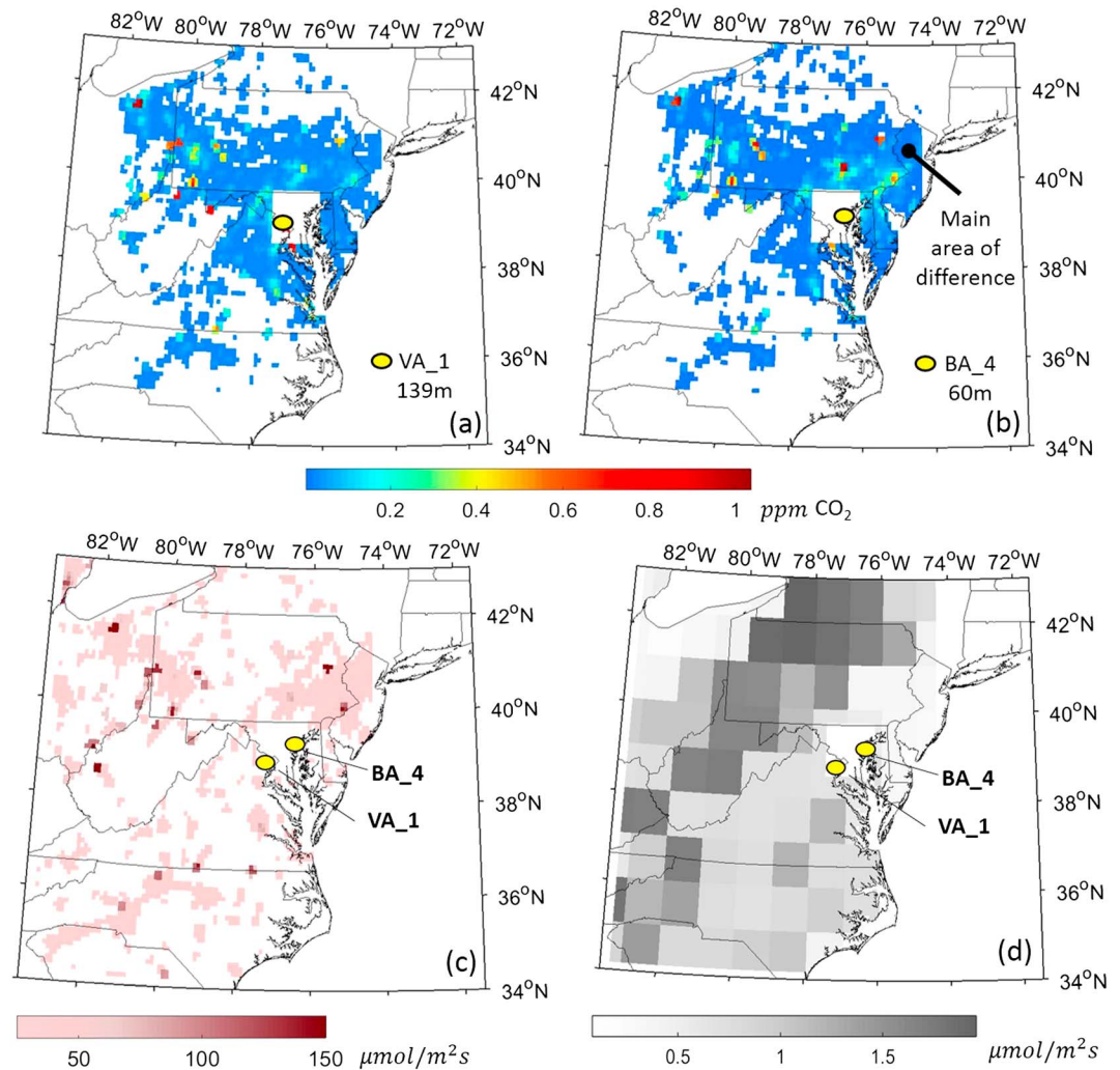
Figure 5. The average monthly contributions (ppm) from different source and sink locations outside the NEC-B/W urban domain to the hourly CO 2 mole fractions as observed for February 2013 at NEC-B/W towers (a) VA_1 (139 m AGL) and (b) BA_4 (60 m AGL) whose sites are denoted by the yellow circle within the urban domain. White areas are areas that have less than a 0.015 ppm contribution to modeled enhancements at these two towers. The monthly averaged (c) Vulcan 2.2 emissions and (d) CarbonTracker (CT) 2013b, respectively, used to create the synthetic observations for February. July contributions are provided in supporting information Figure S3.
