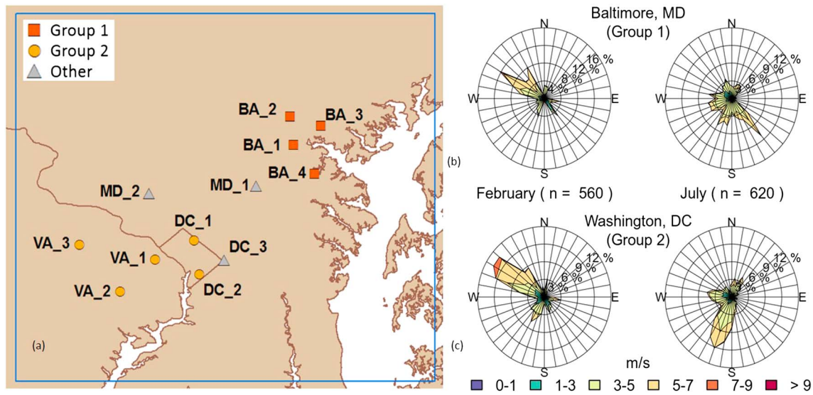
Figure 4. (a) Location of the three groups of NEC-B/W towers as identified by the correlation coefficients and root-mean-square differences of their CO 2 mole fraction time series representing sources and sinks from outside the urban domain. (b and c) The averaged wind roses associated with group 1 (39.33°N, 76.66°W) and group 2 (38.96°W, 77°N) towers generated from the WRF modeled output described in section 2.1 for the months of February and July.
