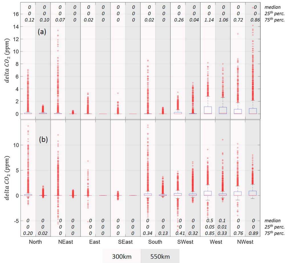
Figure 6. Boxplots of the simulated average contributions to all 12 NEC-B/W mole fractions ( y_{ex} ) from extraurban sources and sinks from different directions for (a) February and (b) July 2013. Far-field contributions (300 km to 550 km) are in the dark gray rectangle boxes, while the intermediate fields (urban domain to 300 km) are in the light gray rectangles. Red lines indicate the median with dashed bars indicating the 5th and 95th percentiles and outliers as red plus symbols. The median and 25th and 75th percentiles for February and July are also noted on each subplot. Note that although median values are small and marginally similar, the extreme outliers have large impacts on the variability of the CO_2 enhancements as observed at the NEC-B/W tower sites.
