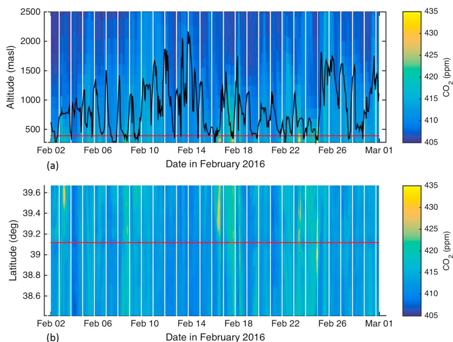
Figure 8. (a) Projected CO 2 mole fractions (ppm) for the location of BG_1. UTC (local time + 5 h) time is represented on the x axis and altitude (meters above sea level) on the y axis. The color represents mole fractions in parts per million throughout the vertical column, and the white lines indicate local noontime periods throughout the month. The black solid line is the PBL, and the pink line is the inlet height at BG_1. (b) Projected CO 2 concentrations (ppm) along the western NEC-B/W boundary. The pink line indicates the latitude of the BG_1 along this wall. This figure for February 2016 provides an example of the variability in time and space of incoming CO 2 that is representative of the winter period (February 2013) used in this study.
