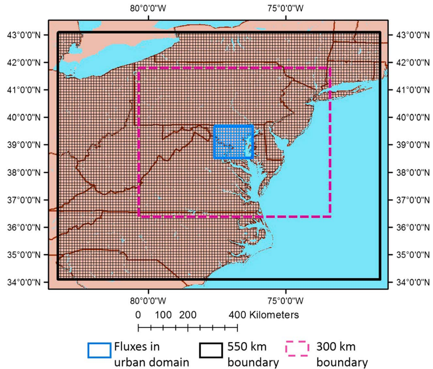
Figure 2. Representation of the two main areas for this study, that is, the urban and extraurban domains. y_{fossil\_ex} and y_{bio\_ex} are the CO 2 enhancements that enter the NEC-B/W urban domain due to sources and sinks (located in small black boxes) between the outer domain (thick black rectangle) and the NEC-B/W urban area (blue rectangle), and y_{fossil\_urb} and y_{bio\_urb} are mole fraction enhancements at the NEC-B/W towers from sources and sinks in the NEC-B/W urban domain (blue box). The work presented also examines the influence of intermediate-field (300 km from the blue box, between blue and thick dashed magenta rectangle) and far-field (300 km to 550 km which is the area between the thick magenta dashed and thick black rectangle) fluxes on CO 2 enhancements observed at the NEC-B/W tower sites (section 3.2).
