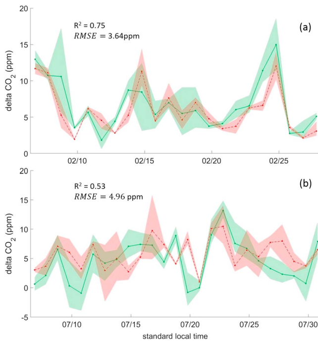
Figure 7. Estimated “background” time series (modeled background using mole fractions from selected background towers, dashed red line with points) and y_{ex} (green line with points, aka truth) as averaged across the urban towers for (a) February and (b) July. Daily mean averages of afternoon observations (12 p.m. to 5 p.m. local time) are shown. The shading around the red and green lines represent the maximum and minimum modeled enhancements for a given afternoon period. Note that although the modeled background generally captures the truth, there are large deviations at specific times in each month.
