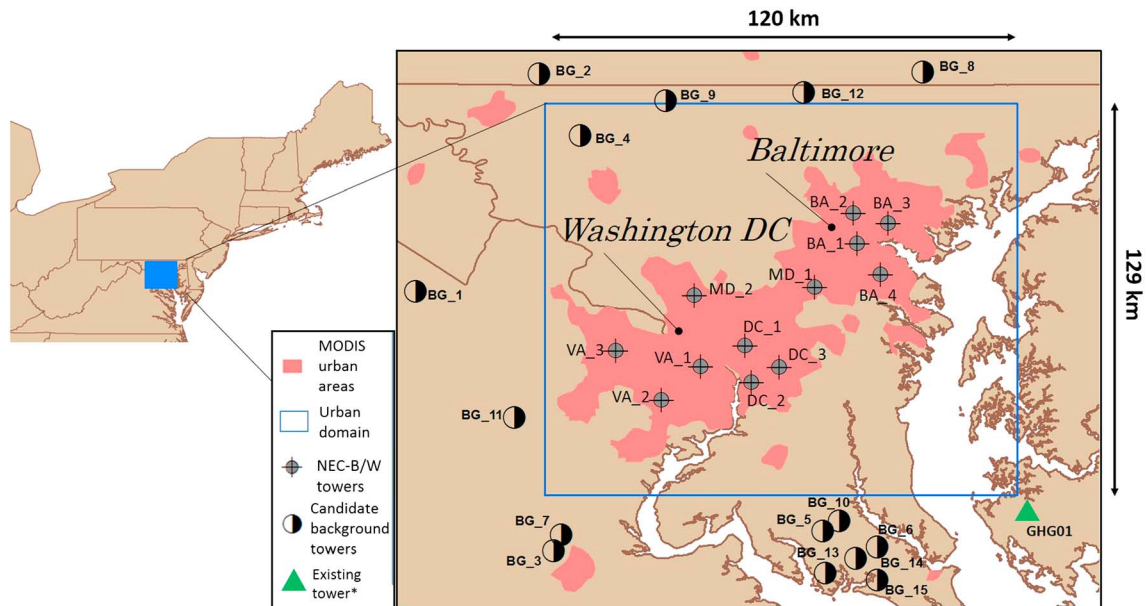
Figure 1. Site map for the Northeast Corridor (NEC-B/W) test bed. The blue box (NEC-B/W domain) is the area where GHG emissions fluxes will be estimated at a 1–2 km 2 resolution using atmospheric in-domain CO 2 observations from 12 urban tower locations shown (gray circles). Candidate background tower locations (black and white circles) are based on FCC towers filtered on specific conditions including height (~100 m) and proximity to major emission sources. GHG01 (green triangle) is an existing in situ tower location. At the time of this analysis, it was unclear whether this tower location would be available as a candidate tower location, and thus, it was not considered in the analysis (refer to section 5). The red areas are urban extent as defined by MODIS 2012 ( https://lpdaac.usgs.gov/dataset_discovery/modis/modis_products_table/mcd12q1 ). A list of both the NEC-B/W towers and potential background tower locations with their latitudes, longitudes, and height above ground level (AGL) is provided in Table S1.
