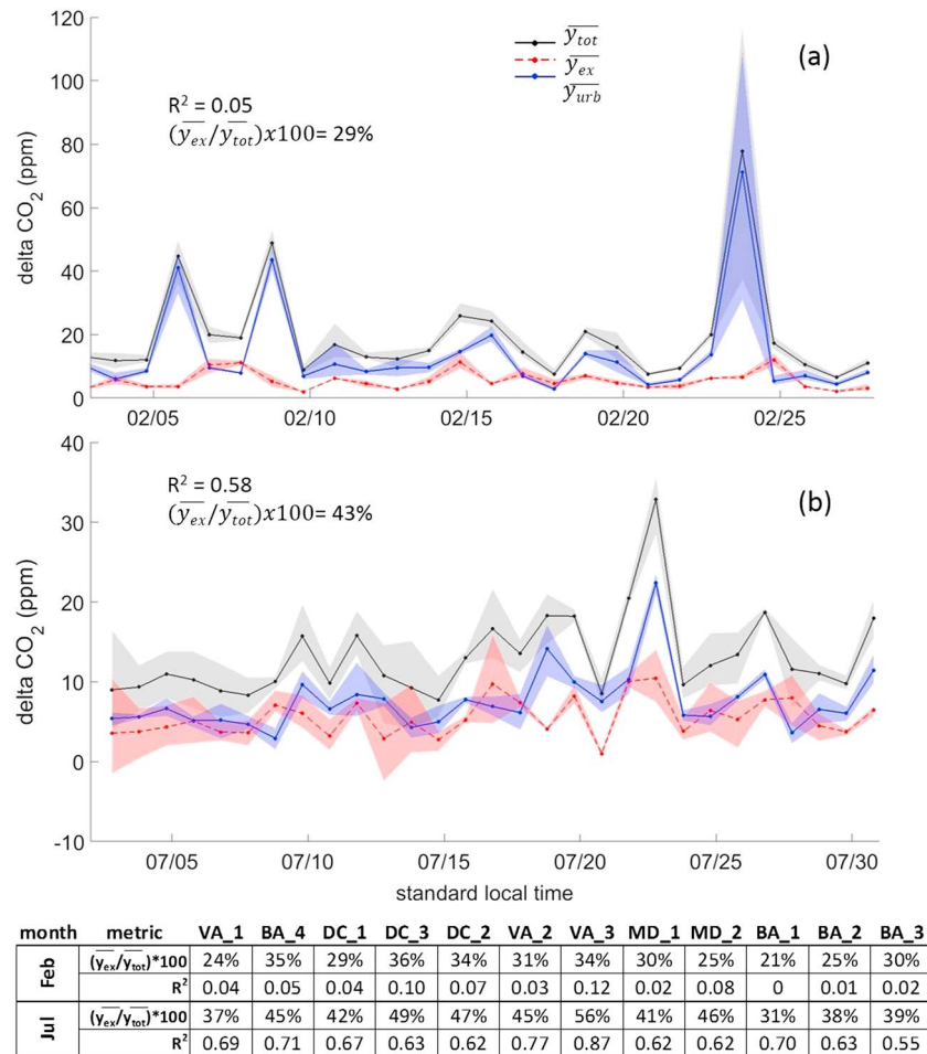
Figure 3. Total modeled CO 2 mole fraction enhancements ( y_{tot} , ppm) (black line and points) of the daily mean of afternoon observations (12 p.m. to 5 p.m. local time) averaged across all the NEC-B/W towers for the months of (a) February and (b) July for 2013. Plots also include modeled CO 2 mole fraction (ppm) from sources and sinks inside the NEC-B/W domain ( y_{urb} , solid blue line and points) and those from extrurban fluxes ( y_{ex} , red dashed line and points). The shading around y_{tot} , y_{ex} , and y_{urb} represent the maximum and minimum modeled enhancement for a given afternoon period. The average y_{tot} , y_{ex} , and y_{urb} are 18.8 ppm, 5.7 ppm, and 13.4 ppm for February. For July, the average y_{tot} , y_{ex} , and y_{urb} are 14.4 ppm, 5.6 ppm, and 8.7 ppm. The associated table below the figure represents the ratio of the total synthetic enhancements ( y_{tot,i} ) to those associated with incoming air observed at each NEC-B/W tower location ( y_{ex,i} ) for each month along with R^2 values. Real observations for February 2017 from the established NEC-B/W towers are consistent with the synthetic observations shown above both in terms of overall magnitudes and the variability of the time series (supporting information Figure S2). Note that the study does not include measurement error, but similar urban networks have reported 0.1 to 0.2 ppm measurement uncertainties associated with hourly mole fraction observations (Verhulst et al., 2016).
