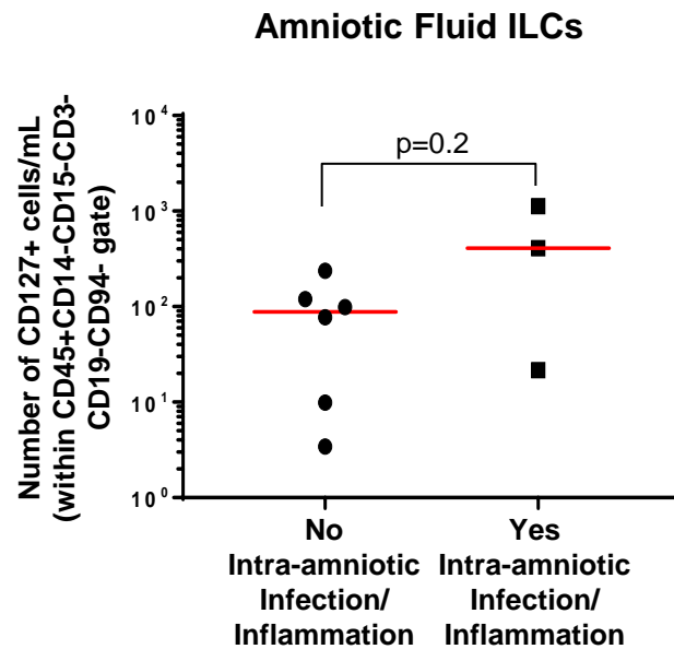
Supplementary Figure 1. Intra-amniotic infection/inflammation does not significantly increase the number of amniotic fluid ILCs in early gestation (18-22 weeks) compared to those in gestational age-matched amniotic fluids without intra-amniotic infection/inflammation. n=3-6 per group.
