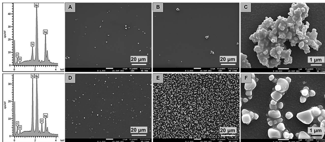
FIGURE 1. Scanning electron micrographs showing surface morphology of newly prepared silicone discs coated with (A) 5 mg L -1 Ag NPs, (B) 50 mg L -1 Ag NPs, (C) detail of a Ag NPs agglomerate adhered to the silicone disc surface, (D) discs coated with 5 mg L -1 AgNO 3 , (E) discs coated with 50 mg L -1 AgNO 3 , and (F) detail of AgNO 3 crystals adhered to the silicone disc surface. All images were acquired at ×1000 magnification, except panels (C) and (F) taken at ×15,000 magnification. The EDS spectra show the elemental composition of the nano-silver coated silicone disc surfaces.
