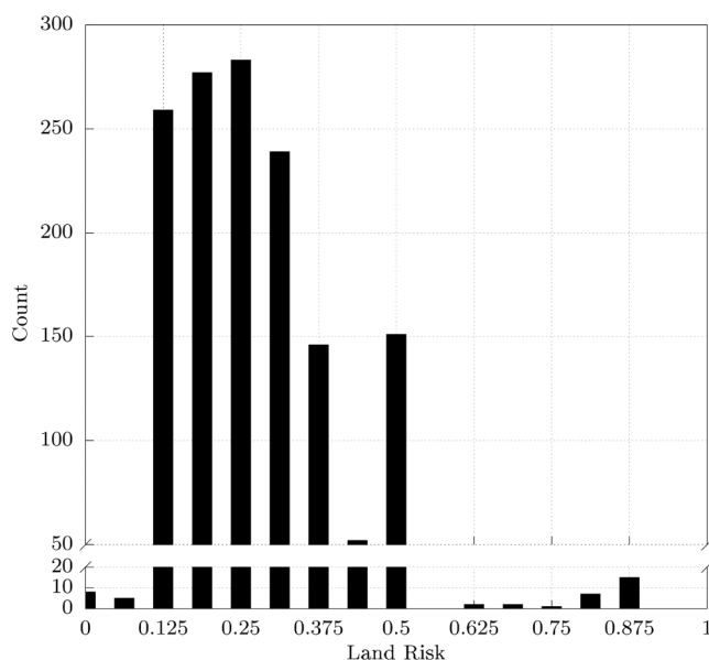
Fig. 13 Histogram of computed landing site risk on 4th December 2013, 08:30 p.m.
