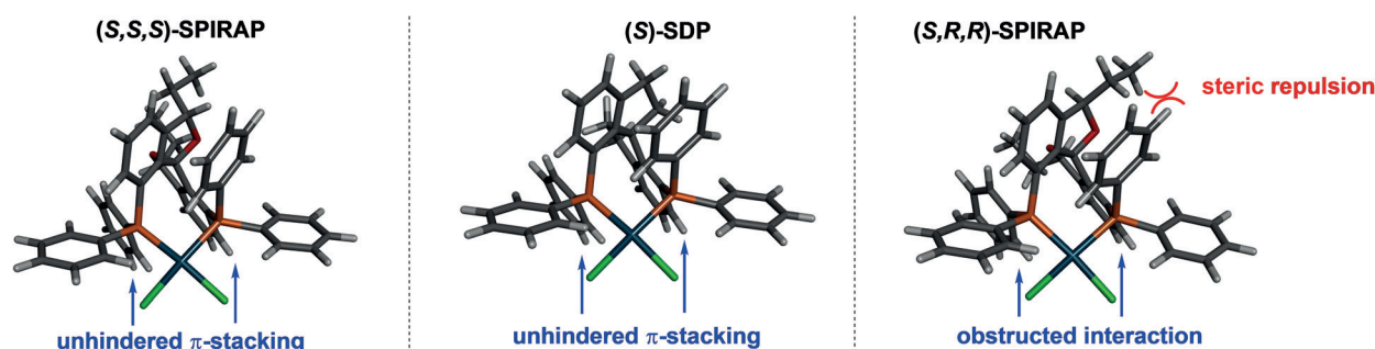
Figure 2. Comparison of ( S,R,R )-SPIRAP, ( S,S,S )-SPIRAP, and SDP complexes of PdCl 2 . The geometries of ( S,S,S )- 11 , ( R,S,S )- 11 , and ( S )- 23 were optimized by DFT with the B97-D exchange functional and mixed basis sets (LanL2dz for Pd, P, and Cl and 6-31G** for all other atoms).
