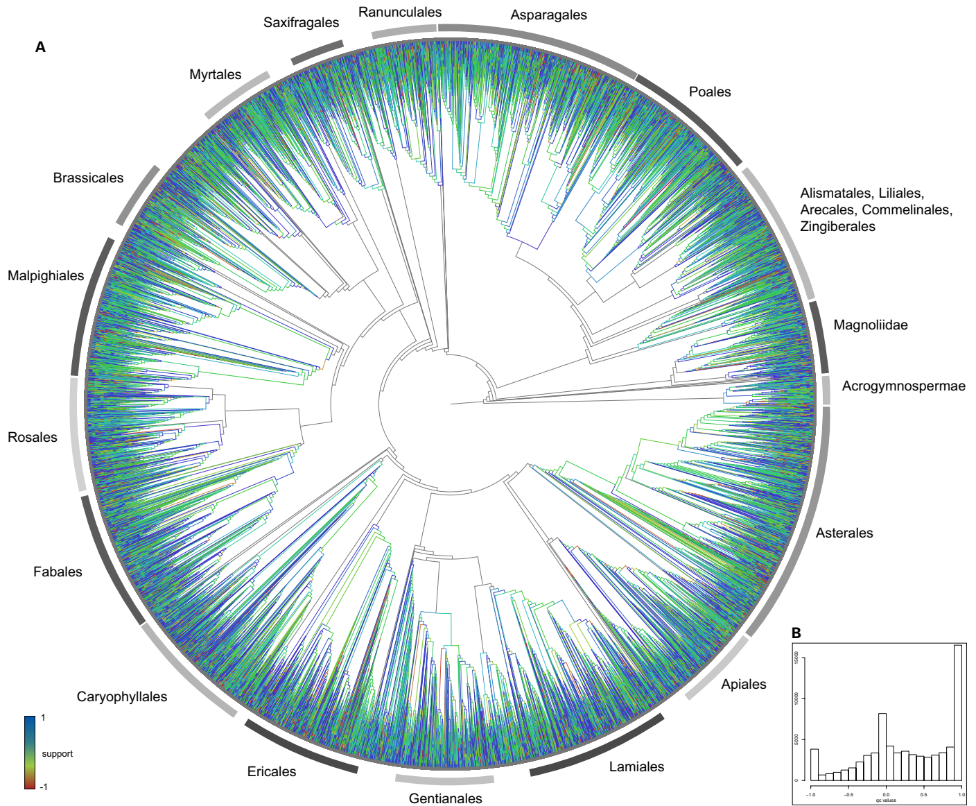
FIGURE 4. Support as measured by Quartet Concordance scores presented on the GBOTB tree (A) and (B) as a histogram summarizing across all data.
