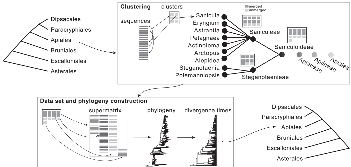
FIGURE 1. Workflow for analyses in constructing the trees. For each clade listed in Appendix S1, here Apiales, we clustered sequences starting at the most tipward clade ( Sanicula highlighted here), and merged clusters as we moved rootward Apiales. We used the clusters at the most rootward clade (Apiales in this example) to construct a supermatrix where we chose clusters that had good representation for the rootward clade or good representation for a subtending clade (as shown by the gene region on the far right). Using this supermatrix, we constructed a phylogeny and estimated divergence times. We then placed this constructed phylogeny into the backbone (either Open Tree of Life or Magallón et al. [2015]) as-is or with the unsampled taxa from the OT-taxonomy placed back.
