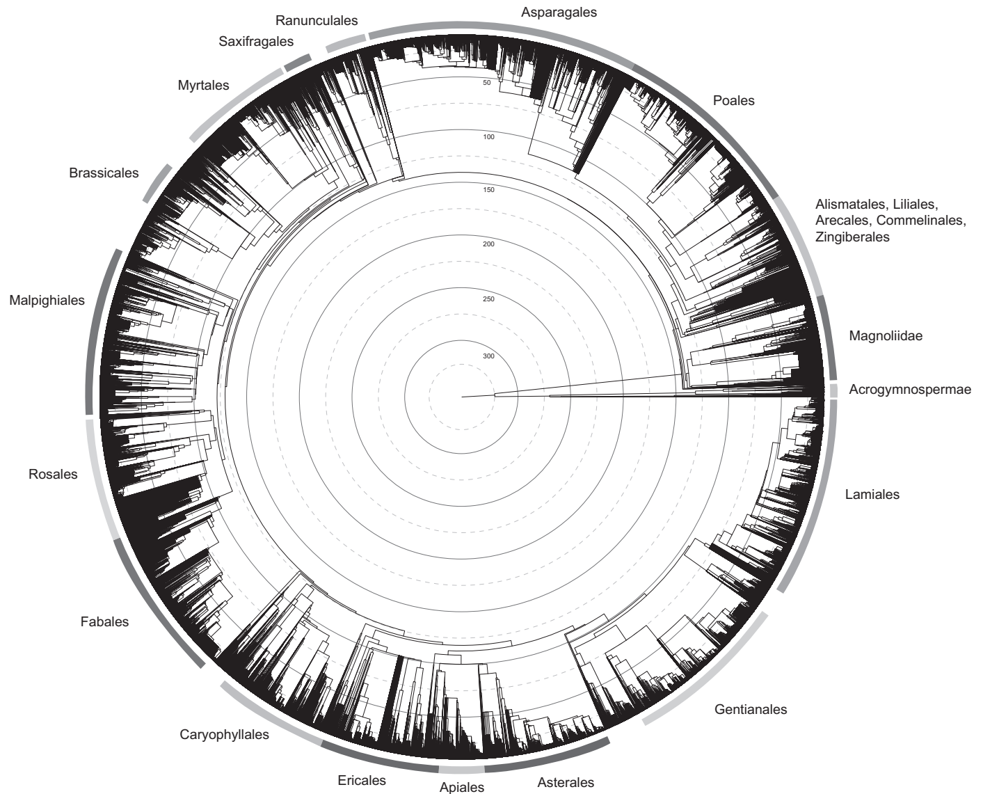
FIGURE 5. The ALLOTB tree with some major clades labeled and 353,185 tips. Divergence times are denoted with concentric circles.
