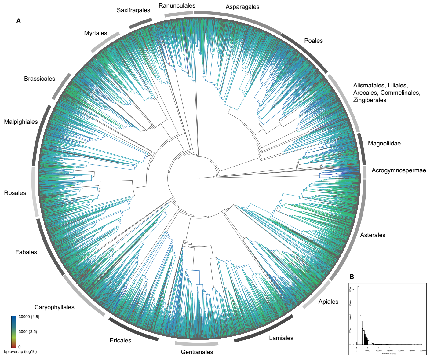
FIGURE 3. Data overlap presented on the GBOTB tree (A) and (B) as a histogram summarizing across all data. Values on the tree are displayed as \log_{10} -transformed to allow for easier visual discrimination.
