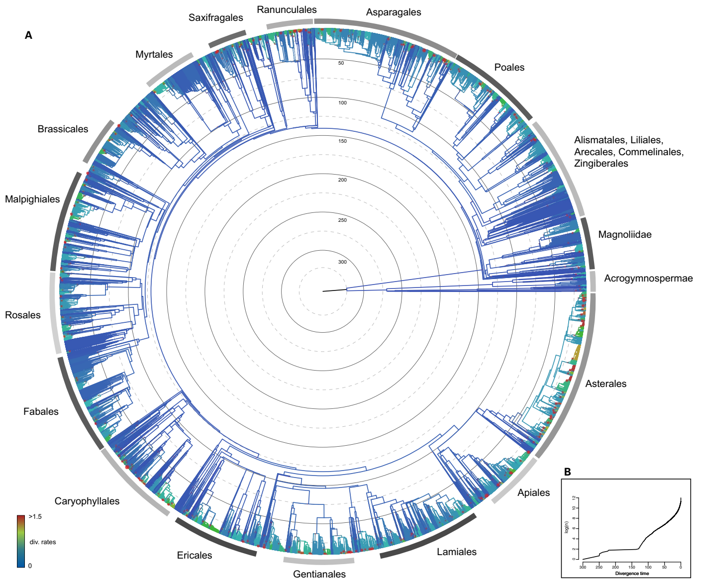
FIGURE 2. (A) GBOTB tree with colors corresponding to binned rates of diversification (see text for details on analyses). Rates were binned to make for easier visualization of rates. Red dots denote nodes with a shift in diversification rate and the size of the dot corresponds to the magnitude of the shift. (B) Lineage through time plot of the GBOTB tree. Divergence times are denoted with concentric circles.
