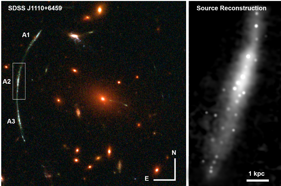
Figure 5.1 The lensed galaxy SGAS 1110. The left panel shows the HST imaging in filters F105W, F606W, and F390W, with the three images of SGAS 1110 labeled. Image A2, the most highly magnified, is highlighted with a box. The right panel shows our reconstruction of this lensed galaxy in the source plane. Two dozen clumps of star formation are obvious in the reconstructed image; all have sizes much smaller than the kiloparsec scales typically probed by unlensed surveys of distant galaxies, and several times smaller than previously probed by gravitational lensing.
