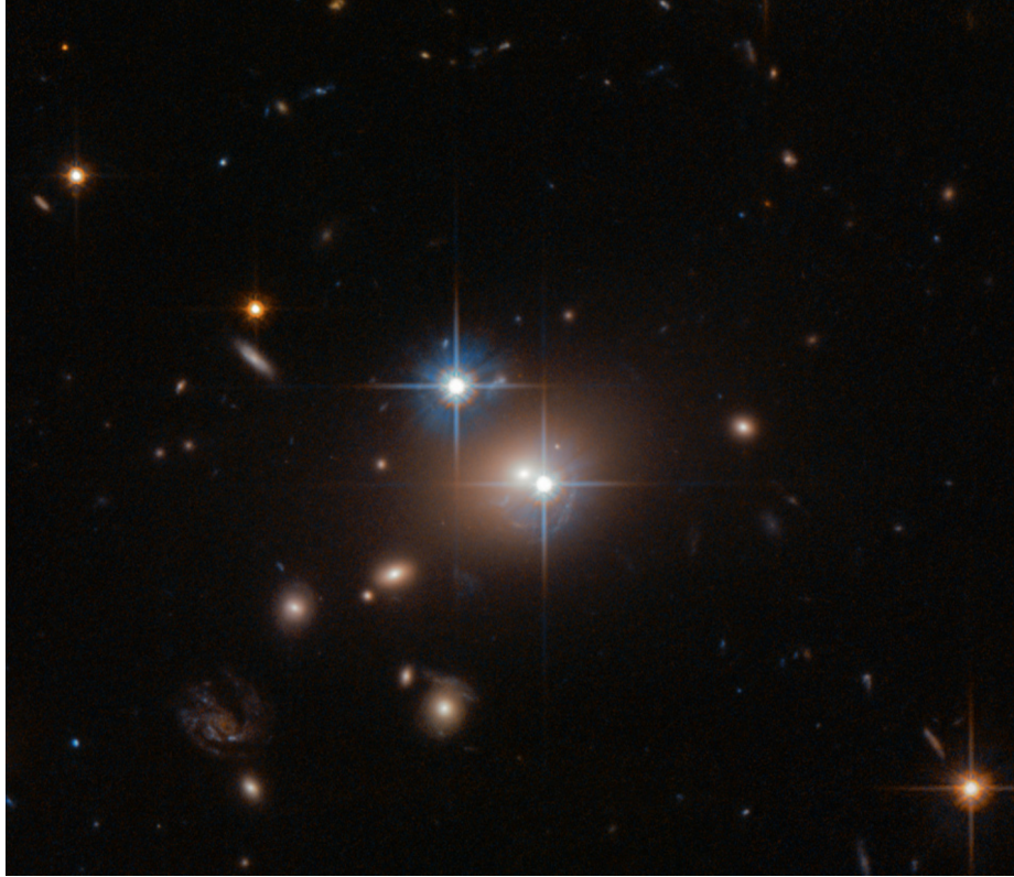
Figure 1.2 Hubble Space Telescope (HST) image of the famous Twin Quasar. From “Seeing double”. ESA/Hubble Picture of the Week. Retrieved 30 November 2017. The two bright blue objects with diffraction spikes close to the central galaxy are the two images of the quasar. The other redder objects with diffraction spikes are foreground stars.
