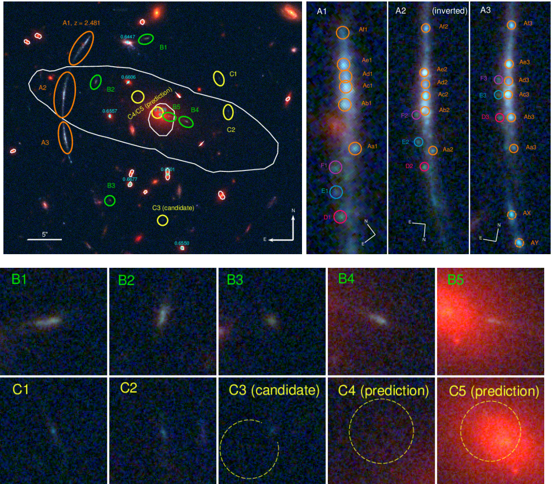
Figure 4.3 (Top left) HST WFC3 imaging of SDSS J1110+6459 in F160W (red), F606W (green), and F390W (blue). Labeled are image systems A, B, and C used in the lens modeling. The redshifts of other objects from Table 4.1 are shown in cyan. The critical curve for z = 2.481 is shown by the white lines. (Top right) Close up image of the three images of the main arc A and systems D, E, and F; the middle image has been inverted along the N-S direction to match parity with the other two images. The clumps labeled A[a-f] are individual clumps matched across all three images used as constraints in the model. AX and AY are likely part of the lensed galaxy, but lie outside the caustic region and thus are not multiply imaged. Each circle is 0.1'' in radius. (Bottom) Images of systems B and C. The dashed circle indicates the center and rms scatter of the predicted images marginalized over all models which predict that image. Each postage stamp cutout is 3'' \times 3'' .
