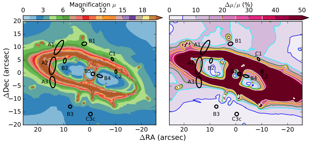
Figure 4.8 The weighted median magnification map for a source at z = 2.481 stacked from all eight different lens models (left) and the corresponding uncertainty in magnification marginalized across all eight models (right). The locations of the multiple images are shown by the black ovals.
