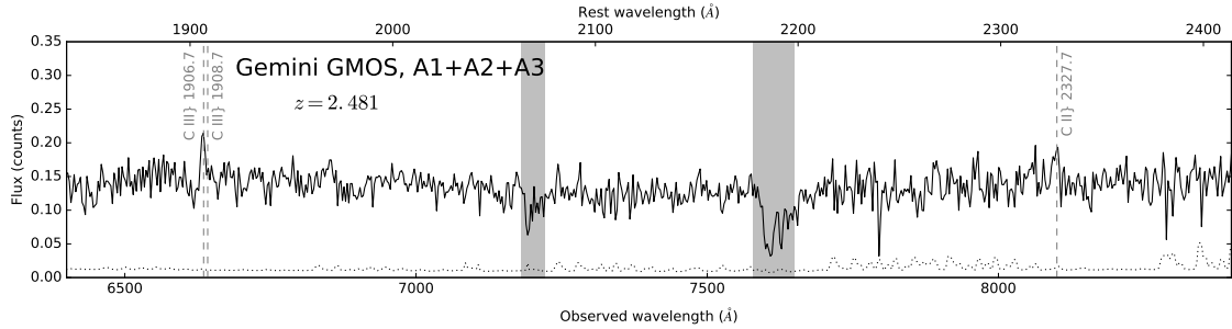
Figure 4.2 Gemini GMOS spectrum of SGAS 1110, summed from slits placed on all three images (A1, A2, and A3). The dotted line indicates the noise level, and the gray bands indicates part of the spectrum with strong telluric absorption. The vertical gray-dashed lines indicate the locations of rest-frame UV emission lines.
