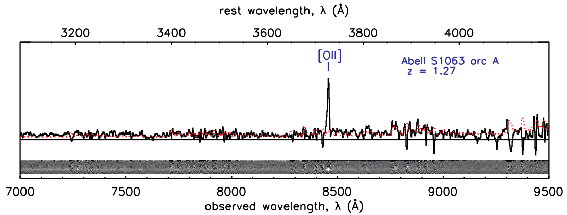
Figure A.6 One-dimensional and two-dimensional spectra of Abell S1063 arc A. The noise level of the one-dimensional spectrum is plotted in red.
