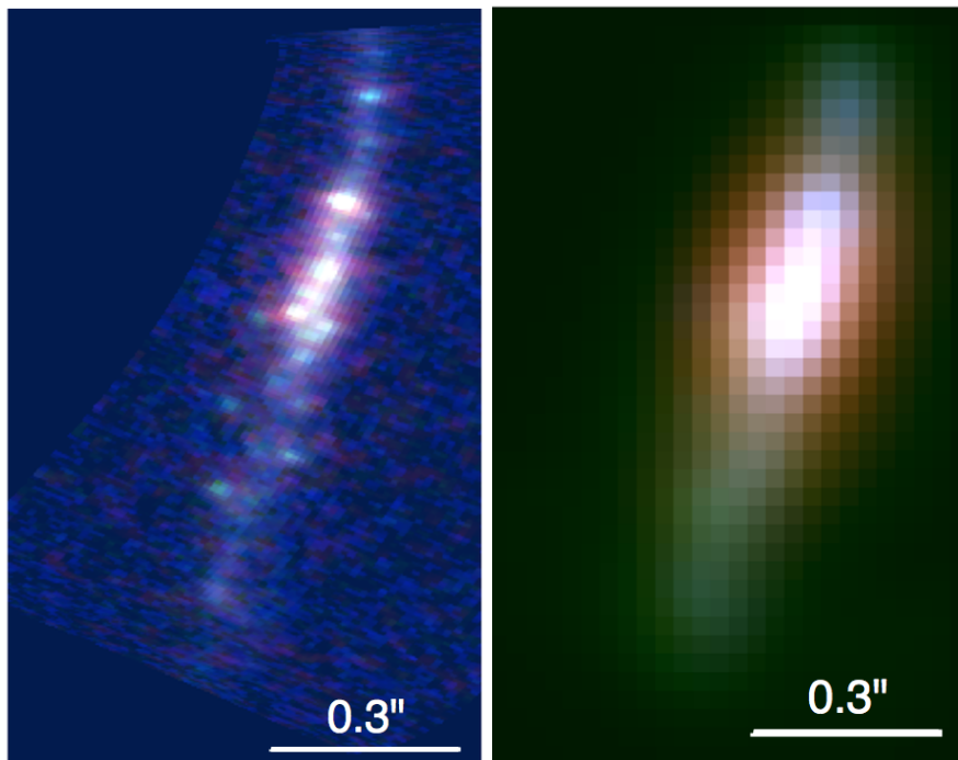
Figure 7.1 From Rigby et al. (2017a): (Left) The source plane reconstruction of SGAS 1110, pixel scale of 3 mas. Roughly 24% of the star formation of this galaxy is in clumps. (Right) SGAS 1110 source reconstruction convolved with the HST PSF and rebinned to a pixel scale of 30 mas. This is what this galaxy would look like had it been detected in a deep field. All the star formation would be observed to occur in an exponential disk, with no evidence of clump morphology.
