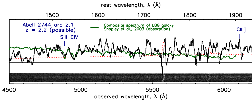
Figure A.7 One-dimensional and two-dimensional spectra of Abell 2744 arc 2. The noise level of the one-dimensional spectrum is plotted in red. We over plot a composite spectrum of high-redshift ( z = 3 ) Lyman break galaxies with strong absorption features from Shapley et al. (2003) to show similarities in spectral features as well as the Lyman break in the continuum. We find a possible solution for the redshift z \sim 2.2 for this galaxy.
