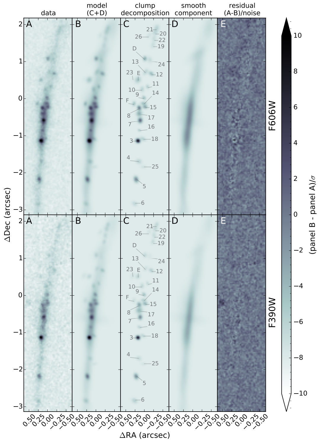
Figure 4.9 GALFIT clump decomposition in F606W (top) and F390W (bottom) imaging. (A) HST imaging of the middle image of SGAS 1110 in the image plane. (B) The complete GALFIT model of the middle image of the arc. (C) Clump component of panel B. (D) Smooth component of panel B. (E) Residual of the clump+smooth GALFIT model and the data in units of rms noise.
