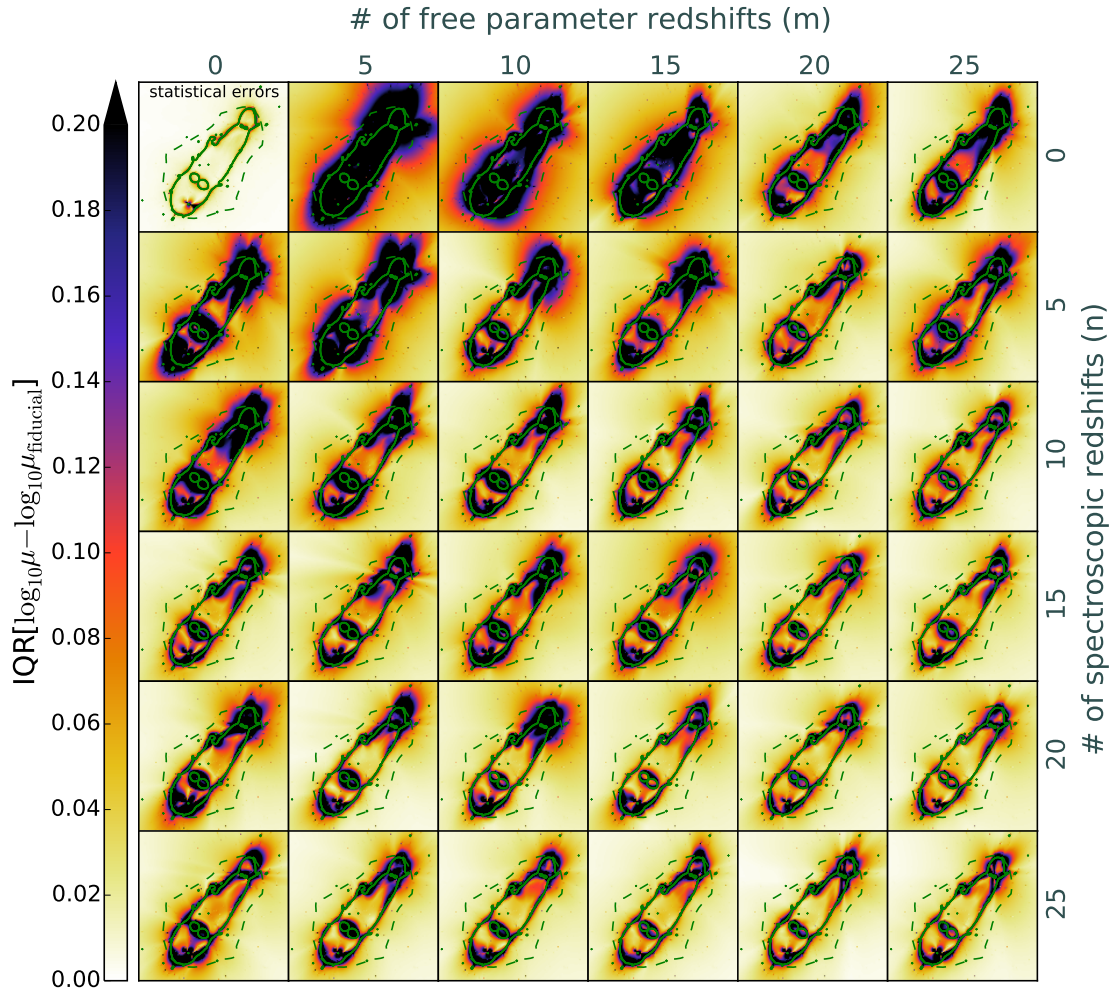
Figure 3.7 Interquartile range (IQR) of errors in the magnification maps for z = 2 for each set of models with various numbers of constraints with spectroscopic redshifts and free parameter redshifts. The error is computed with respect to the magnification map of the fiducial model. The z = 2 critical curve for the fiducial model is shown in the solid green and the region enclosed by the dashed green line is the extent of image multiplicity for sources at z = 2 . The top-left panel shows the statistical error range in magnification for each pixel of the fiducial model. Each panel has dimensions 200'' \times 200'' .
