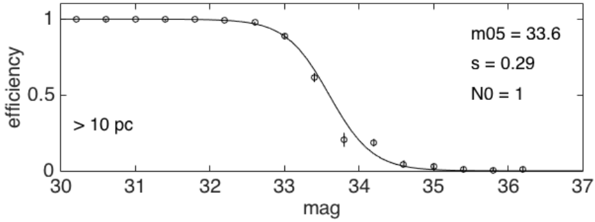
Figure 4.12 Model fits to the empirical efficiency for clumps larger than 10 pc, as a function of clump magnitude. The best-fit parameters to (4.8) for each size bin are shown in the upper right-hand corner.
