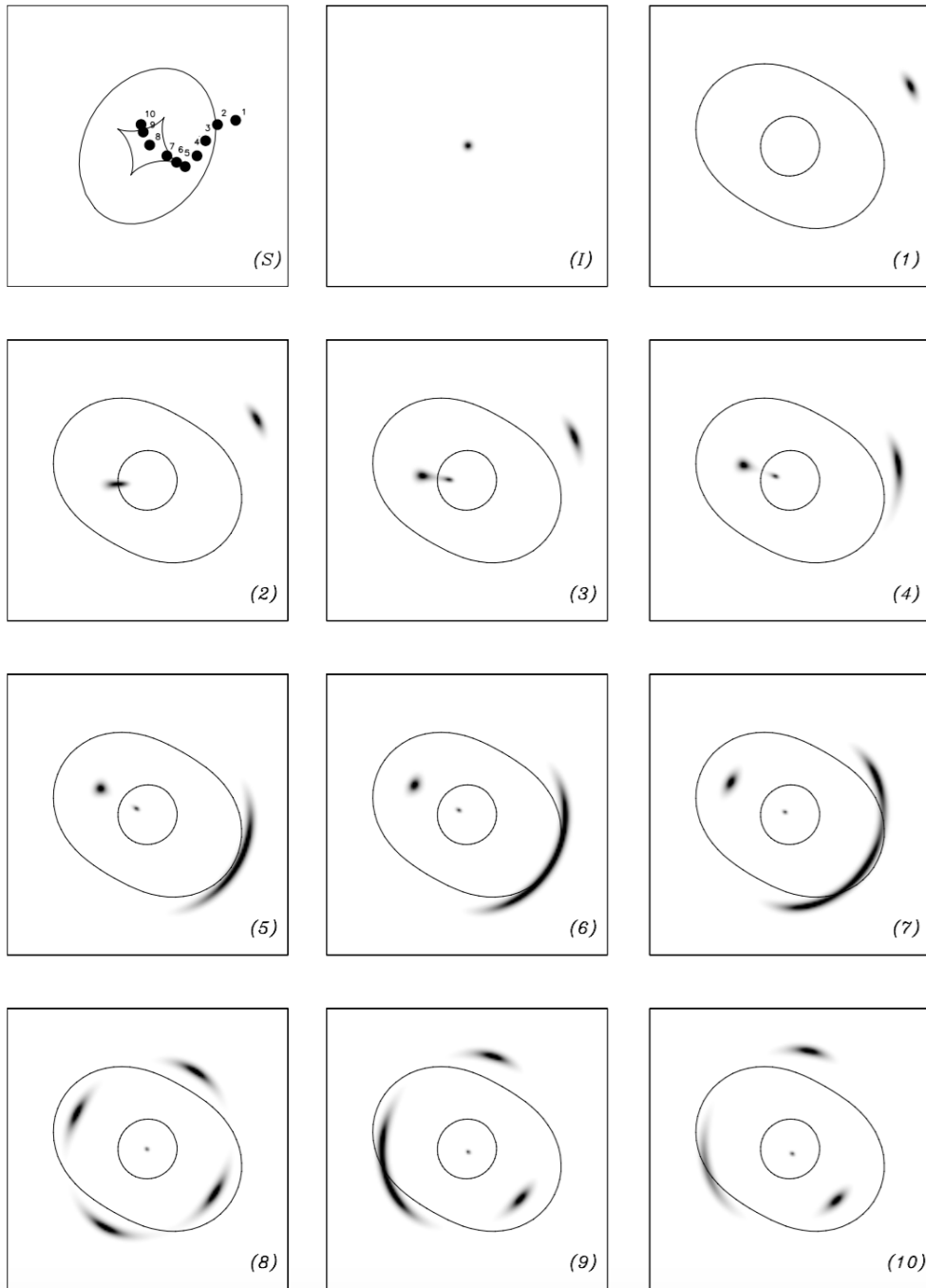
Figure 1.5 From Kneib & Natarajan (2011), original caption: “Multiple-image configurations produced by a simple elliptical mass distribution. The panel (S) shows the caustic lines in the source plane and the positions numbered 1 to 10 denote the source position relative to the caustic lines. The panel (I) shows the image of the source without lensing. The panels (1) to (10) show the resulting lensed images for the various source positions. Certain configurations are very typical and are named as follows: (3) radial arc, (6) cusp arc, (8) Einstein cross, (10) fold arc.”
