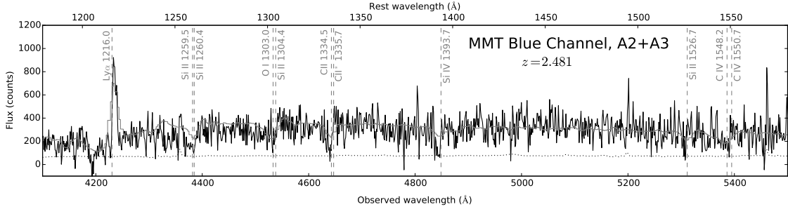
Figure 4.4 MMT Blue Channel Spectrograph spectrum of SGAS 1110. The dotted line indicates the noise level, and the gray-solid line is a spectral template of Ly \alpha -emitting galaxies with strong absorption features at z \sim 3 galaxies from Shapley et al. (2003). The vertical gray-dashed lines indicate the locations of rest-frame UV emission and absorption lines.
