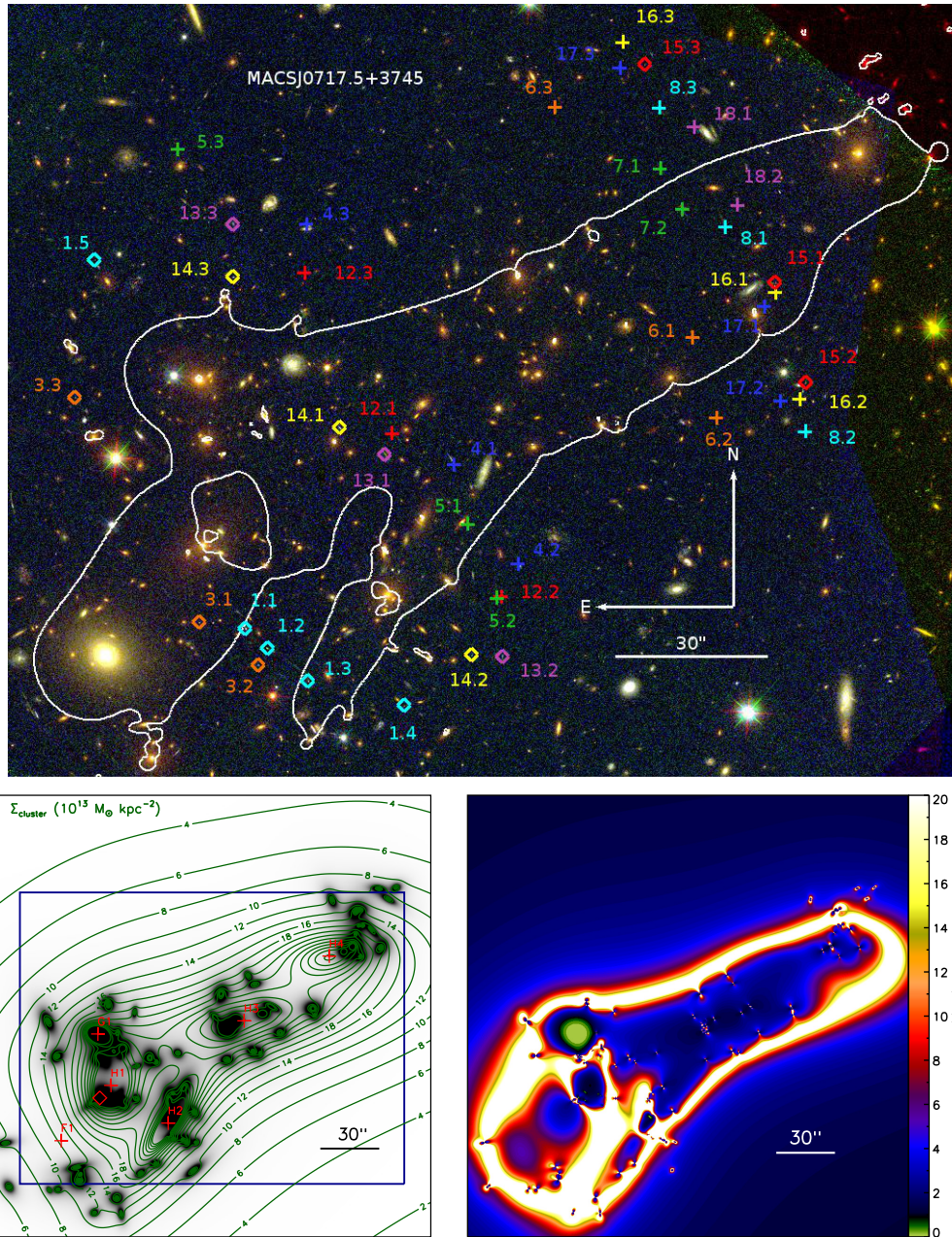
Figure 2.3 Top: False color image of MACS J0717.5+3745 from ACS imaging (red, F814W; green, F606W; blue, F435W). Labels are the same as in Figure 2.1. Left: Contour map of the total surface mass distribution (in units of 10^{13} M_{\odot} \text{ kpc}^{-2} ) of the cluster overlaid on the mass contained in cluster member galaxies. The spacing of the contours is linear. The locations and labels of each optimized halo (see Table C.3) are shown in red crosses. The red diamond indicates the location of the reference point. The blue box indicates the field of view of the top image. Right: Absolute value of magnification in the image plane for a source at z = 9 .
