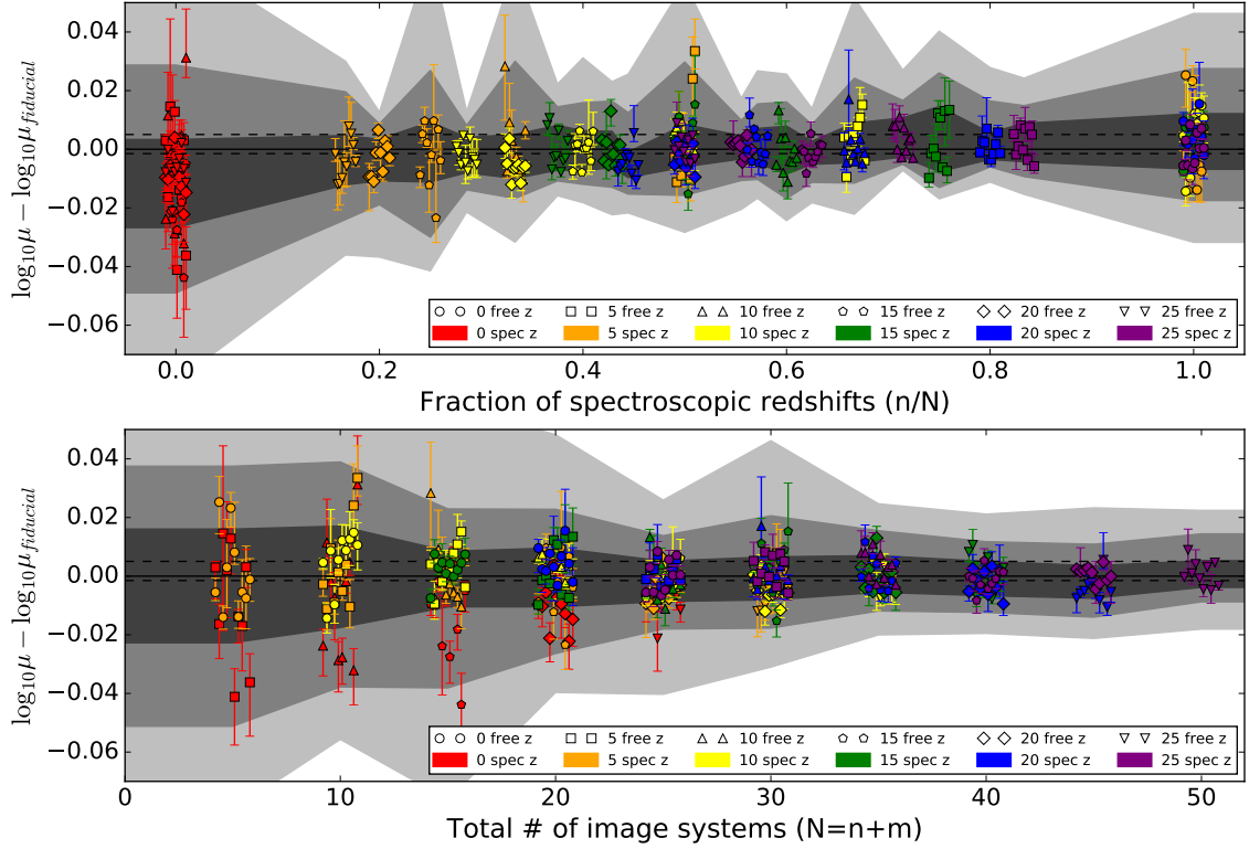
Figure 3.9 The relative magnification error ( z = 2 ) for the region of pixels shown in Figure 3.2 for all the test models versus fraction of spectroscopic redshifts n/N (top) and total number of image systems N (bottom). The values are median and 1\sigma range of values within the region for the best fit models. The different shapes and colors indicate the number of free parameter redshifts and spectroscopic redshifts used in the model, respectively. The dashed lines indicated the 1\sigma statistical errors for the fiducial model. The gray contours represent the 1, 2, and 3\sigma ranges for each block of the test models in fraction/number of systems. Note: the abscissa values for the test models within each grouping of test models have been slightly offset horizontally for display purposes. There is a clear trend of improved magnification error with the total number of images, but no dependence on the fraction of spectroscopic redshifts.
