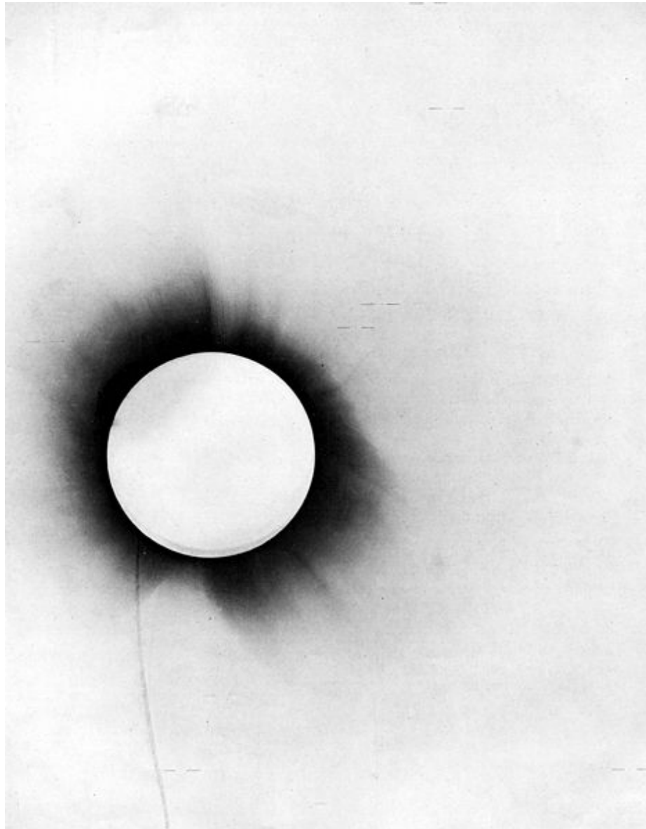
Figure 1.1 From Dyson et al. (1920), original caption: “From the report of Sir Arthur Eddington on the expedition to verify Albert Einstein’s prediction of the bending of light around the sun. In Plate 1 is given a half-tone reproduction of one of the negatives taken with the 4-inch lens at Sobral. This shows the position of the stars, and, as far as possible in a reproduction of this kind, the character of the images, as there has been no retouching. A number of photographic prints have been made and applications for these from astronomers, who wish to assure themselves of the quality of the photographs, will be considered as far as possible acceded to.”
