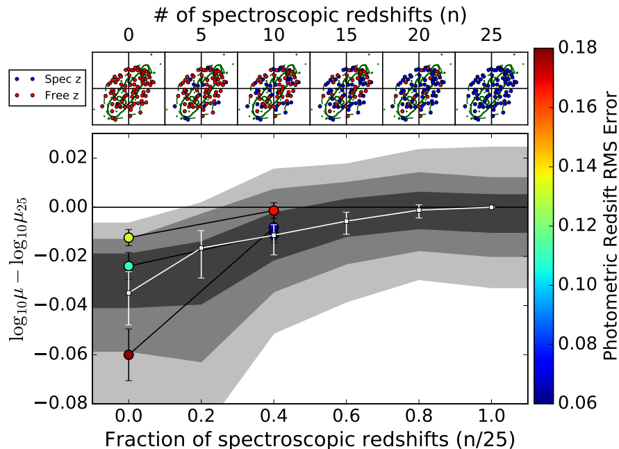
Figure 3.10 The relative magnification error in ( z = 2 ) for the region of pixels shown in Figure 3.2 versus fraction of spectroscopic redshift systems for six lens models built using the same 25 image systems. The first model uses no spectroscopic redshifts, the second model adds spectroscopic redshifts to 5 systems, the third model adds spectroscopic redshifts to 5 more systems (10 total), etc. until all systems have spectroscopic redshifts. The errors are with respect to the model with all 25 spectroscopic redshift systems. The values are the median and 1\sigma range of values with the region of the best fit model. The gray contours represent the 1,2, and 3\sigma statistical errors estimated from the MCMCs. The top row shows the image plane positions of the images from the 25 systems used as constraints. The blue and red points represent systems with and without spectroscopic redshifts, respectively. Each map is 200'' \times 200'' centered on the origin defined in Figure 3.2. The green solid and dashed lines indicate the locations of the z = 2 critical curve and region of multiple images, respectively. The colored circles represent models using the same constraints as the models shown in the maps above; however, photometric redshift measurements are used as the priors for the free parameter redshifts rather than a uniform random prior. The colors indicate the rms error in the photometric redshifts used for that particular model: (z_{\text{spec}} - z_{\text{phot}})/(1 + z_{\text{spec}}) (see § 3.9.2).
