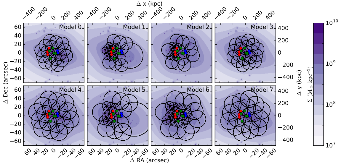
Figure 4.6 Surface mass density of each lens model. The circles show where each node of the multi scale grid is centered, with radius equal to the cut radius of that node. Overlaid on grid for reference are the locations for arcs A (red), B (green), and C (blue). All offsets are given with respect to the center of the BCG.
