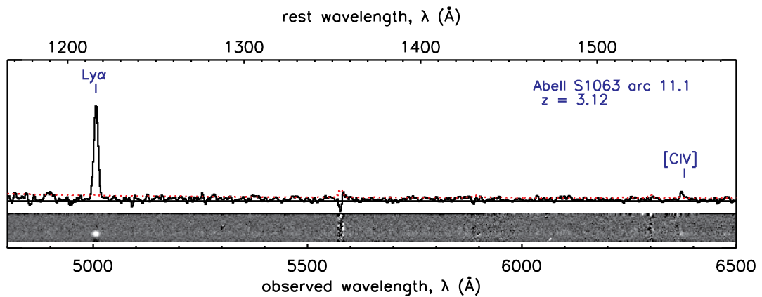
Figure A.5 One-dimensional and two-dimensional spectra of Abell S1063 arc 11.1. The noise level of the one-dimensional spectrum is plotted in red.
