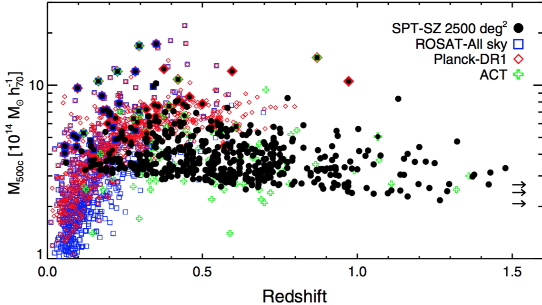
Figure 1.8 From Bleem et al. (2015): The masses and redshifts of optically-confirmed clusters discovered in the SPT, ACT, Planck and ROSAT surveys.
