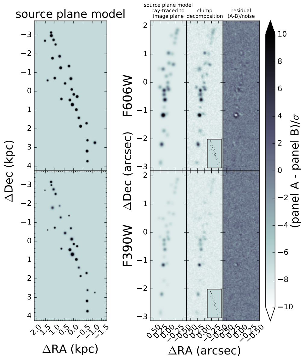
Figure 4.10 Left panel: model of clumps in the source plane. Note: the middle image of the galaxy has negative parity in declination; for display purposes the y-axis has been flipped to match the orientation of galaxy in the image plane. Panel A: the source plane model from the left panel, ray-traced to the image plane and convolved with the HST PSF. Panel B: the clump decomposition model (also Panel B from Figure 4.9 with added noise). The inset shows the source plane model (left panel), scaled to its true angular size with respect to its magnified image. Panel C: residual of source plane model and clump decomposition, in units of rms noise.
