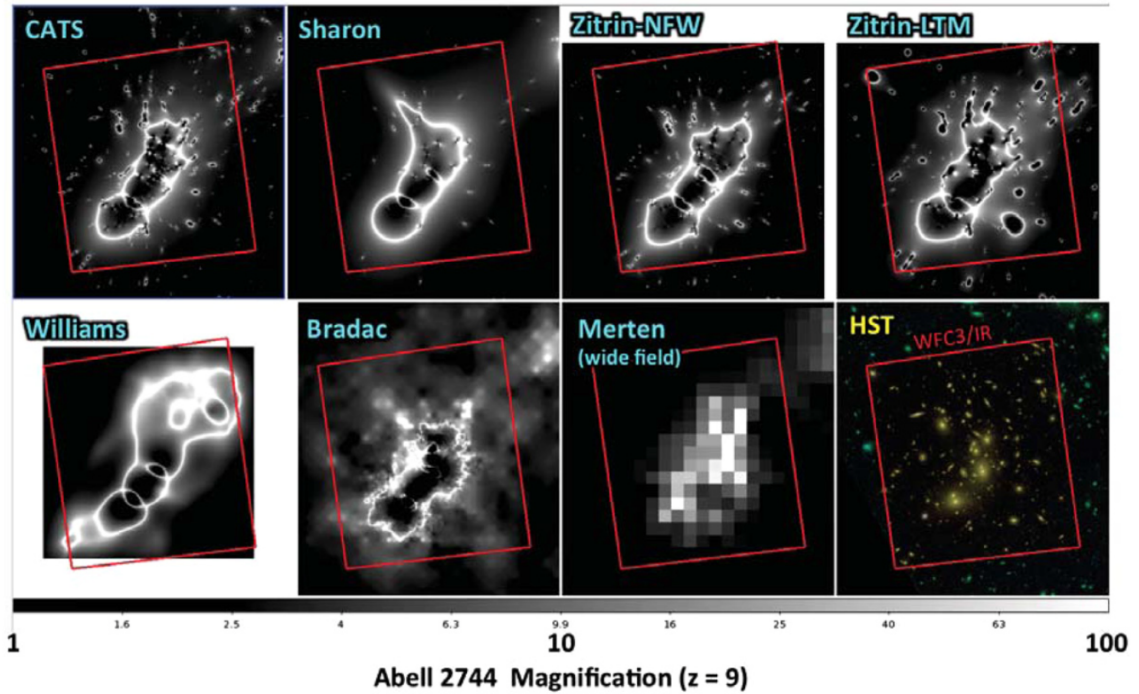
Figure 1.10 From Coe et al. (2015), original caption: “Magnification maps (log grayscale) for z = 9 galaxies lensed by A2744 according to all seven submitted gravitational lensing models. The Frontier Fields WFC3/IR FOV ( 136'' \times 123'' ) is outlined in red. At bottom right is a color HST image (produced with Trilogy; Coe et al., 2012) showing the Frontier Fields WFC3/IR observations (red channel) within the prior ACS observations (blue-green). North is up and East is to the left.”
