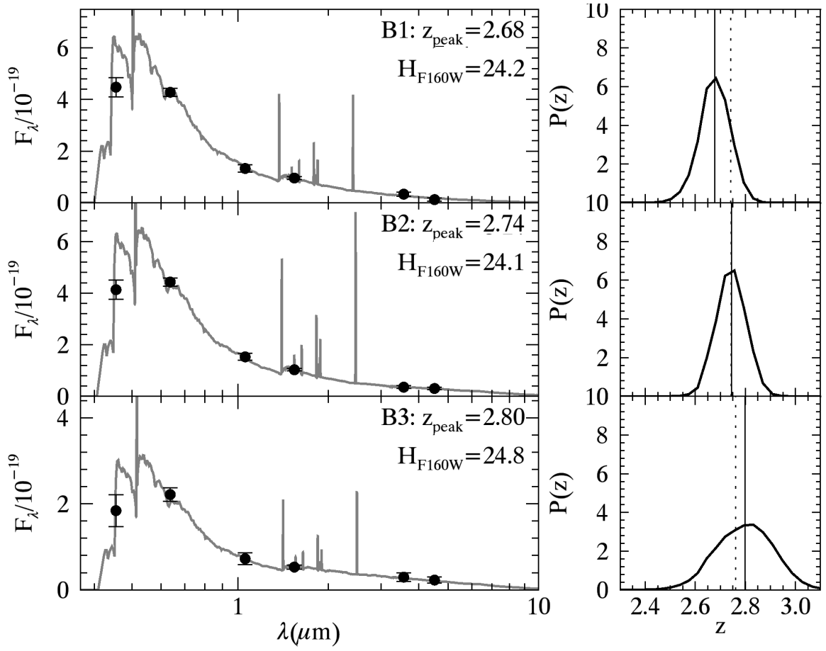
Figure 4.5 Spectral energy distribution and photometric redshift for arcs B1, B2, and B3. z_{\text{peak}} is the highest-probability z weighted by P(z) : z_{\text{peak}} = \int zp(z)dz / \int P(z)dz . F_{\lambda} is in units of \text{erg s}^{-1} \text{cm}^{-2} \text{\AA}^{-1} .
