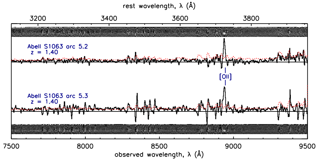
Figure A.3 One-dimensional and two-dimensional spectra of Abell S1063 arcs 5.2 and 5.3. The noise level of the one-dimensional spectrum is plotted in red.
