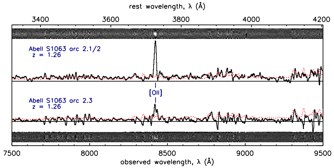
Figure A.2 One-dimensional and two-dimensional spectra of Abell S1063 arcs 2.1/2 (merging pair) and 2.3. The noise level of the one-dimensional spectrum is plotted in red.
