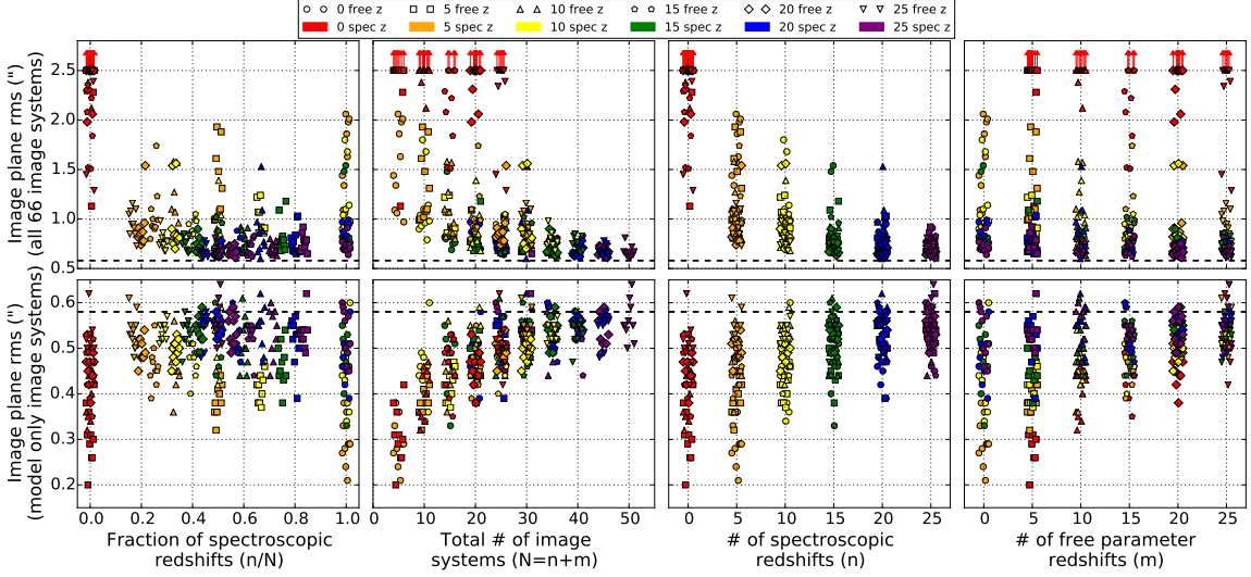
Figure 3.3 Image plane rms for all the test models plotted versus fraction of spectroscopic redshifts, total number of image systems, number of spectroscopic redshifts, and number of free parameter redshifts. The colors and shapes of the points represent the number of spectroscopic redshifts and number of free parameter redshifts used in the model, respectively (see legend at top). The top panels show the image plane rms values computed for all 66 image systems using the true redshift values. The bottom panels show the image plane rms values computed only from the images used as constraints in the lens model and model predicted redshifts. The dashed line indicates the value of the image plane rms for the fiducial model and is computed from all 66 image systems and true redshifts.
