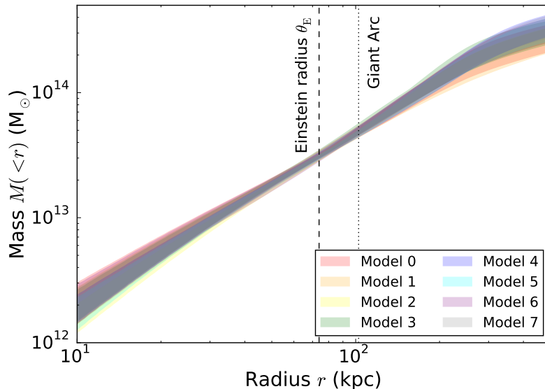
Figure 4.7 We plot the integrated mass profile within radius r of the galaxy cluster SDSS J1110+6459 for each of the eight lens models. The shaded region indicates the 1\sigma uncertainty range in the mass. The dashed lines indicate the locations of the effective Einstein radius at z = 2.481 and the radius of the giant arc. All models are in good agreement and converge at the Einstein radius, which corresponds roughly to the typical projected radius of the multiple images used as constraints in the lens models.
