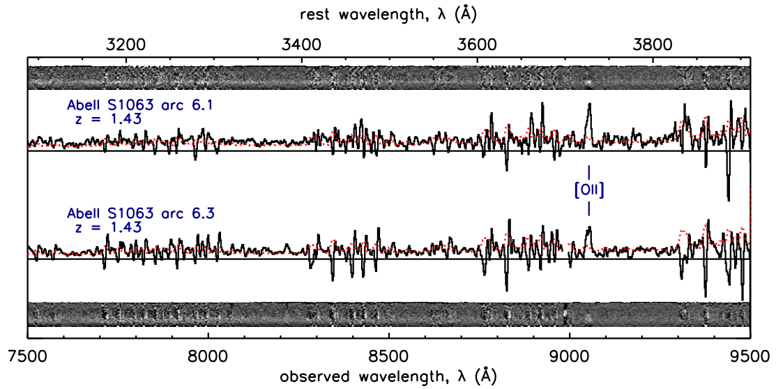
Figure A.4 One-dimensional and two-dimensional spectra of Abell S1063 arcs 6.1 and 6.3. The noise level of the one-dimensional spectrum is plotted in red.
