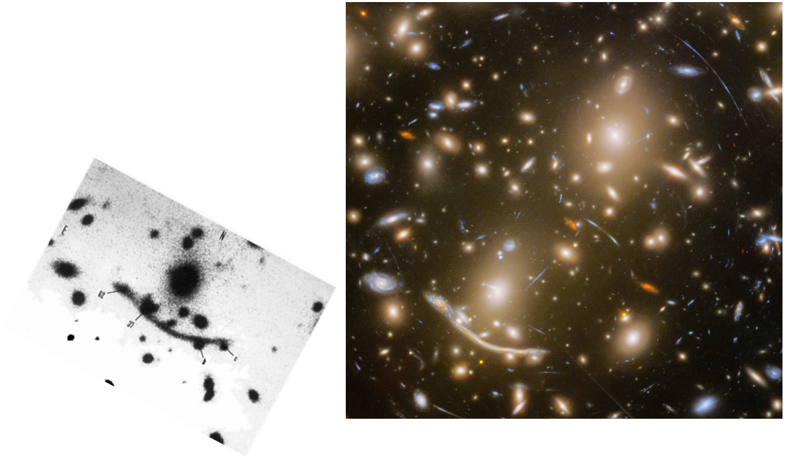
Figure 1.3 Left: From Soucail et al. (1988), original caption: “CCD frame of the giant arc in A370. This picture was obtained by J.L. Prieur at the prime focus of the 3.60m Canada-France-Hawaii telescope on October 25th, 1987. The CCD was a 640 \times 1024 RCA2: scale 0.2''/\text{pixel} – seeing 0.7'' , with an exposure time of 10 minutes in white light. Note the shape of the object #37, which was already suspected based on its spectrum Soucail et al. (1987b)”, meaning that since the object is not at the cluster redshift, but indeed behind it and being lensed into a fantastic arc. Right: 140-orbit HST image of Abell 370 from the Hubble Frontier Fields Director’s Discretionary Program. From “The last of the Frontier Fields – Abell 370. STScI. Retrieved 30 November 2017.
