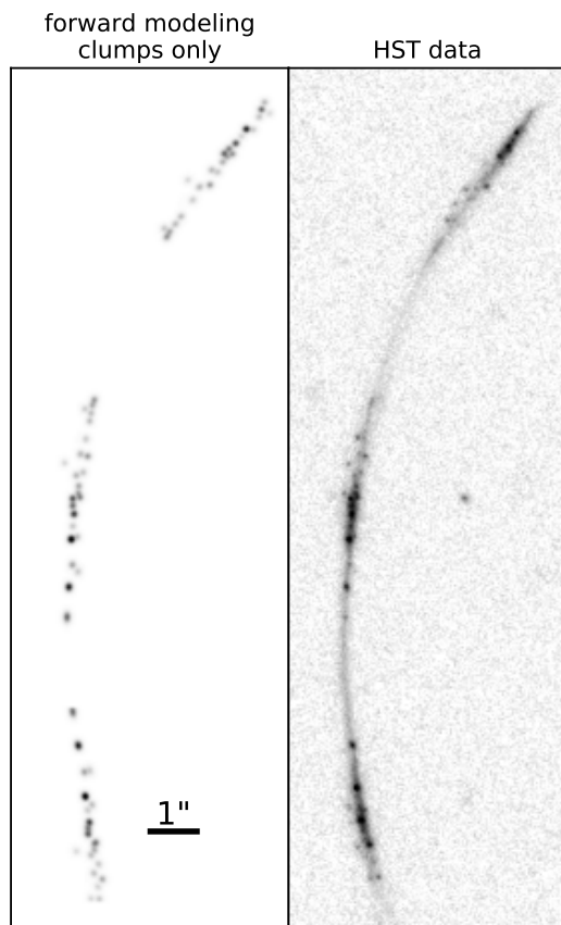
Figure 4.11 Left panel: model of clumps ray-traced to the image plane in all three images of the giant arc. Right panel: HST data of the entire giant arc. Both panels are coadded F606W and F390W. The stretch of the scaling is square root.
