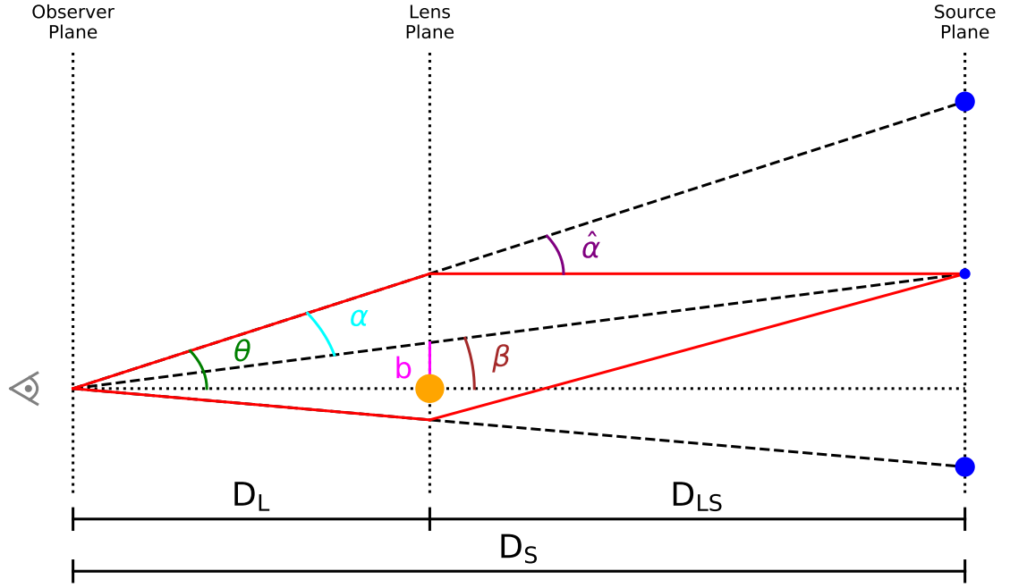
Figure 1.4 Diagram showing the definitions of angles and angular diameter distances used for deriving the lens equation.
