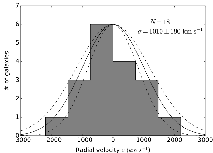
Figure 4.1 Histogram of the radial velocities of the spectroscopically confirmed cluster member galaxies in SDSS J1110+6459 with respect to the bi-weight center at z = 0.656 . We overplot Gaussians centered on the bi-weight center with widths set to the velocity dispersion (solid line) and its 1\sigma errors (dashed lines).
