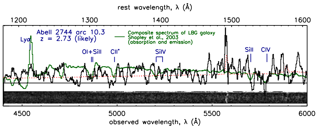
Figure A.10 One-dimensional and two-dimensional spectra of Abell 2744 arc 10.3. The noise level of the one-dimensional spectrum is plotted in red. We over plot a composite spectrum of high-redshift ( z = 3 ) Lyman break galaxies with both strong absorption and emission features from Shapley et al. (2003) to show similarities in these spectral features as well as Lyman break in the continuum. We find a possible solution for the redshift z = 2.73 for this galaxy.
