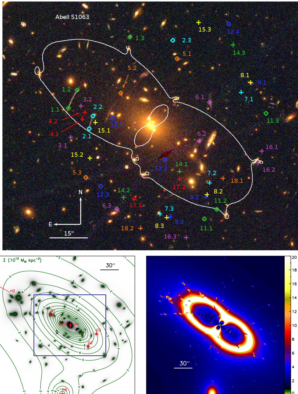
Figure 2.5 Top: False color image of Abell S1063 from ACS imaging (red, F814W; green, F606W; blue, F435W). Labels are the same as in Figure 2.1. Left: Contour map of the total surface mass distribution (in units of 10^{13} M_{\odot} \text{ kpc}^{-2} ) overlaid on the mass contained in cluster member galaxies. The spacing of the contours is linear. The locations and labels of each optimized halo (see Table C.5) are shown in red. The blue box indicates the field of view of the top image. Right: Absolute value of magnification in the image plane for a source at z = 9 .
