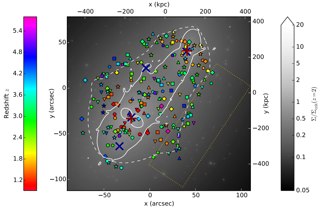
Figure 3.2 The fiducial lens model of Ares. The grayscale image shows the projected surface mass density \Sigma in units of the critical density \Sigma_{\text{crit}} = (c^2 D_S)/(4\pi G D_{\text{LS}} D_L) at z = 2 . The locations of the multiple images used in the lens model are shown by the symbols, with colors indicating redshift. Images that match to the same source have the same redshift and are represented by the same symbol. The z = 2 critical curve is shown by the solid white lines. The dashed white lines indicates the region where the model predicts multiple images for z = 2 . The red crosses and blue x's mark the centers of the two cluster halos and four galaxy halos listed in Table 3.1, respectively. The gold dotted boxed region indicates the pixels used to generate the plots in Figures 3.8, 3.9, & 3.10.
