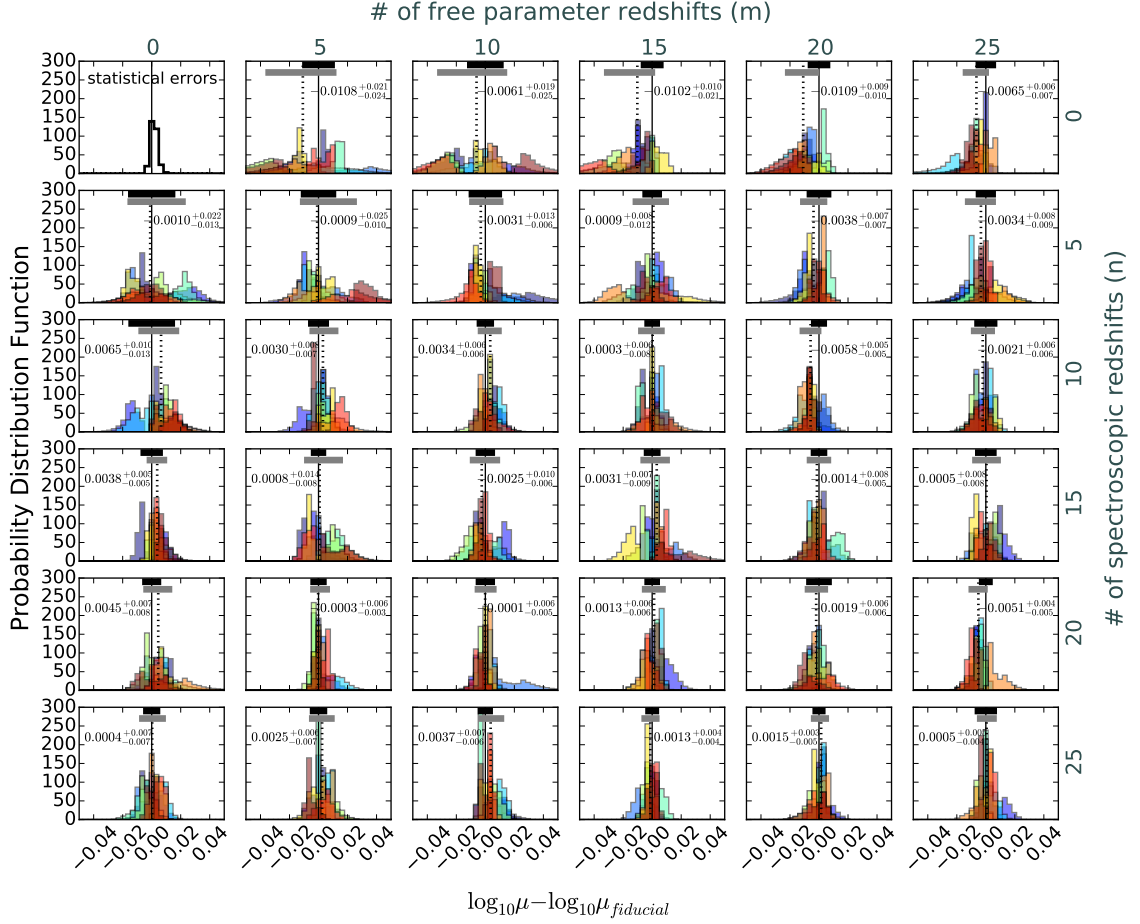
Figure 3.8 Histograms of magnification error ( z = 2 ) for the region of pixels shown in Figure 3.2 for models with different numbers of spectroscopic and free parameter redshifts. Each color shade represents a unique model constructed with different random subsets of images used as constraints. The top-left panel shows the 1\sigma statistical errors of each pixel in the fiducial model. The black bar on top shows the typical 1\sigma statistical error for a test model. The dashed vertical line and horizontal grey bars show the median and 1\sigma range in magnification error distribution of all test models combined, and these values are displayed in each panel.
