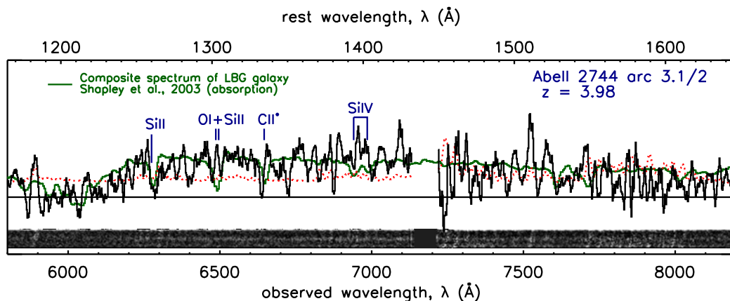
Figure A.8 One-dimensional and two-dimensional spectra of Abell 2744 arcs 3.1/2 (merging pair). The noise level of the one-dimensional spectrum is plotted in red. We over plot a composite spectrum of high-redshift ( z = 3 ) Lyman break galaxies with strong absorption features from Shapley et al. (2003) to show similarities in spectral features as well as the Lyman break in the continuum. This lensed arc corresponds to a star-forming galaxy at z = 3.98 .
