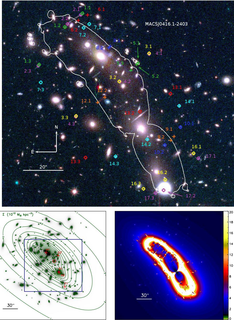
Figure 2.2 Top: False color image of MACS J0416.1-2403 from WFC3/IR (red; F105W, F110W, F125W, F140W, and F160W), ACS (green; F435W, F475W, F606W, F625W, F775W, F814W, and F850LP), and WFC3/UVIS (blue; F225W, F275W, F336W, and F390W) imaging. Labels are the same as in Figure 2.1. Left: Contour map of the total surface mass distribution (in units of 10^{13} M_{\odot} \text{ kpc}^{-2} ) overlaid on the mass contained in cluster member galaxies. The spacing of the contours is linear. The locations and labels of each optimized halo (see Table C.2) are shown in red crosses. The red diamond indicates the location of the reference point. The blue box indicates the field of view of the top image. Right: Absolute value of magnification in the image plane for a source at z = 9 .
