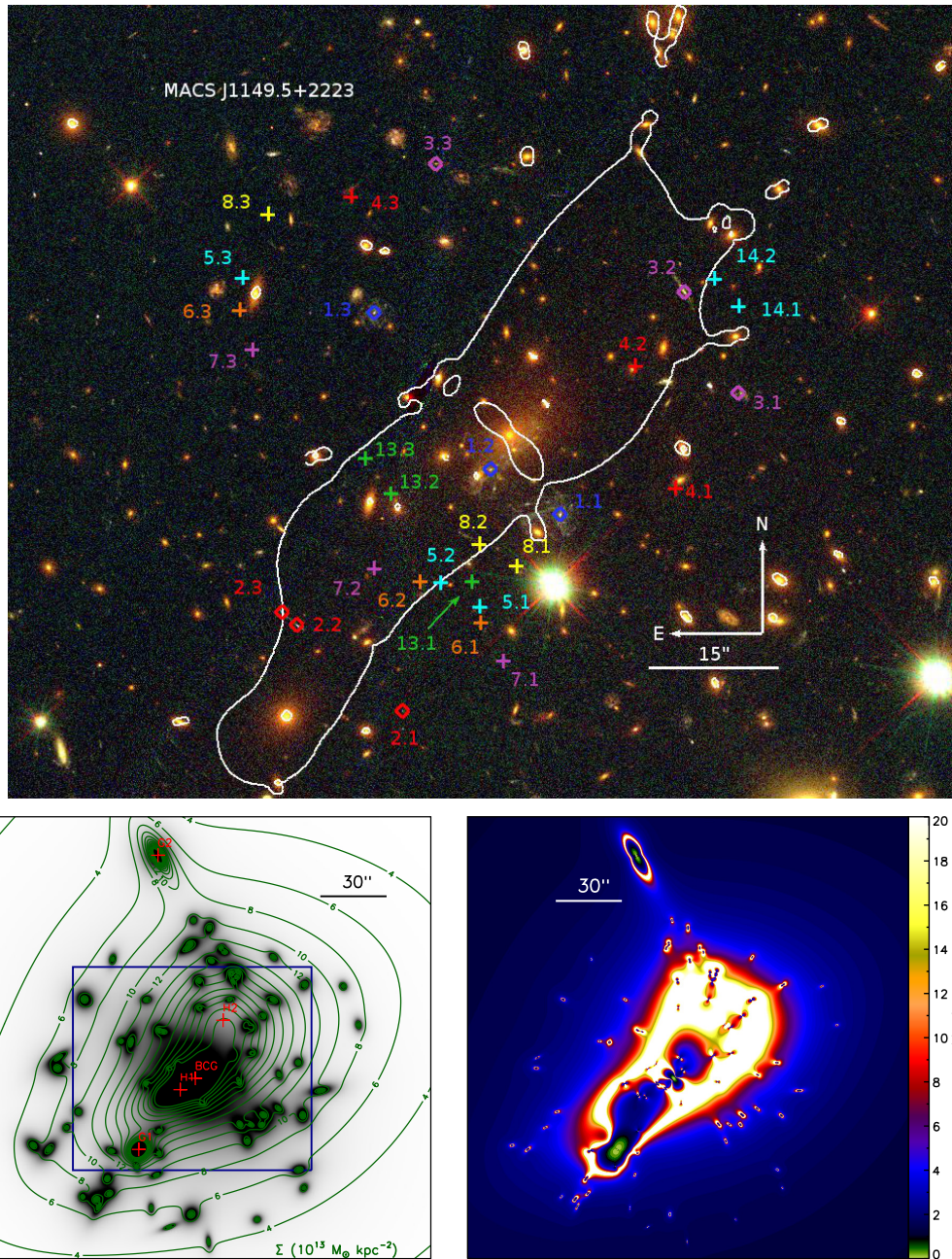
Figure 2.4 Top: False color image of MACS J1149.5+2223 from ACS imaging (red, F814W; green, F606W; blue, F435W). Labels are the same as in Figure 2.1. Left: Contour map of the total surface mass distribution (in units of 10^{13} M_{\odot} \text{ kpc}^{-2} ) overlaid on the mass contained in cluster member galaxies. The spacing of the contours is linear. The locations and labels of each optimized halo (see Table C.4) are shown in red. The blue box indicates the field of view of the top image. Right: Absolute value of magnification in the image plane for a source at z = 9 .
