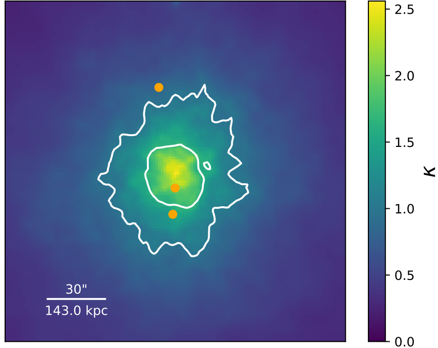
Figure 6.1 Simulated cluster at z = 0.349 created using the HACC code (Habib et al., 2016). Shown \kappa = \Sigma/\Sigma_{\text{crit}} , the surface mass density in units of the critical density for a source at z = 1.9615 . The white line is the critical curve for z = 1.9615 . Shown is example image configuration for a source at z = 1.9615 .
