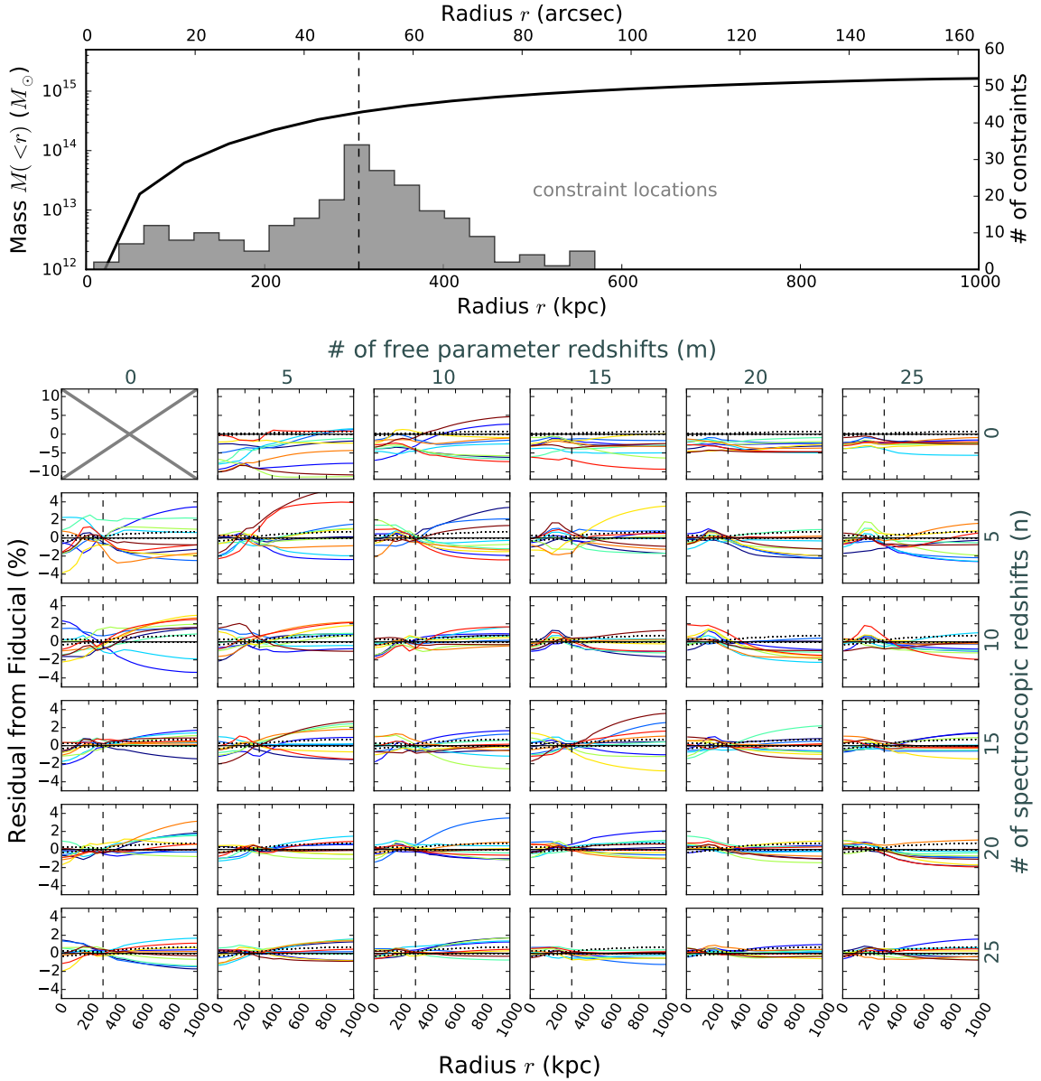
Figure 3.5 (Top) radial mass profile for the fiducial model. The histogram shows the projected radii of all the constraints used in the model. The dashed vertical line is the median projected radius of the arcs at r_{\text{arcs}} = 305 kpc. (Bottom) Radial mass profile residuals from the fiducial model for all test models with different numbers of spectroscopic and free parameter redshifts used as constraints. The dotted lines represent the 1\sigma statistical error in the fiducial model mass profile estimated from the MCMC. The dashed vertical line matches r_{\text{arcs}} from the top plot. Note: the top row ordinates have a different scale from the other plots.
