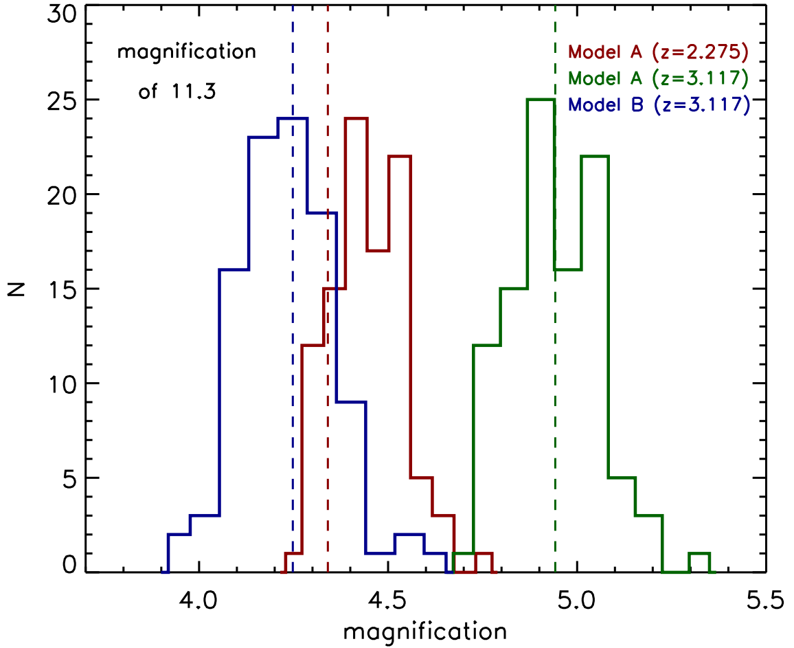
Figure 2.8 We plot the magnifications of image #11.3 from Model A (the redshift of image system #11 is a free parameter in the model) and Model B (the redshift of image #11 is fixed to the spectroscopic redshift). For Model A, we derive the magnification for two source plane redshifts: the model-predicted redshift of the image system z = 2.275 (red) and the spectroscopic redshift z = 3.117 (green). Model B (blue) is set to the spectroscopic redshift. The dashed lines represent the value of magnification of the best-fit model.
