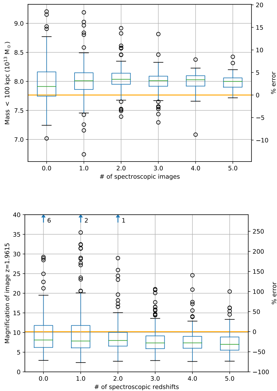
Figure 6.2 (Top) The distribution of derived mass within 100 kpc of the simulated cluster core from 1024 lens models with varying numbers of known (“spectroscopic”) redshifts. (Bottom) The distribution of derived magnifications for the top image in Figure 6.1 at z = 1.9615 . (Both) The orange horizontal lines indicate the values calculated from the true mass and magnification of the simulated cluster.
