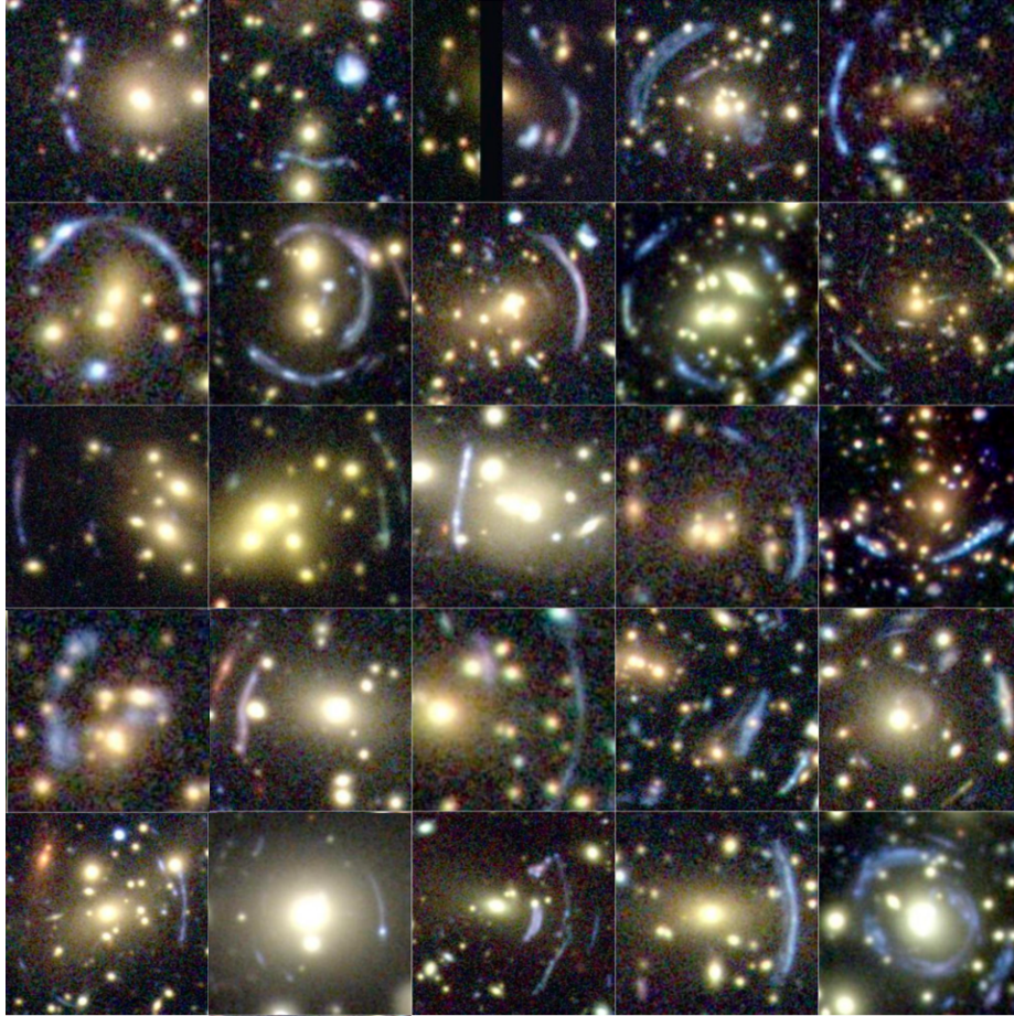
Figure 1.9 A selection of the best lensing clusters found in the Sloan Giant Arc Survey. Each image is gri 5 min exposures with Gemini /GMOS. Image credit: M. Bayliss.
