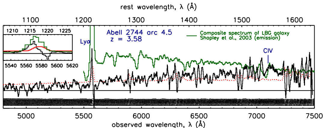
Figure A.9 One-dimensional and two-dimensional spectra of Abell 2744 arc 4.5. The noise level of the one-dimensional spectrum is plotted in red. We over plot a composite spectrum of high-redshift ( z = 3 ) Lyman break galaxies with strong Lyman \alpha emission from Shapley et al. (2003) to show similarities in these spectral features as well as Lyman break in the continuum. The Lyman \alpha emission line lies slightly blueward of the 5577\text{\AA} skyline residual, as shown in the inset in the upper left. We find a likely solution of z = 3.58 for this galaxy.
