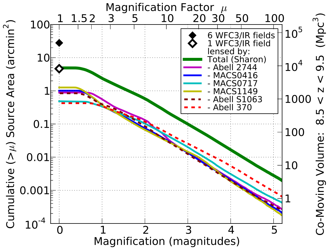
Figure 2.9 We show the cumulative area and co-moving volume of background sources at 8.5 < z < 9.5 lensed by each of the HFF clusters to magnification \mu and higher. We show, for reference, the corresponding area and co-moving volume of a one and six WFC3/IR FOVs (diamonds).
