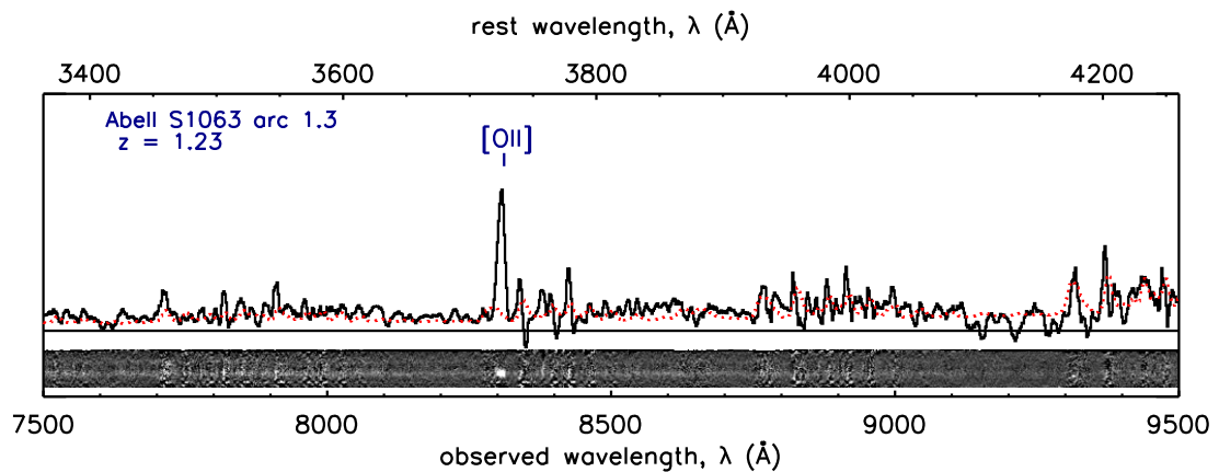
Figure A.1 One-dimensional and two-dimensional spectra of Abell S1063 arc 1.3. The noise level of the one-dimensional spectrum is plotted in red.
