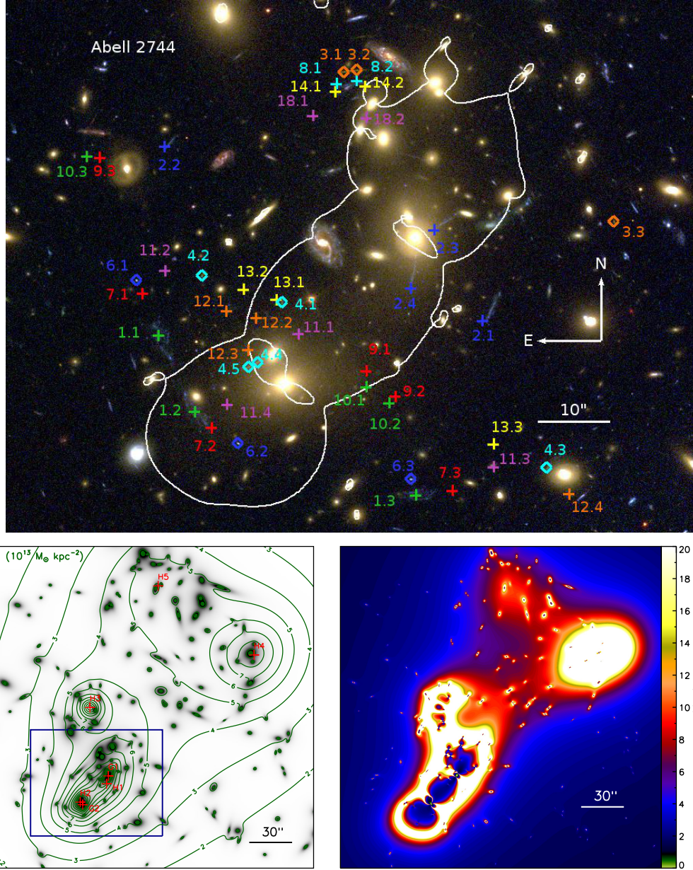
Figure 2.1 Top: False color image of Abell 2744 from archival ACS imaging (red, F814W; green, F606W; blue, F435W) obtained as part of GO program 11689 (PI: R. Dupke). The locations of multiply imaged galaxies used as constraints in the model of Abell 2744 are overlaid. Diamonds designate image systems with spectroscopic redshifts, where crosses indicate that the redshift of the image system is left as a free parameter in the model. The critical curves (white) trace the region of high magnification for a source at z = 2 . Left: Contour map of the total surface mass distribution (in units of 10^{13} M_{\odot} \text{ kpc}^{-2} ) overlaid on the mass contained in cluster member galaxies. The spacing of the contours is linear. The locations and labels of each optimized halo (see Table C.1) are shown in red. The blue box indicates the field of view of the top image. Right: Absolute value of magnification in the image plane for a source at z = 9 .
