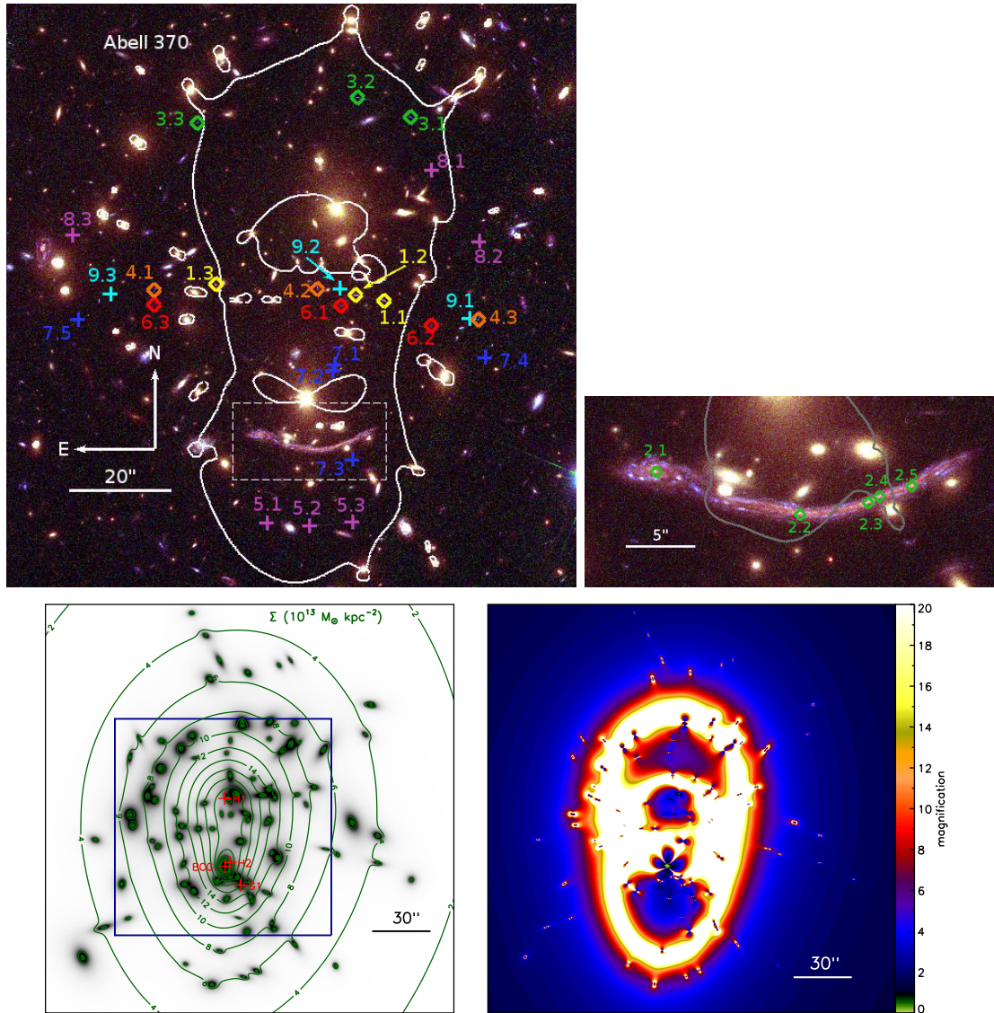
Figure 2.6 Top left: False color image of Abell 370 from archival ACS imaging (red, F814W; green, F606W; blue, F435W) by HST SM4 ERO program 11597 (PI: K. Noll), program 11591 (PI: J.-P. Kneib), program 11582 (PI: A. Blain), and program 11108 (PI: E. Hu). Labels are the same as in Figure 2.1. Top right: The inset shows the image constraints of the giant arc (image system #2); the gray line is the critical curve corresponding to the spectroscopic redshift of this arc, z = 0.725 . Bottom left: Contour map of the total surface mass distribution (in units of 10^{13} M_{\odot} \text{ kpc}^{-2} ) overlaid on the mass contained in cluster member galaxies. The spacing of the contours is linear. The locations and labels of each optimized halo (see Table C.6) are shown in red. The blue box indicates the field of view of the top image. Bottom right: Absolute value of magnification in the image plane for a source at z = 9 .
