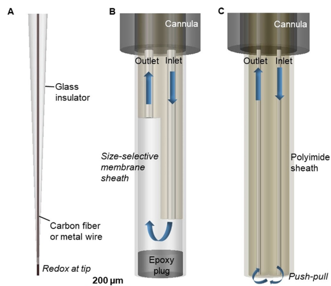
Figure 1. Schematic of conventional probes for in vivo neurochemical monitoring with comparison of probe sizes. A) Electrochemical microelectrode with 10 \mu\text{m} diameter, 50 \mu\text{m} long. B) Concentric microdialysis probe with 1 mm long polyacrylonitrile (PAN) membrane with 230 \mu\text{m} o.d. C) low flow push-pull probe made assembly of 20 \mu\text{m} i.d./ 90 \mu\text{m} o.d. capillaries side-by-side, sheathed with 180 \mu\text{m} i.d./ 220 \mu\text{m} o.d. polyimide tubing. Models were drawn to scale for comparison of probe size and regions of chemical monitoring (at exposed electrode surface for (A), membrane surface for (B), and space between orifices for (C)).
