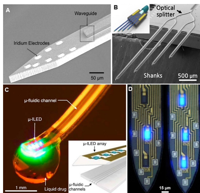
Figure 4. Examples of microfabricated probes with optical elements. A) Neural probe with an oxynitride waveguide and iridium electrodes. [195] B) SU-8 waveguide, multi-shank probe for stimulation at varied depths. [198] C) Multilayered probe with microfluidic channels and \mu\text{LED} 's. [200] D) Expanded view of \mu\text{LED} 's from 4-shank probe design. [205]
