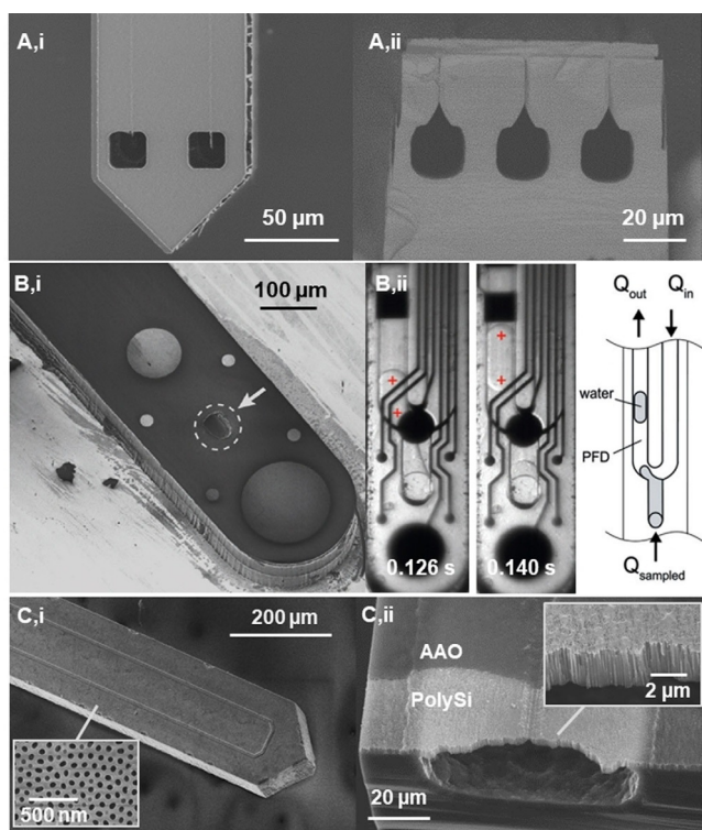
Figure 3. Examples of microfabricated probes for sampling. A) Push-pull probe: orifices for sampling (A,i) and cross-section of a probe with additional channel (A, ii); B) Direct sampling probe, an arrow indicates a single sampling orifice (B,i). This probe is integrated with electrical recording and stimulation (circle dots), and flow-segmentation (B, ii). [153] C) Dialysis probe: Top view of probe tip (C,i) with AAO membrane in the inset, and cross-section (C,ii) of a microchannel with embedded AAO-poly Si membranes. [163]
