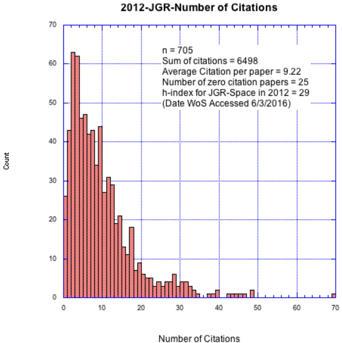
Figure 1. The distribution of citations for the 705 papers that appeared in JGR-Space Physics in 2012 from Thomsen-Reuters ISI-WoS accessed on 3 June 2016. The median citation count is 7, while the mean is 9.22.
