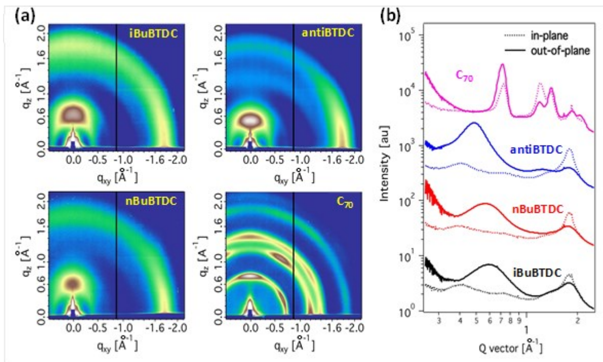
Figure 4. a) Two-dimensional grazing incidence X-ray diffraction (GIXD) scattering patterns of vacuum deposited donor and acceptor thin films; and b) the corresponding line cut profiles.
