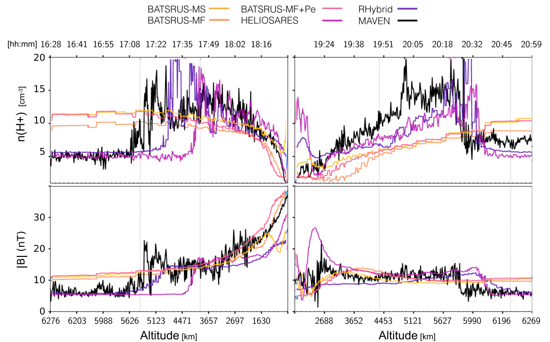
Figure 3. Flythrough of model results of the inbound and outbound portions of the orbit (#2349, 14 December 2015) excluding periapsis with corresponding MAVEN data. Panels show H^+ number density and magnetic field magnitude. The location at which the orbit passes through the analytic boundary locations (Trotignon et al., 2006) for the bow shock and MPB/IMB are plotted as vertical dashed lines.
