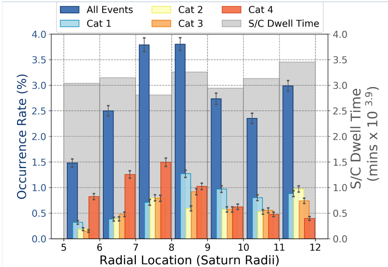
Figure 9. Radial distribution of interchange events from 2005 - 2016. Superimposed on the total sampling time the spacecraft spent in each radial bin of 1 R_s (the grey shaded region), we demonstrate by category of event the occurrence rates of interchange (the colored bars). We have binned our data by 1 R_s to prevent any sampling bias. Each bar plotted represents a 1 R_s range. The dark blue bars represent all categories combined.
