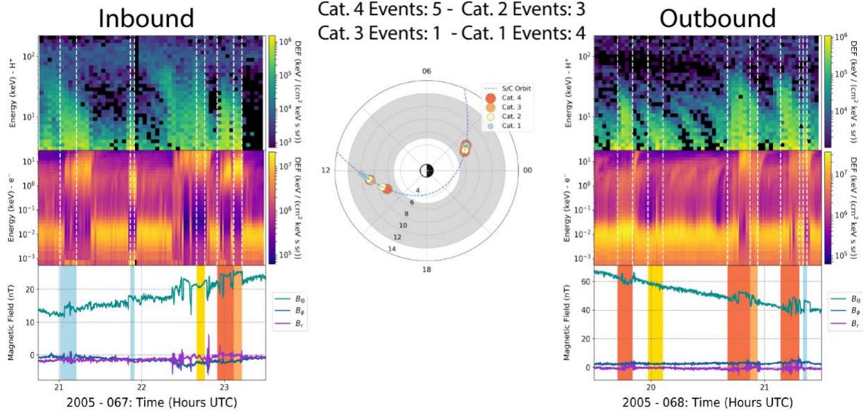
Figure 4. Cassini orbit pass and categorical events classifications identified for Day Of Year (DOY) 66 – 71 of 2005. This figure demonstrates the different categories of events within one orbit pass in the beginning of 2005. The panels marked inbound and outbound represent selected portions of a single orbit trajectory, with the top sub-panel displaying CHEMS H+ differential energy flux between 3 and 220 keV, followed by the CAPS ELS differential energy flux for electrons from Anode 4, and finally the magnetic field components in KRTP (Kronocentric body-fixed, J2000 spherical Coordinates). We did not use the MAG or ELS data to identify events but we do display it here for illustration purposes. In the outbound panel we can observe how injection events may or may not show a demonstrated magnetic field enhancement. The middle panel represents the orbit of Cassini, with the region allowable for the algorithm shaded in grey. The orbit of Cassini is the blue dashed line plotted in local time in hours and radial distance in units of Saturn Radii. In the orbit and magnetic field plots the most intense events are marked with dark orange, with least intense in light blue. In the CHEMS and CAPS panels the event boundaries are marked with dashed white lines.
