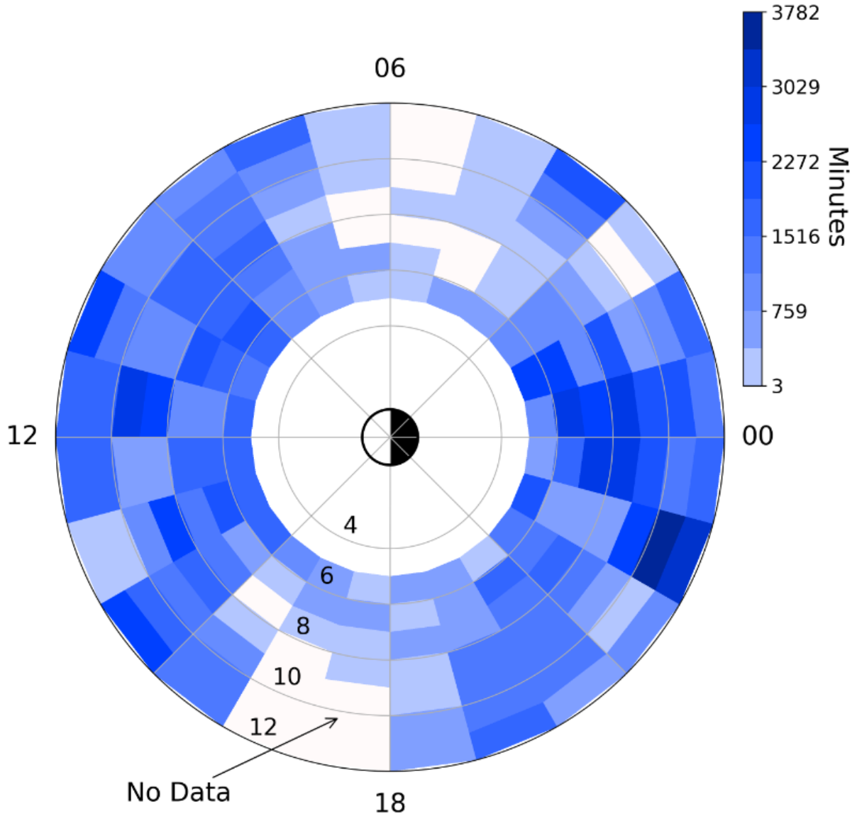
Figure 2. Spacecraft dwell time from 2005-2016 representing the sample size of the CHEMS H + dataset. Each region shows the total minutes occupied by Cassini that satisfy our selection criteria. This figure demonstrates the dwell time calculated from CHEMS timestamps of the Cassini spacecraft within the radial range of 5 – 12 R s and at latitudes below 10° in SZS arranged by local time where noon is on the left of the figure. Bins with no data are shown in gray.
