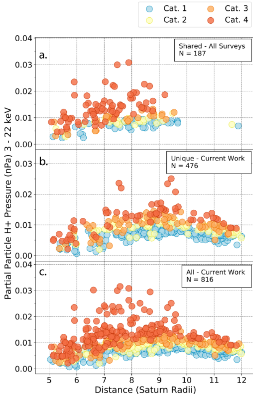
Figure 8. Comparison of identified event partial particle pressure (3 – 22 keV H+) to previous surveys. a) Partial particle pressure of interchange events cross listed in all surveys. This panel
