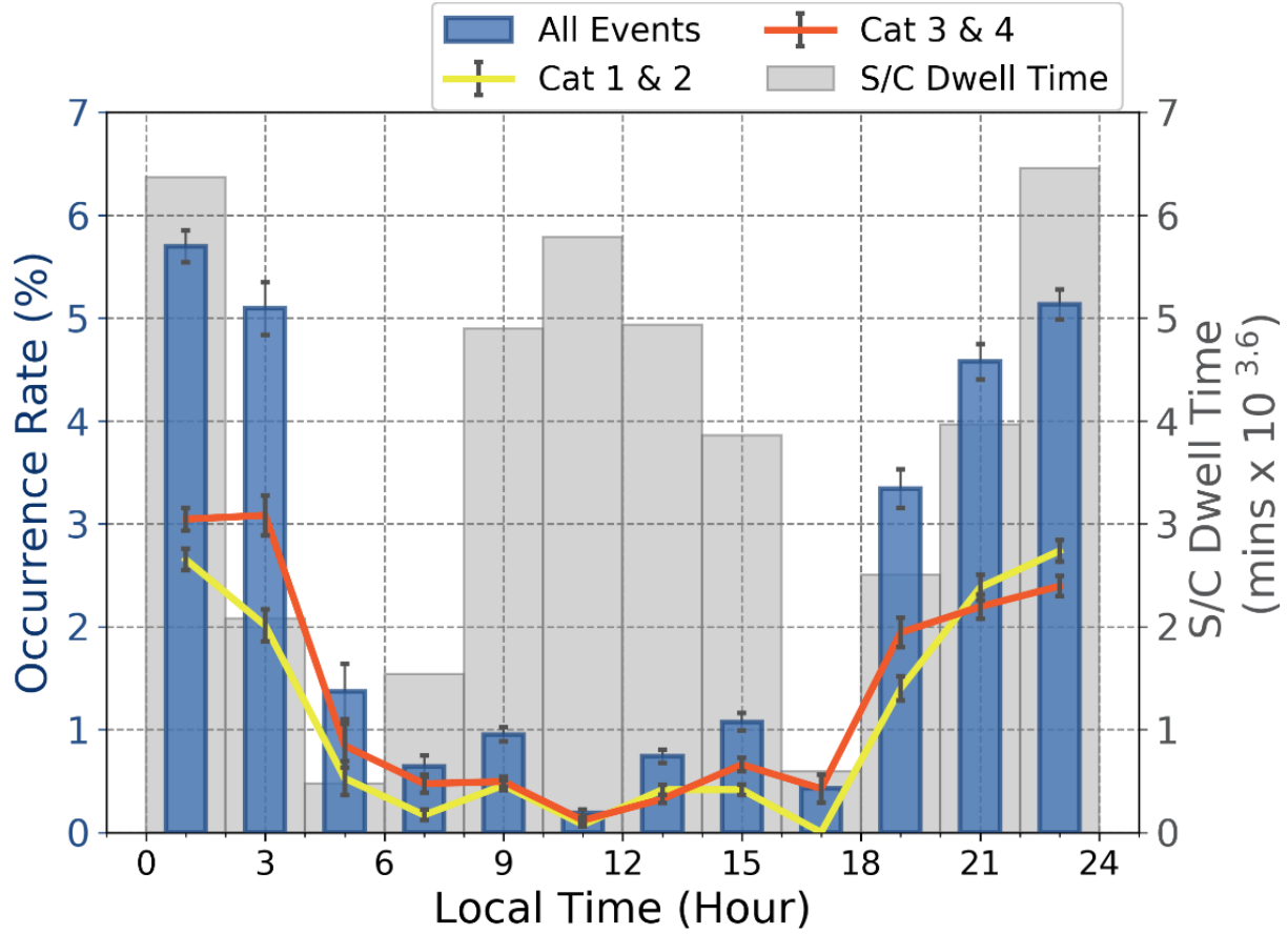
Figure 10. Local time distribution of interchange injection events over all years from 2005 – 2016. Superimposed on the total sampling time that the spacecraft spent in each local time bin of 2 hours (the grey shaded region), we present by grouped category of interchange the occurrence rates (time in event / total observation time) as a function of local time (blue bars and colored lines). The blue bars represent all interchange injections while the yellow and orange lines represent the rates of low intensity (cat 1 and 2) and high intensity (cat 3 and 4), respectively.
