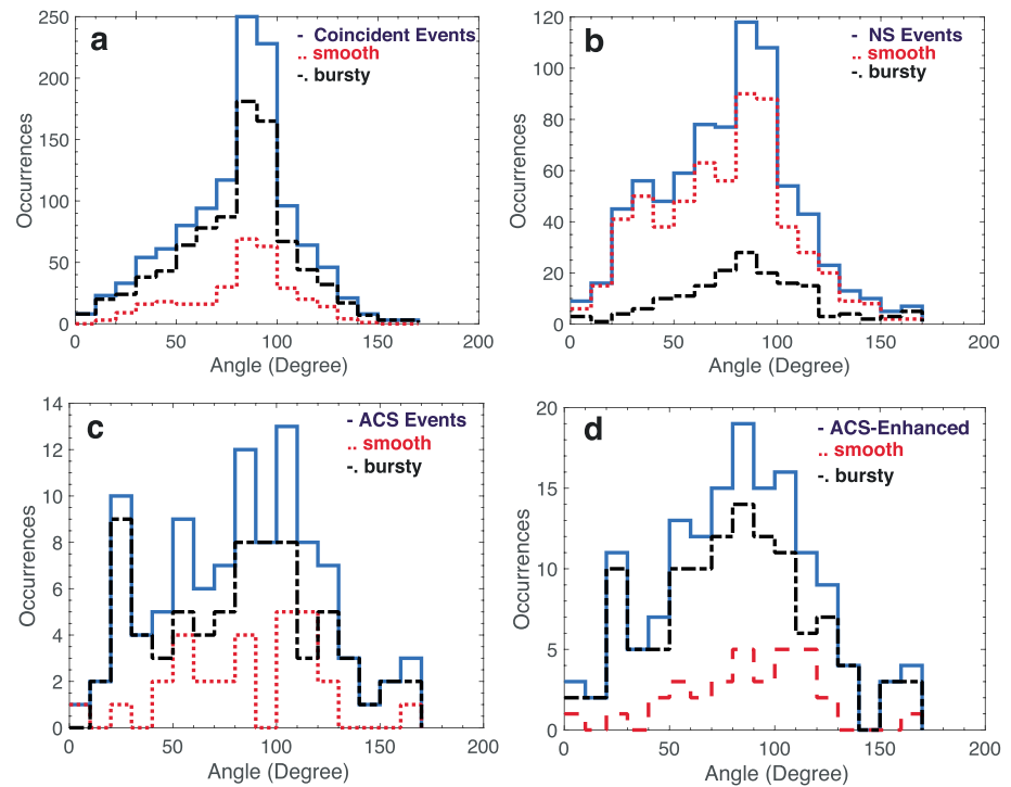
Figure 13. Histograms of the angle between the measured magnetic field vector and y axis of the spacecraft in Mercury solar orbital coordinates. (a) Coincident events; (b) neutron spectrometer (NS)-only events; (c) anticoincidence shield (ACS)-only events; and (d) ACS-enhanced events.
