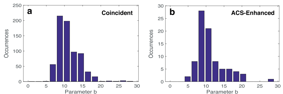
Figure 10. (a) Histograms of parameter b of the exponential fit for Coincident events and (b) for anticoincidence shield (ACS)-enhanced events. This parameter is a proxy for the hardness of spectrum, where larger b indicates a harder spectrum. Based on the two-sample Kolmogorov-Smirnov goodness-of-fit hypothesis test, the two histograms follow a statistically similar distribution.
