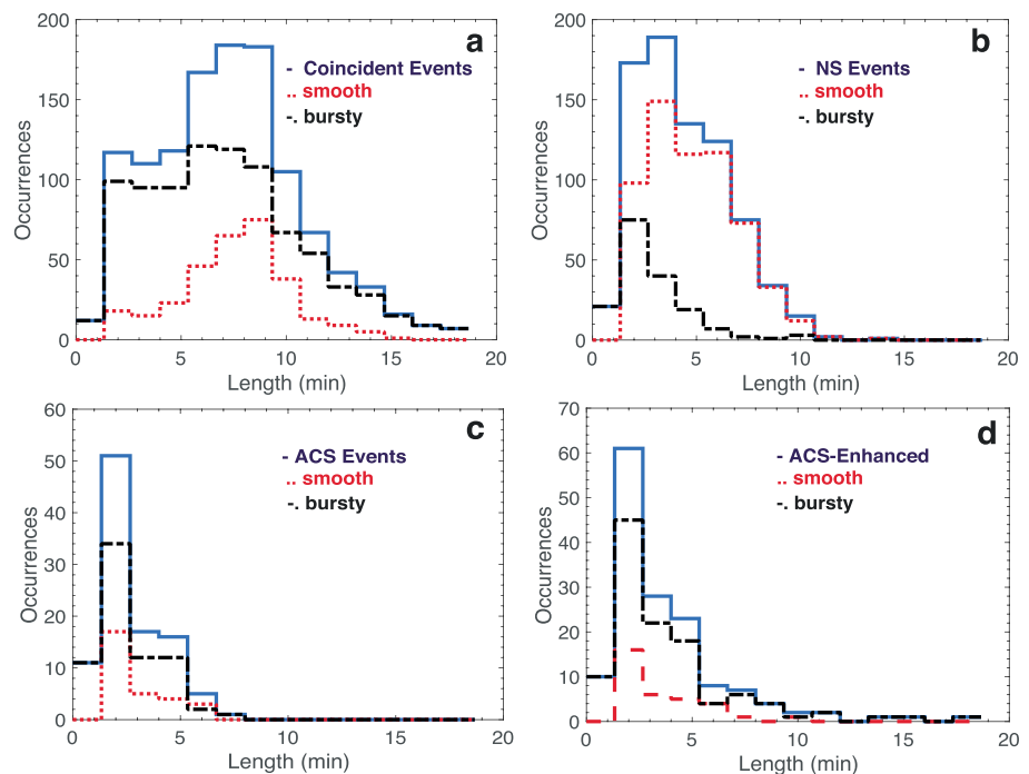
Figure 3. Histograms of the energetic electron event duration for (a) Coincident, (b) neutron spectrometer only, (c) anticoincidence shield (ACS) only, and (d) ACS enhanced. Histograms of smooth and bursty events are shown in red and black, respectively, for each class.
