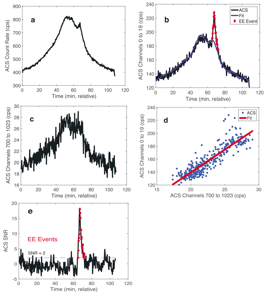
Figure 1. An example of an energetic electron (EE) event detected by anticoincidence shield (ACS) on 9 May 2013 between 16:42 UT and 16:50 UT. (a) The ACS count rate data for the near-planet portion of orbit 1962. (b) The ACS low-energy channel count rate data and the fit of ACS low-energy channel data to high-energy channel data are shown in black and blue lines, respectively. The EE event is marked in red diamonds. (c) The ACS high-energy channel count rate data. (d) Low-energy channel data versus high-energy channel data for the same period of Figure 1a. Individual data points are plotted in blue circles, while the linear fit is plotted in red. (e) The ACS signal-to-noise ratio (SNR) for the data during the same period. The EE event is plotted in red diamonds. The dashed line shows the SNR = 2 threshold.
