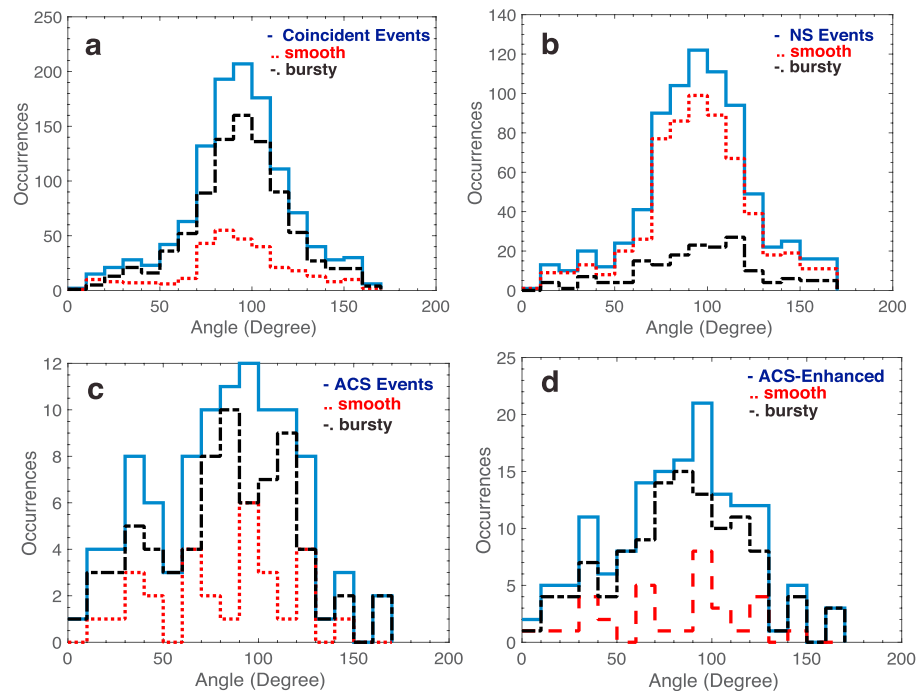
Figure 14. Histograms of the angle between the measured magnetic field vector and z axis of the spacecraft in Mercury solar orbital coordinates. (a) Coincident events; (b) neutron spectrometer (NS)-only events; (c) anticoincidence shield (ACS)-only events; and (d) ACS-enhanced events.
