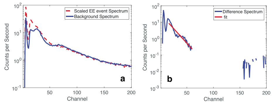
Figure 9. (a) Energy deposition spectra in gamma-ray spectrometer anticoincidence shield from the event on 2 February 2014. Average energy counts for the energetic electron (EE) event and for the whole orbit without the EE event are shown in dashed red and solid blue, respectively. The trough and peak at the lowest channels (1 to 15) are due to a lower-level discriminator cut off and noise counts in the electronics. The statistical uncertainties on these spectra are roughly a factor of 2 to 3 larger than the point-to-point scatter in the data. (b) The difference spectrum and the corresponding exponential fit ( y = ae^{-b} ) (or linear in a logarithmic scale ( y = a_1 - \frac{x}{b} ), where a_1 = \log a ) are shown in blue and red, respectively. The linear fit parameters are a_1 = 3.26 \pm 0.27 and b = 11.06 \pm 0.77 .
