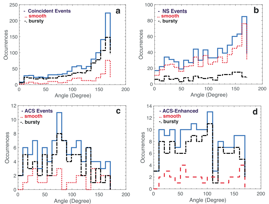
Figure 12. Histograms of the angle between the measured magnetic field vector and x axis of the spacecraft in Mercury solar orbital coordinates. (a) Coincident events; (b) neutron spectrometer (NS)-only events; (c) anticoincidence shield (ACS)-only events; and (d) ACS-enhanced events.
