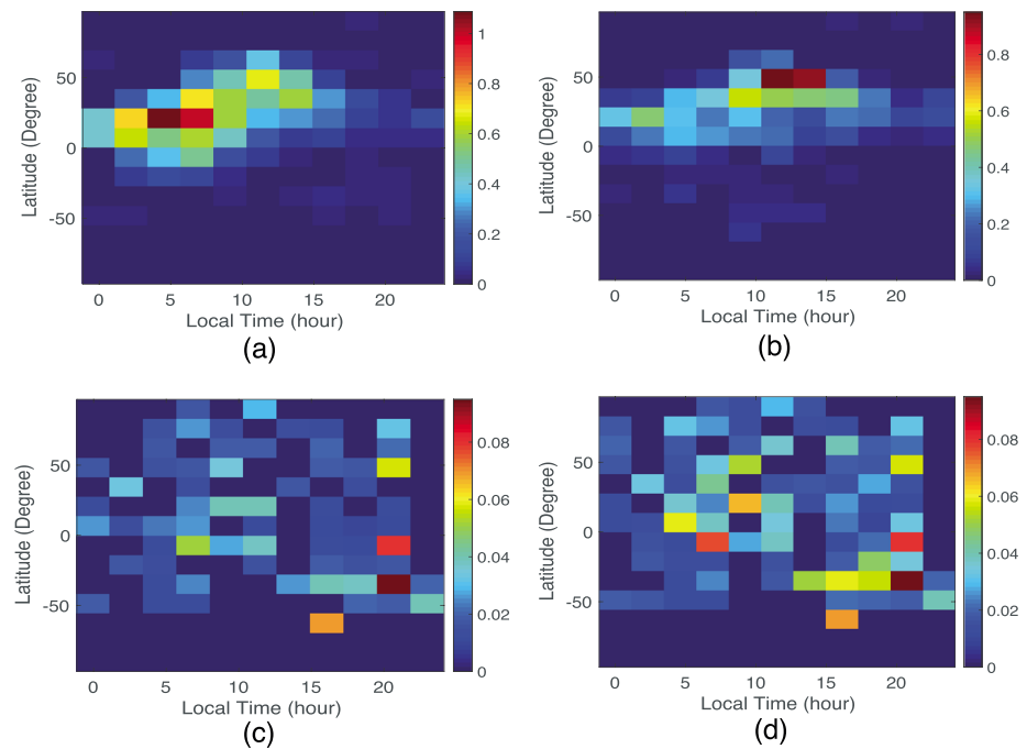
Figure 8. Normalized occurrences of events for local time and latitude. (a) Coincident events; (b) neutron spectrometer only events; (c) antineutrino shield (ACS)-only events; and (d) ACS-enhanced events.
