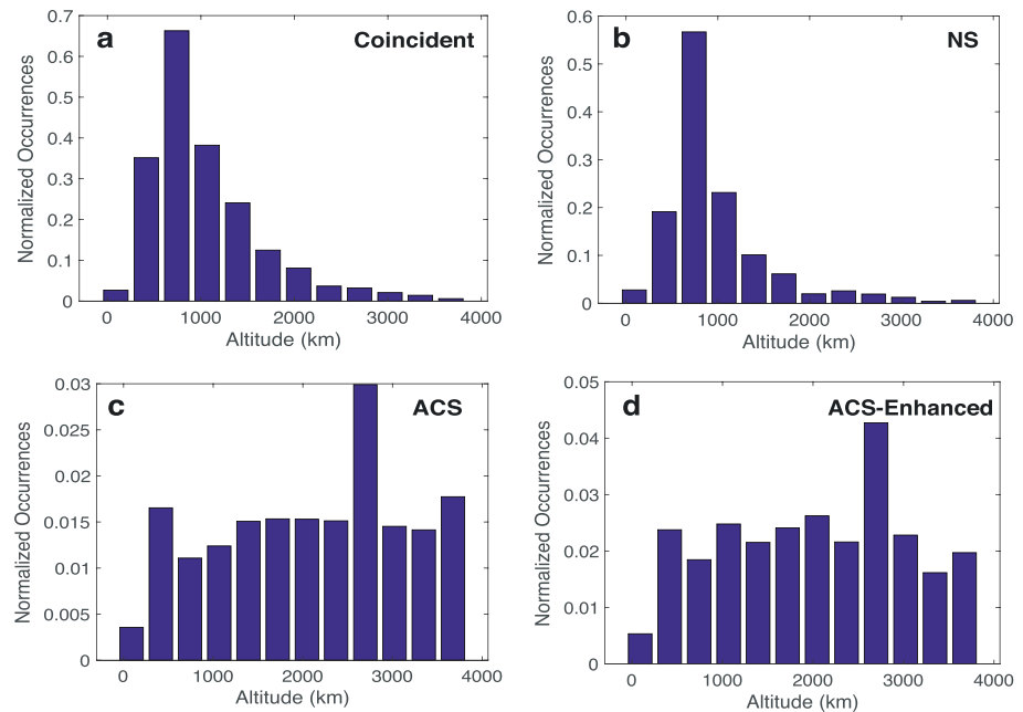
Figure 6. Normalized occurrences of events binned by altitude. (a) Coincident events; (b) neutron spectrometer (NS)-only events; (c) anticoincidence shield (ACS)-only events; and (d) ACS-enhanced events.
