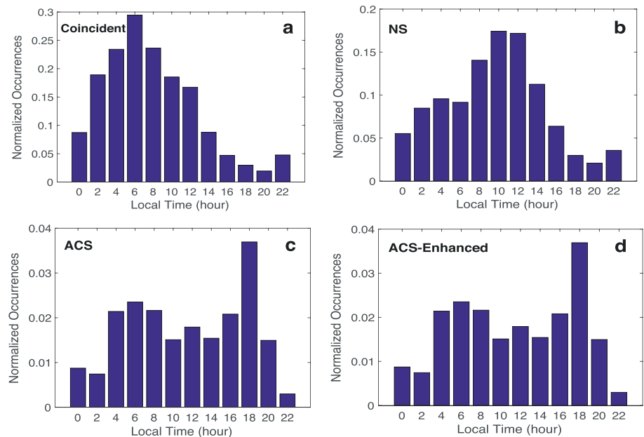
Figure 7. Normalized occurrences of events binned by local time. (a) Coincident events; (b) neutron spectrometer (NS)-only events; (c) anticoincidence shield (ACS)-only events; and (d) ACS-enhanced events.
