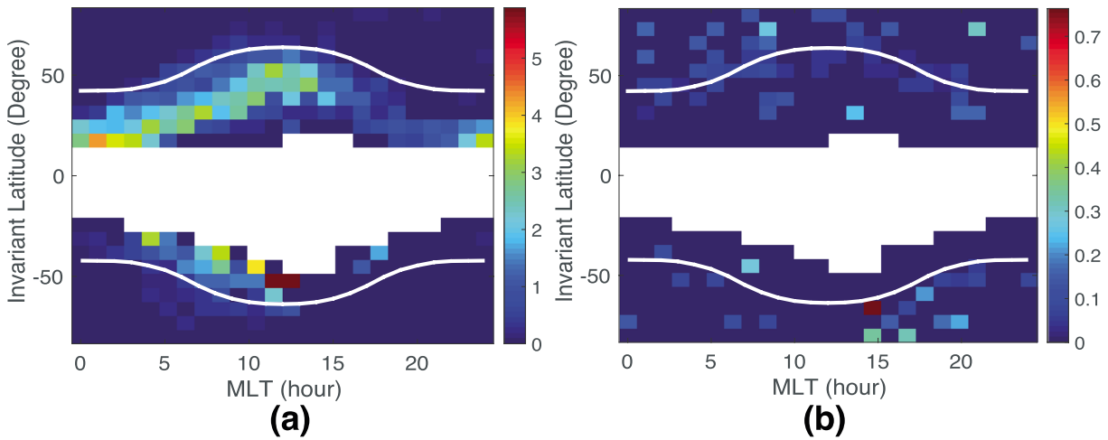
Figure 11. Two-dimensional normalized histograms of energetic electron events for invariant latitude versus magnetic local time (MLT). (a) Coincident events. (b) Anticoincidence shield enhanced events. The normalization is performed based on the MLT-invariant latitude space covered by the spacecraft for the entire time between 1 March 2013 and 30 April 2015, when the spacecraft altitude was 4,000 km or less from Mercury surface. The modeled boundary between the open and closed field lines is shown by the white lines. The white area between \pm 20^\circ invariant latitude indicates that the spacecraft was never located in these areas.
