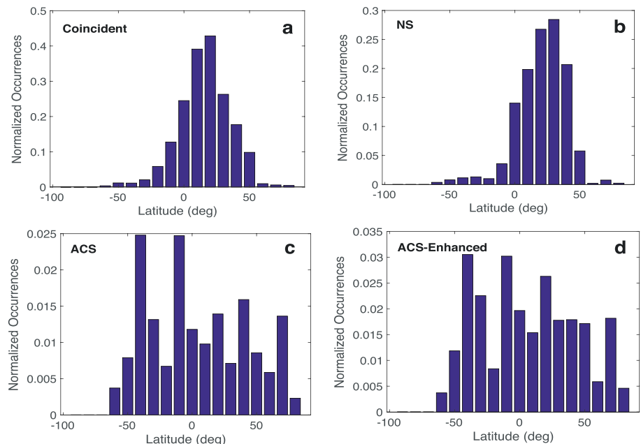
Figure 5. Normalized occurrences of events binned by latitude. (a) Coincident events; (b) neutron spectrometer (NS)-only events; (c) anticoincidence shield (ACS)-only events; and (d) ACS-enhanced events.
