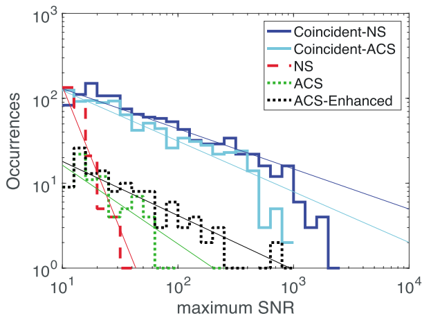
Figure 4. Histograms of maximum signal-to-noise ratio (SNR) for Coincident events. Neutron spectrometer (NS) values and anticoincidence shield (ACS) values for coincident events are plotted in blue and cyan, respectively; red and green traces show histograms of NS-only and ACS-only events. All histograms follow a power law distribution (thin lines) with power law indices of -0.47 \pm 0.11 , -0.59 \pm 0.08 , -3.36 \pm 0.4 , -0.92 \pm 0.38 , and -0.63 \pm 0.23 for Coincident (NS), Coincident (ACS), NS-only, ACS-only, and ACS-enhanced, respectively.
