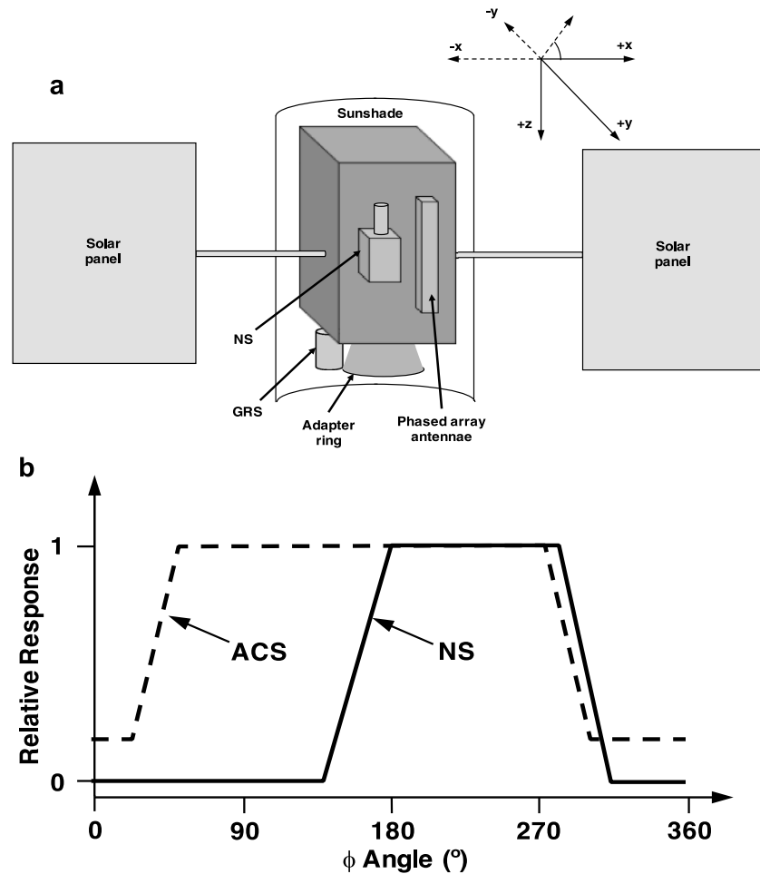
Figure 15. (a) Schematic view of the MESSENGER spacecraft where specific components relevant to this study are labeled including the neutron spectrometer (NS), gamma-ray spectrometer (GRS), adapter ring, and phased array antennae. The spacecraft coordinate system is shown in the upper right, where the angle \phi is given in the x - y plane. \phi = 90^\circ represents electrons traveling in the -y axis to +y axis direction. (b) Schematic response of the NS (solid) and anticoincidence shield (ACS; dashed) as a function of \phi angle.
