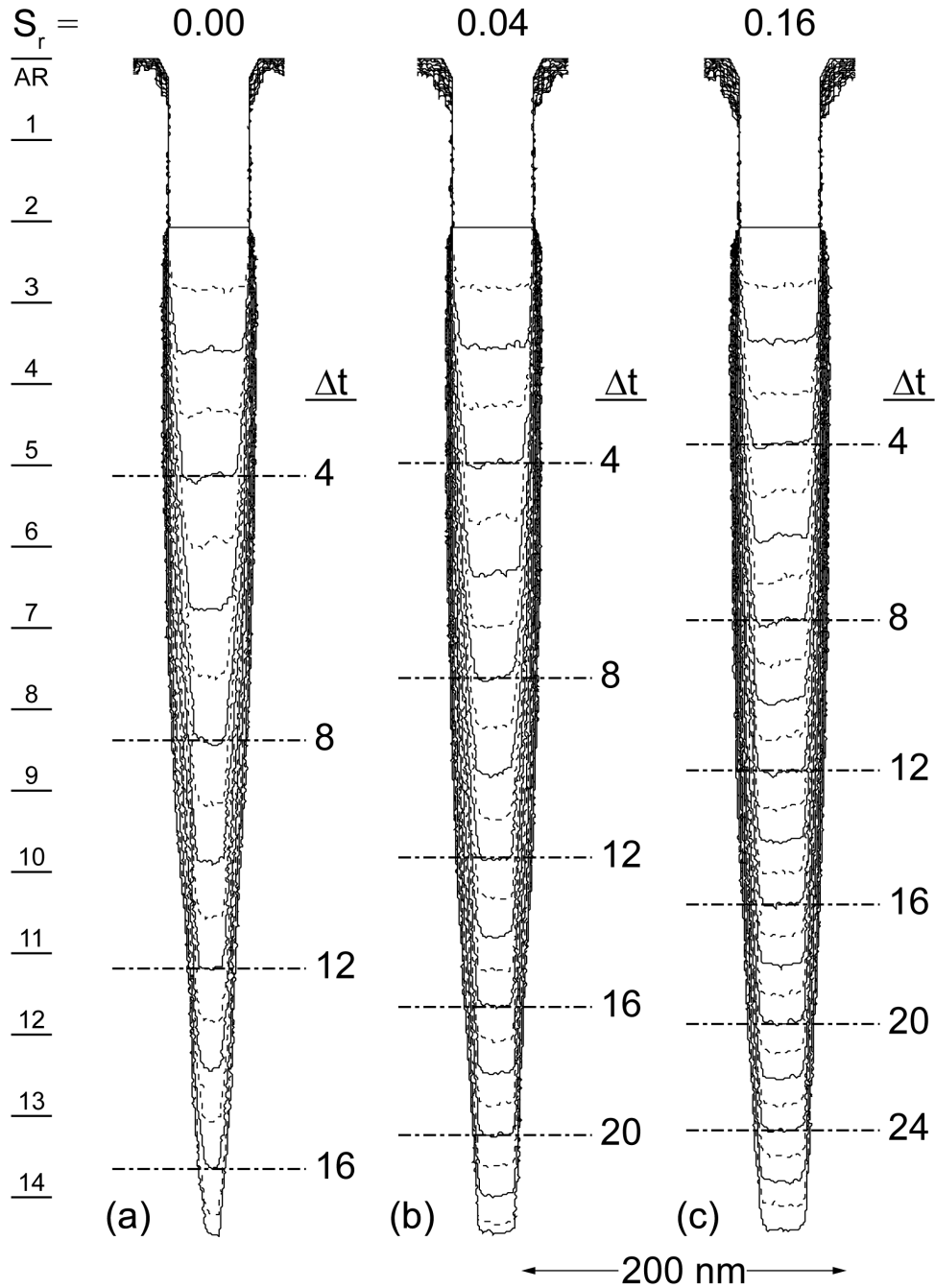
Fig. 4.12 Time evolution of silicon trench profile during \text{Ar}/\text{Cl}_2 etching for different chlorine recombination probabilities, S_r . The recombination probabilities of atomic Cl on \text{SiCl}_3 shown are (a) 0.00, (b) 0.04 and (c) 0.16. Line spacing represents a constant time interval \Delta t for all profiles. Numbered lines represent similar etch times in each profile.
