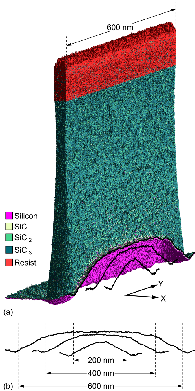
Fig. 4.5 Longitudinal slice (Y-direction) through the center of the trench in the 3-d FinFET, showing the etch front (solid lines) for three fin lengths: 200, 400 and 600 nm. (a) Perspective view with each color representing a different material. (b) Height at the bottom of the trench in the longitudinal (Y-direction) for different fin lengths. (The nominal fin lengths are shown as dotted lines for reference.)
