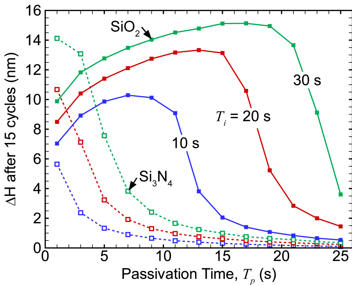
Fig. 7.7 Total change in height ( \Delta H ) of the surface of \text{SiO}_2 or \text{Si}_3\text{N}_4 (not including overlayer) after 15 ALE cycles as a function of passivation time ( T_p ) for ion bombardment times ( T_i ) of 10, 20 and 30 s. \text{SiO}_2 ALE is shown as solid lines, \text{Si}_3\text{N}_4 as dotted lines.
