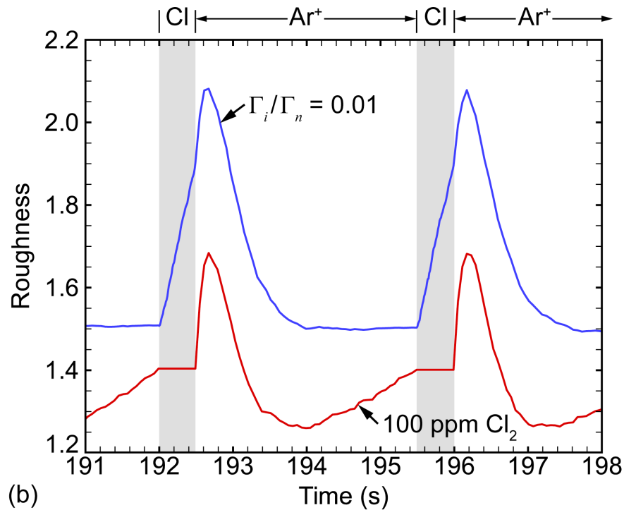
Fig. 5.5 Surface roughness as a function of time. (a) First 25 pulses for \Gamma_i/\Gamma_n = 0.02 , 0.01 , 10^{-3} and 10^{-4} in the passivation step, showing the transient roughening at early etch times. (b) Sub-cycle roughening behavior at steady-state ( 55^{\text{th}} pulse) for \Gamma_i/\Gamma_n = 0.01 in the passivation phase and 100 \text{ ppm Cl}_2 in the ion bombardment phase. ALE sub-cycles are listed at the top, with the passivation phase highlighted with grey in the figure.
