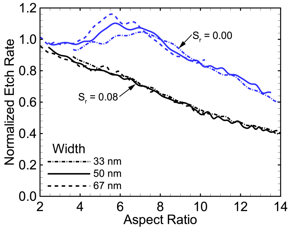
Fig. 4.18 Etch rate as a function of aspect ratio and trench width for two values of chlorine recombination rate, S_r . For the base case, S_r = 0.08 , the etch rate depends only on aspect ratio and not trench width. For the case without chlorine recombination, S_r = 0.00 , the peak in etch rate weakly depends on trench width, but at higher aspect ratios the ARDE trends are again independent of trench width.
