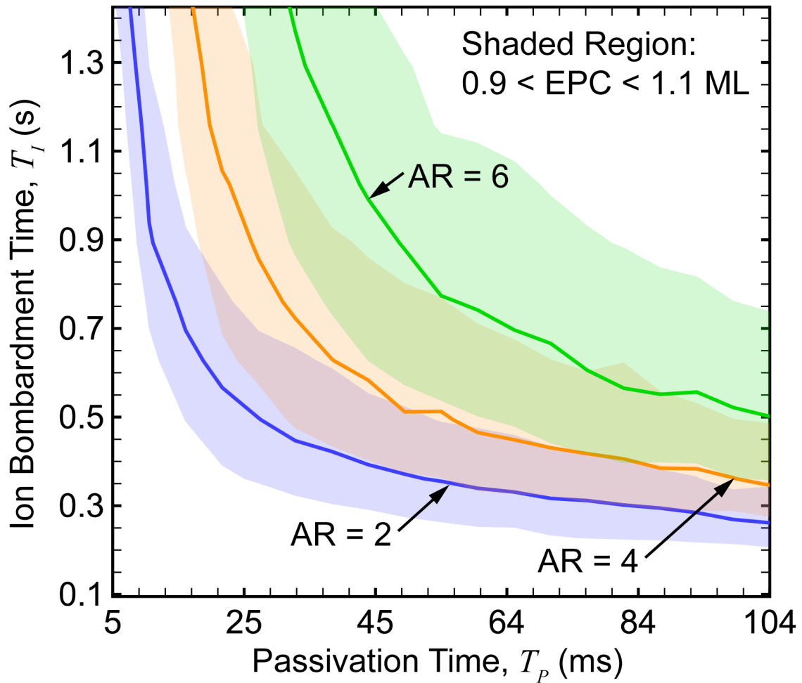
Fig. 5.12 Trend of etch depth per cycle (EPC) as a function of ion bombardment time ( T_I ) and passivation time ( T_P ). The solid line represents an EPC of 1, and the shaded region is the window from 0.9 < \text{EPC} < 1.1 .
