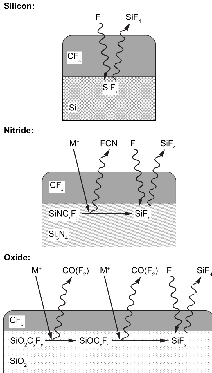
Fig. 3.1 Schematic of the Si, Si 3 N 4 and SiO 2 etching mechanisms. The term M + denotes activation from any ion or hot neutrals. Straight lines through the polymer overlayer imply ion implantation, while wavy lines represent diffusion through the overlayer.
