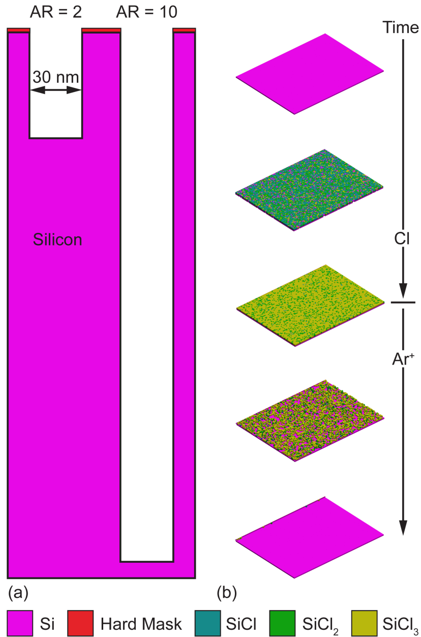
Fig. 5.1 Schematic of the ideal ALE process. (a) Schematic of the initial trench geometry used for ideal ALE simulations. (b) View of the etch front at multiple times, with different colors representing different materials. Time increases from top to bottom, but not with equal steps between images.
