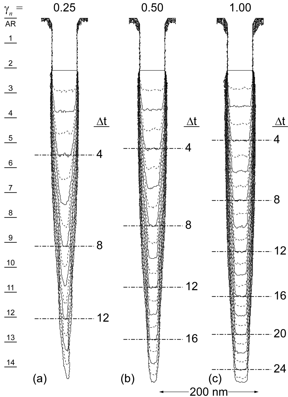
Fig. 4.14 Time evolution of silicon trench profile for different neutral angular distributions, \gamma_n . The normalized angular distribution scaling factors are (a) 0.25, (b) 0.50 and (c) 1.00. Line spacing represents a constant time interval \Delta t for all profiles. Numbered lines represent similar etch times in each profile.
