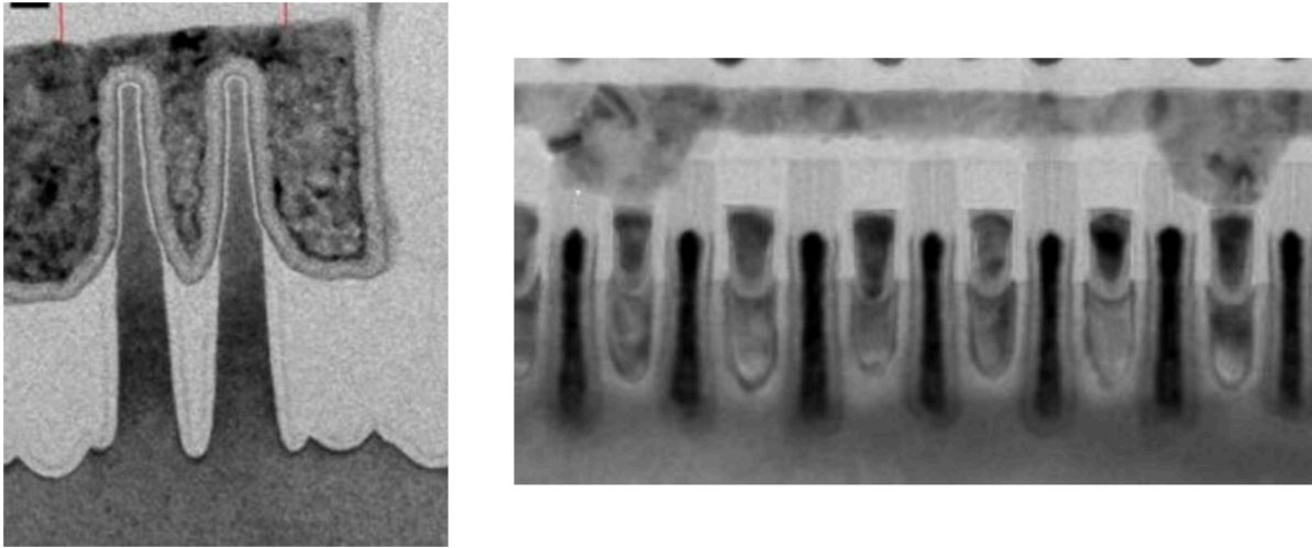
Fig. 1.8 Two cross sectional scanning electron microscope images of the gate structure in Intel's 10 nm process. In order to take these images, the transistors were cut using focused ion beam milling to expose the cross-sectional view. Reproduced from Auth et al..[65]
