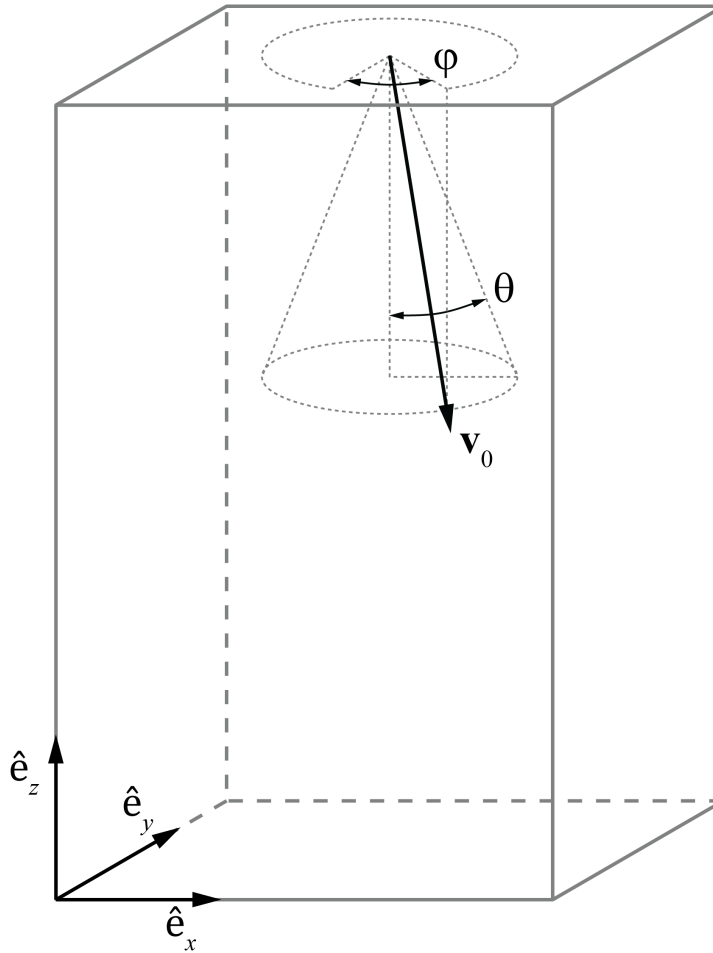
Fig. 2.1 Illustration of the simulation domain showing the origin and cardinal coordinates \hat{e}_x , \hat{e}_y , and \hat{e}_z . An initial velocity vector, \mathbf{v}_0 , is shown along with the polar ( \theta ) and azimuthal ( \phi ) angles.
