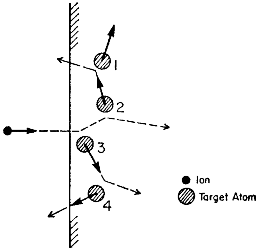
Fig. 1.7 Two different three body collision cascades which result in sputtering. Target atom 2 undergoes a collision with the incoming ion, then a second collision with target atom 1 before being ejected from the solid. Target atom 3 undergoes a collision with the incoming ion, then transfers (some of) the kinetic energy from the ion collision to atom 4, which is ejected from the solid. Reproduced from Sigmund.[13]
