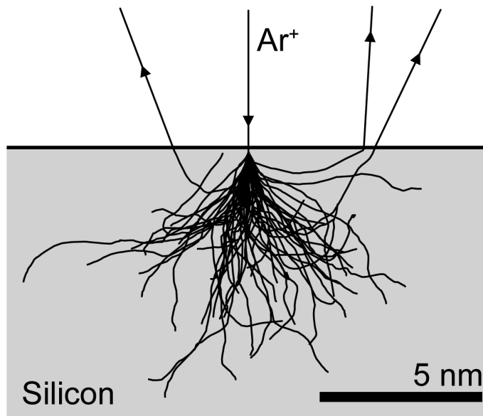
Fig. 2.2 Implant path of 60 argon ions with energy of 2000 eV impinging on silicon.
