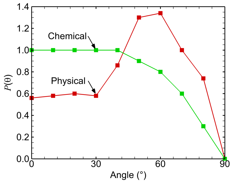
Fig. 2.5 Angular dependence functions, P(\theta) , for chemical and physical sputtering processes.
