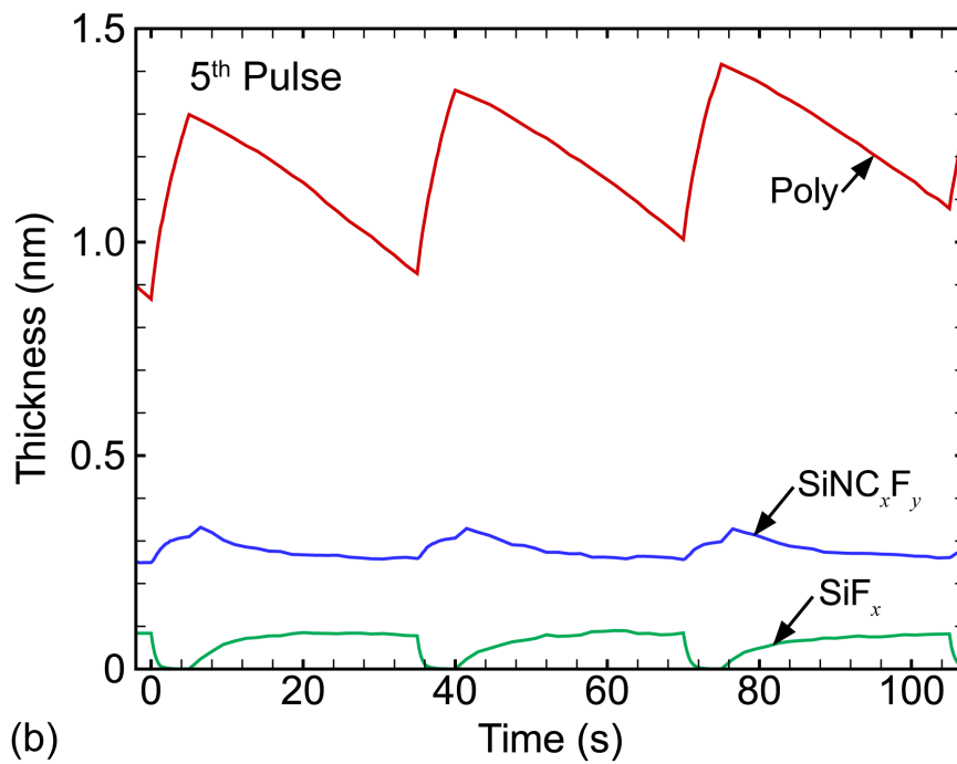
Fig. 7.6 Thickness of each overlayer species as a function of time during three ALE pulses ( t = 0 is the start of the 5 th pulse) for (a) \text{SiO}_2 and (b) \text{Si}_3\text{N}_4 .
