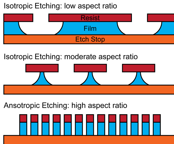
Fig. 1.1 Comparison of isotropic and anisotropic etching. Low aspect ratio features can be etched adequately by isotropic etching, while high aspect ratio features require an anisotropic etch profile.
