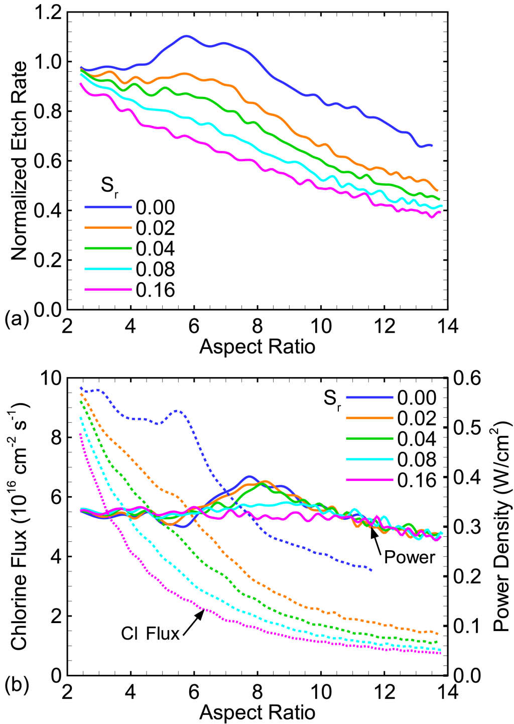
Fig. 4.13 Dependence of (a) etch rate, and (b) chlorine flux and power density on aspect ratio and the probability of recombination of radical chlorine on the walls, S_r . (a) Etch rates are normalized to the etch rate in the open field for the base case ( S_r = 0.08 ). Power density and chlorine flux are measured at the etch front as it evolves.
