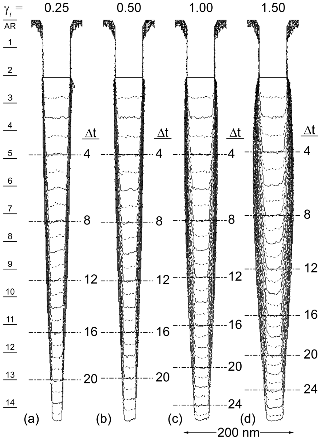
Fig. 4.16 Time evolution of silicon trench profile for different ion angular distributions, \gamma_i . The normalized angular distribution scaling factors shown are (a) 0.25, (b) 0.50, (c) 1.00, and (d) 1.50. Line spacing represents a constant time interval \Delta t for all profiles. Numbered lines represent similar etch times in each profile.
