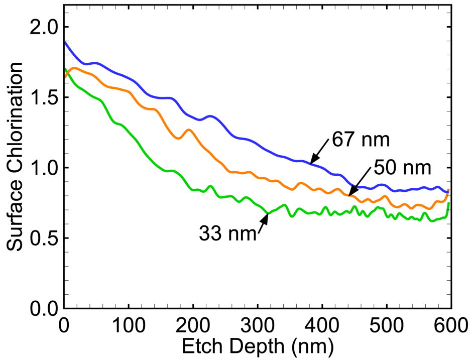
Fig. 4.7 Average surface chlorination (Cl atoms per silicon site) of the etch front as a function of etch depth for trenches having widths of 33, 50 and 67 nm.
