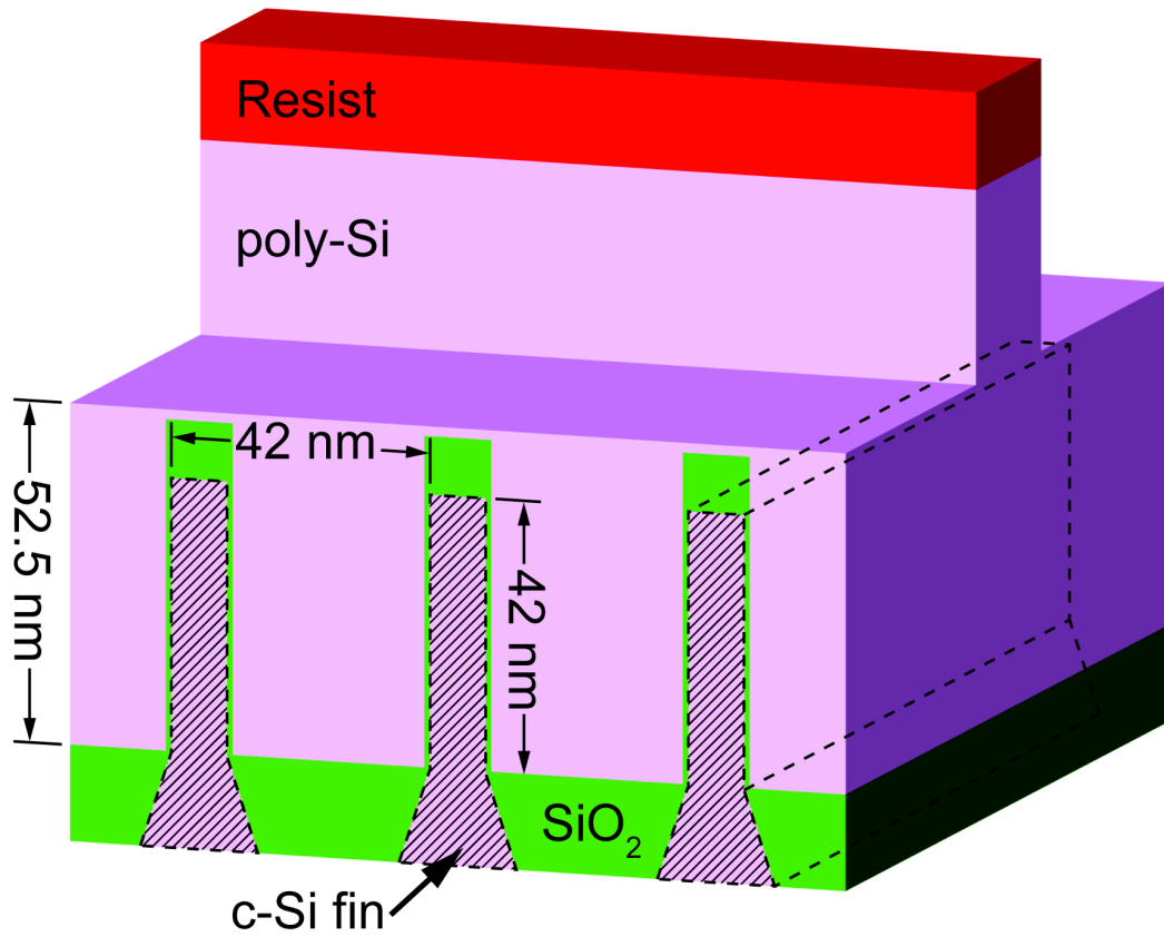
Fig. 5.14 Initial geometry used for the gate etch case study. The crystalline silicon (c-Si) fin travels back into the page, as indicated by the dotted lines. The resist (red) masks the poly-silicon gate structure, which is pre-etched to a depth just above the top of the fins.
