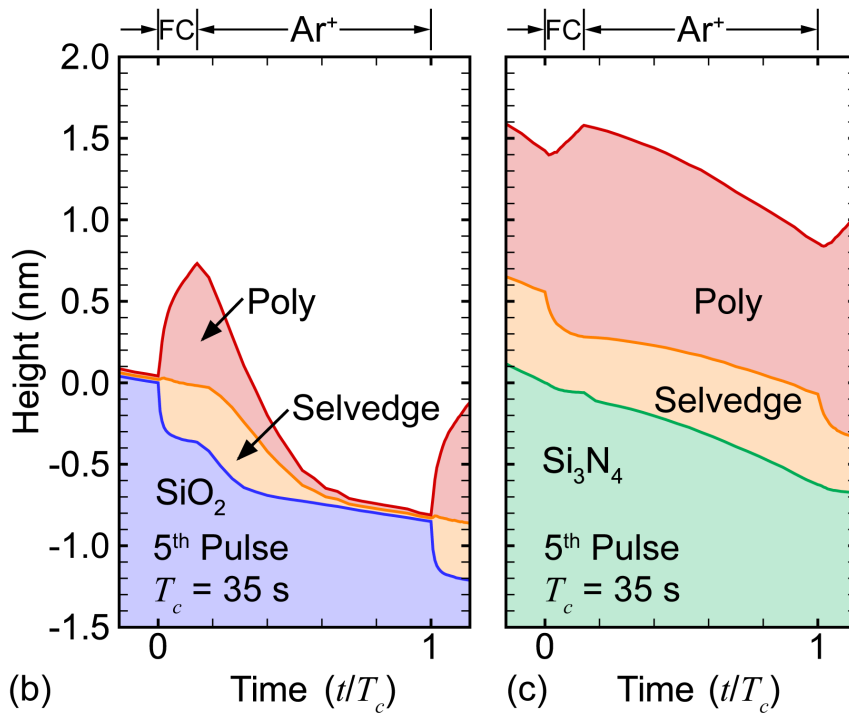
Fig. 7.5 ALE of \text{SiO}_2 and \text{Si}_3\text{N}_4 using non-ideal fluxes. (a) Change in total height (including polymer) as a function of time for \text{SiO}_2 and \text{Si}_3\text{N}_4 . The shaded regions represent the overlayer thickness, comprised of both the selvedge and polymer layers. Height of individual material layers during the 5 th ALE pulse for (b) \text{SiO}_2 and (c) \text{Si}_3\text{N}_4 .
