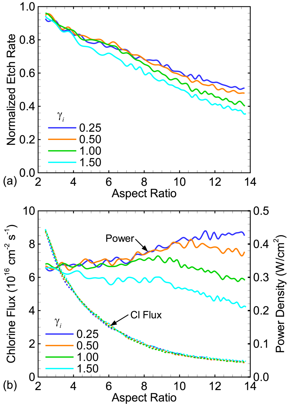
Fig. 4.17 Dependence of (a) etch rate, and (b) chlorine flux and power density on aspect ratio and the angular distribution of ions, \gamma_i . Etch rates are normalized to the etch rate in the open field for the base case ( \gamma_i = 1.00 ). Power density and chlorine flux are taken at the etch front as it evolves.
