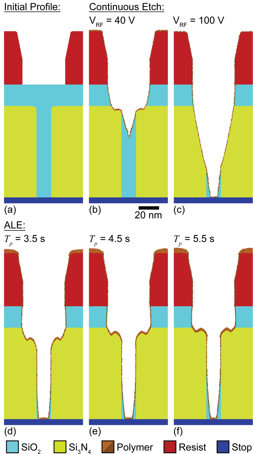
Fig. 7.9 Self-aligned-contact etch profiles for continuous etching and ALE. (a) Initial profile. Continuous etch using the FC gas mixture with 1200 W ICP power for (b) V_{RF} = 40 \text{ V} and (c) V_{RF} = 100 \text{ V} . ALE profiles after 165 cycles using T_i = 20 \text{ s} and T_p = (d) 3.5 s, (e) 4.5 s and (f) 5.5 s.
