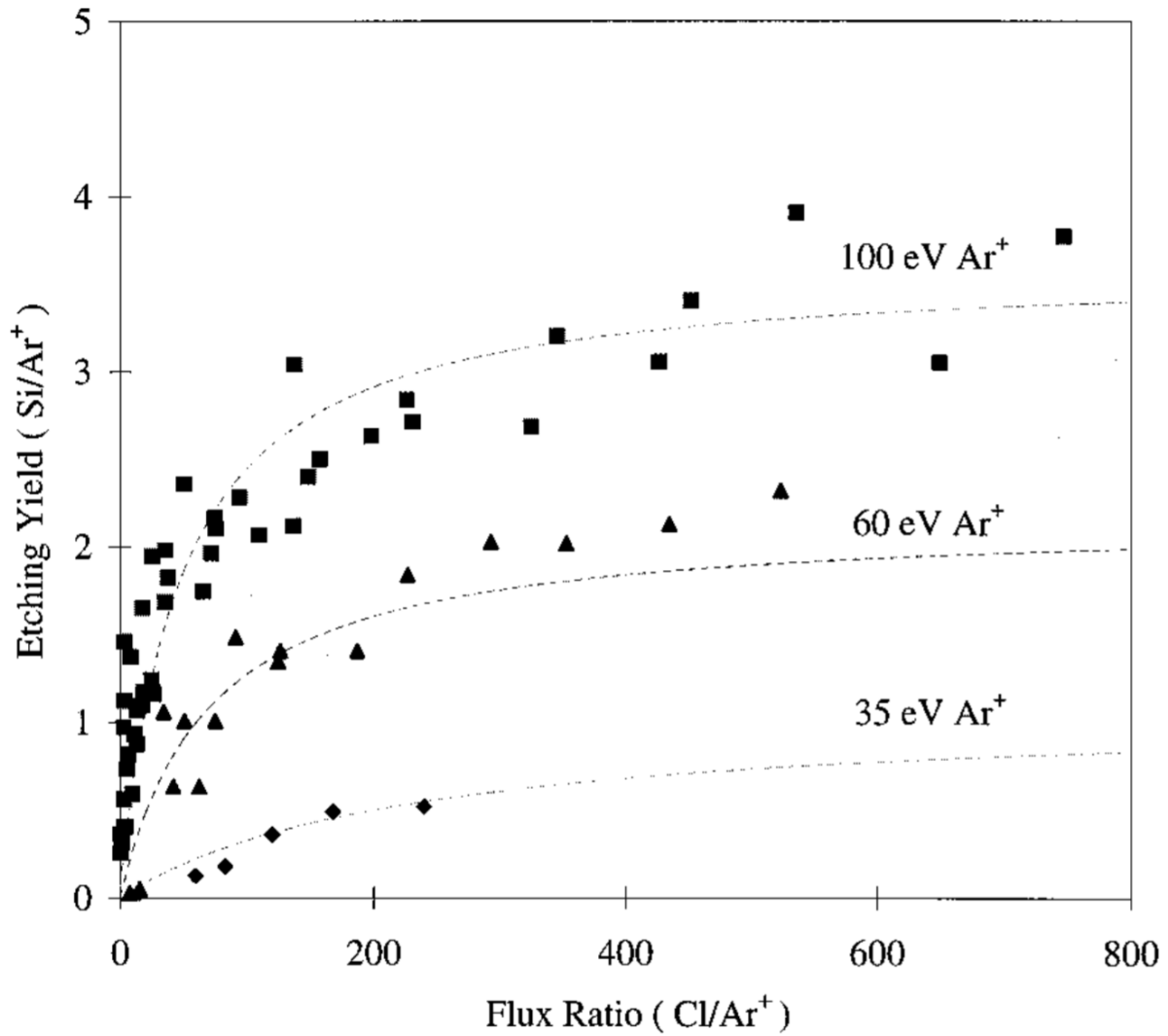
Fig. 1.10 Etch yield per Ar + ion as a function of \Gamma_n/\Gamma_i (Cl/Ar + ). The etching yield increases rapidly for low \Gamma_n/\Gamma_i and saturates when the reaction becomes ion starved. Reproduced from Chang et al.[22]
