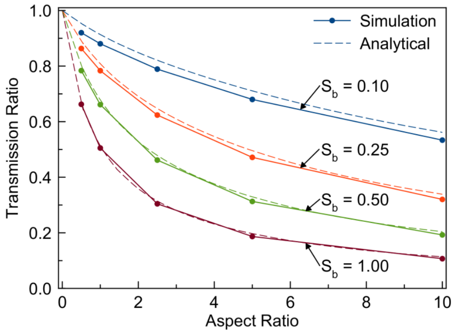
Fig. 2.7 Neutral transport simulation in MCFPM for cylindrical tubes with sticking coefficients S_b on the bottom surface. Transmission ratio is the flux of particles at the bottom of the tube, divided by the flux of particles entering the feature.
