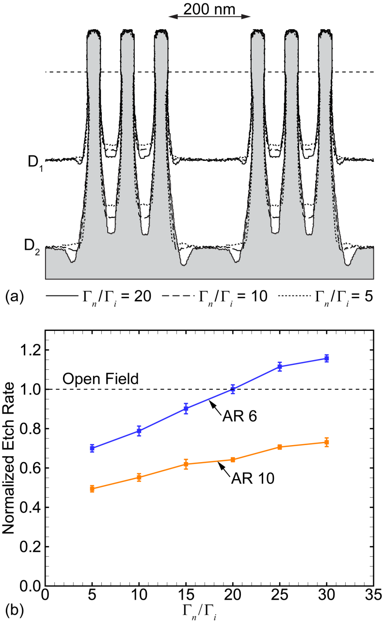
Fig. 4.8 Etch properties for different values of \Gamma_n/\Gamma_i . (a) Two dimensional slice through FinFET profile for several incoming neutral to ion flux ratios. The lines labeled D_1 and D_2 represent equal etch depths, and are taken at different etch times due to the different etch rates between cases. The slice is taken through the center of the length of the fin. (b) Normalized etch rates as a function of \Gamma_n/\Gamma_i for two different AR. Etch rates are normalized to the initial etch rate of each respective \Gamma_n/\Gamma_i to enable comparison.
