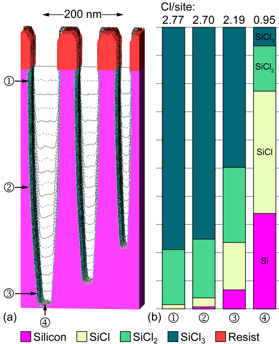
Fig. 4.6 Etch properties for trenches. (a) Simultaneously etched profiles showing ARDE for three trenches having different widths. Colors represent different solid materials. Black lines represent slices through the center of the trench at different times, taken at constant time intervals. (b) Normalized density of surface species at different locations along the 67 nm profile. The etch front measurement is taken on the horizontal surface being bombarded by ions. Side high, mid and low measurements are taken from the side wall just below the resist, halfway down the profile and just above the etch-front. All chlorination measurements were taken at the final time step.
