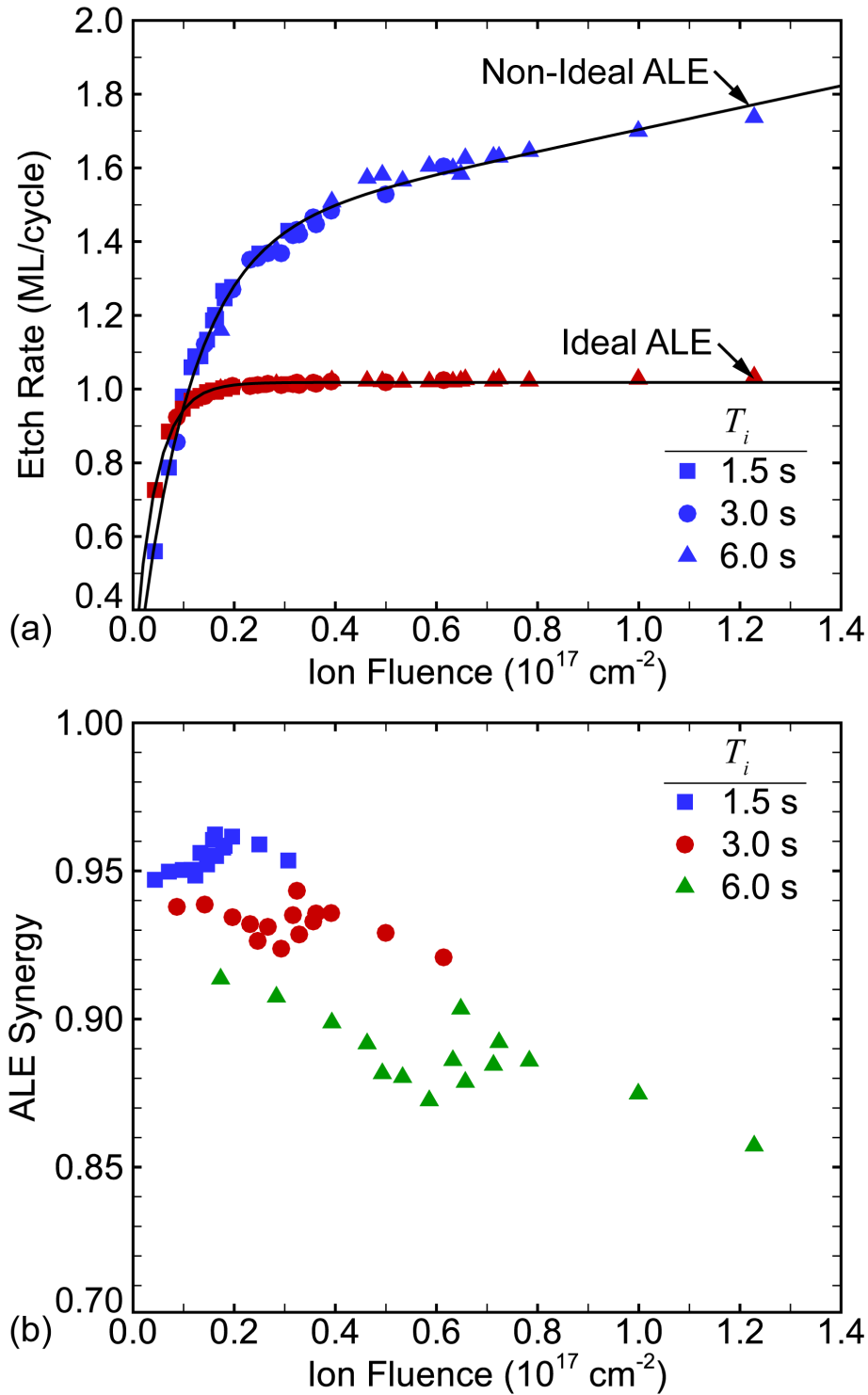
Fig. 6.4 Data points from three ion bombardment times T_i are shown using different symbols (squares: T_i = 1.5 \text{ s} ; circles: T_i = 3 \text{ s} ; triangles: T_i = 6 \text{ s} ). For each T_i , data from all three antenna configurations is shown without differentiation. (a) Etch rate. (b) ALE synergy \mathcal{S}_y .
