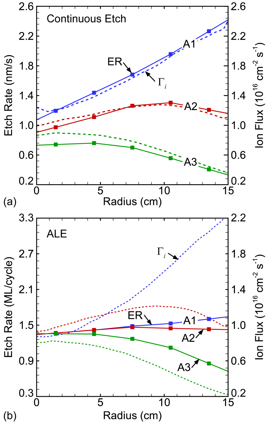
Fig. 6.2 Etch rate and ion flux to the wafer as a function radius for three antennas, A1, A2 and A3. (a) Continuous etching ( \text{Ar}/\text{Cl}_2 = 90/10 ) with etch rate in nm/s. (b) Ion fluxes from argon plasma with 10 ppm \text{Cl}_2 contamination with ALE rate in ML/cycle.
