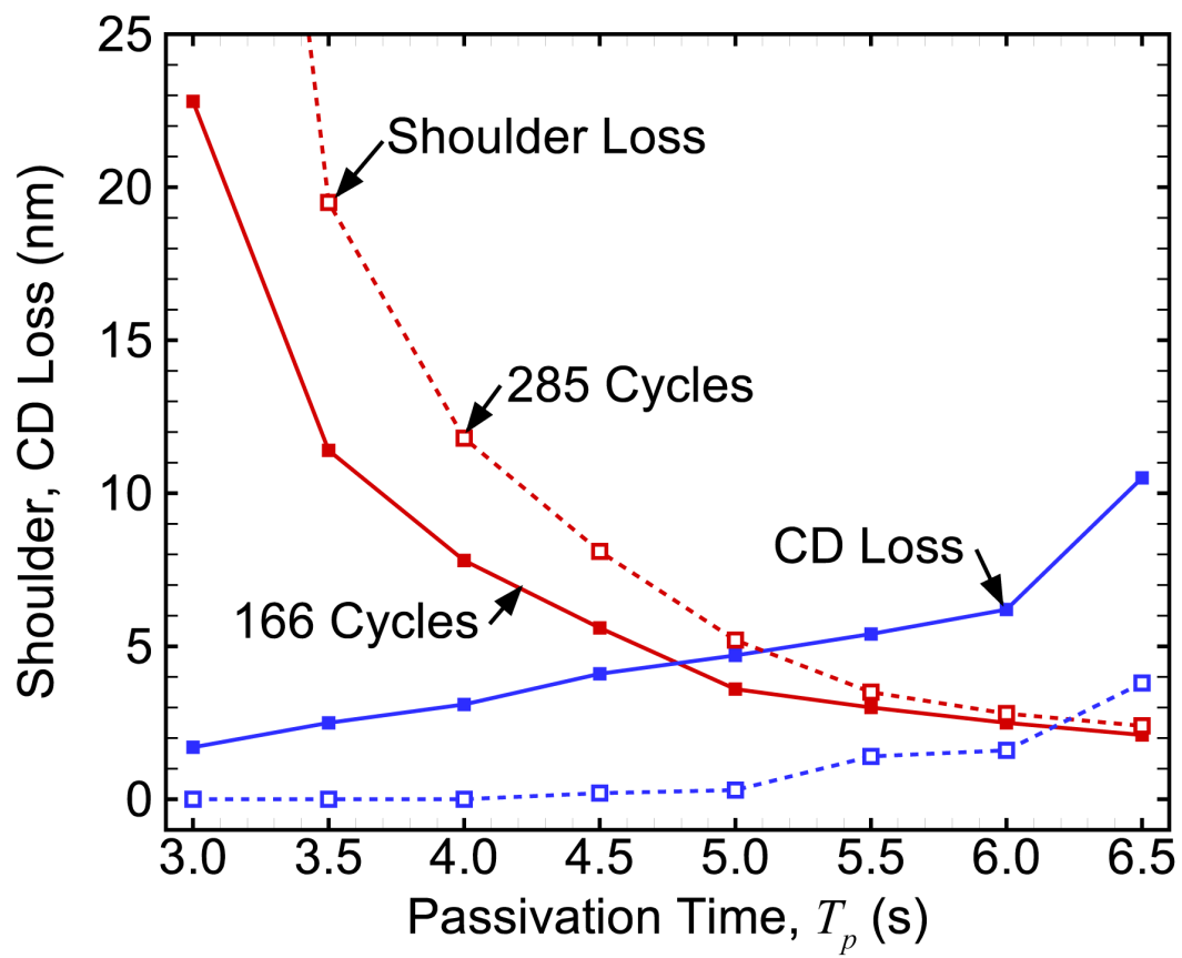
Fig. 7.10 Shoulder loss and CD loss as a function of passivation time for the SAC feature with T_i = 20 s.
