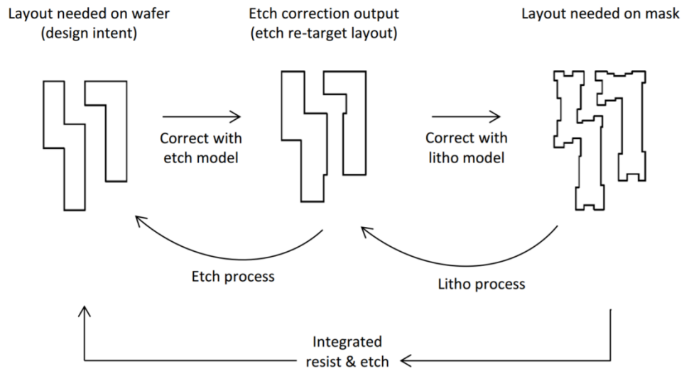
Fig. 1.14 Schematic of incorporating the etch model into the mask design phase. Using the etch model in this way may enable the correction of etch imperfections which cannot otherwise be resolved. Reproduced from Zavyalova et al.[64]
