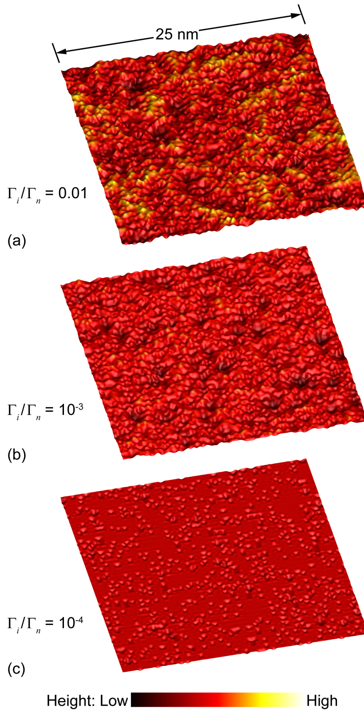
Fig. 5.6 Surface morphology of the trench bottom for \Gamma_i/\Gamma_n = (a) 0.01, (b) 10^{-3} and (c) 10^{-4} in the passivation step after 25 pulses (87.5 s etch time). Color represents the profile height, with black being deeper etching, red representing the average etch depth and yellow/white being higher features.
