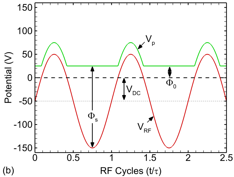
Fig. 1.3 Schematic example of the effect of applying a RF bias to a wafer in a (a) symmetric and (b) asymmetric reactors.
