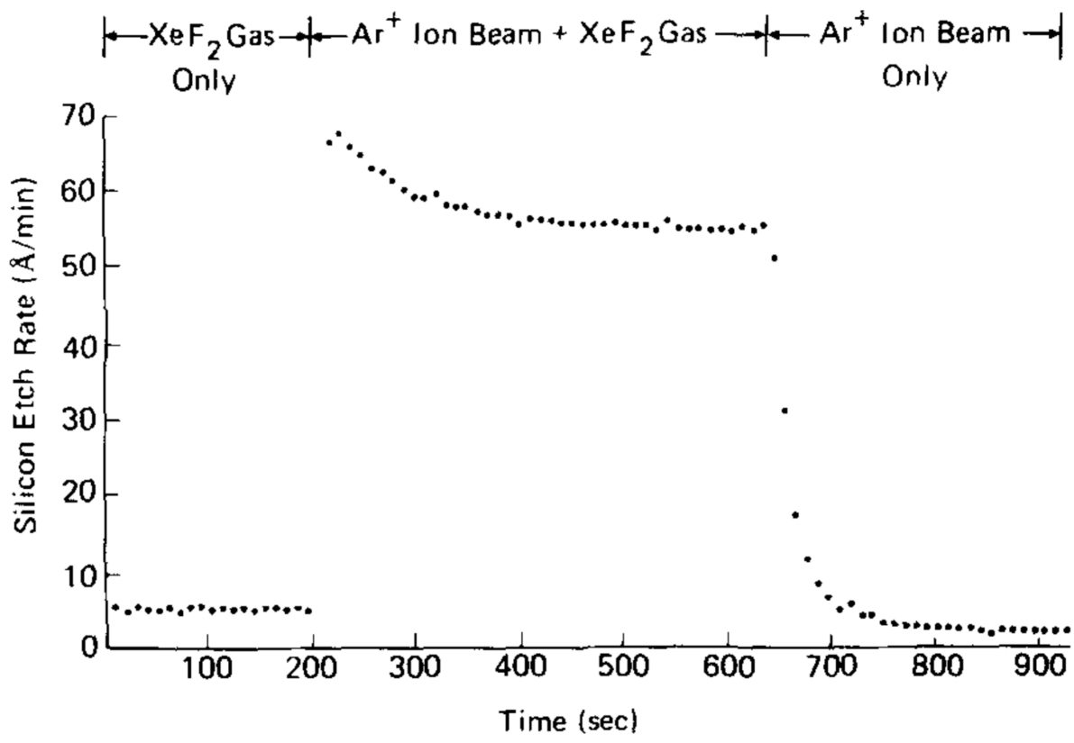
Fig. 1.9 Etch rate of silicon exposed to XeF 2 only, XeF 2 /Ar + and Ar + only. The dramatic increase in etch rate when XeF 2 is combined with Ar + exposure is due to the reduced surface binding energy of fluorinated silicon. Reproduced from Coburn and Winters.[21]
