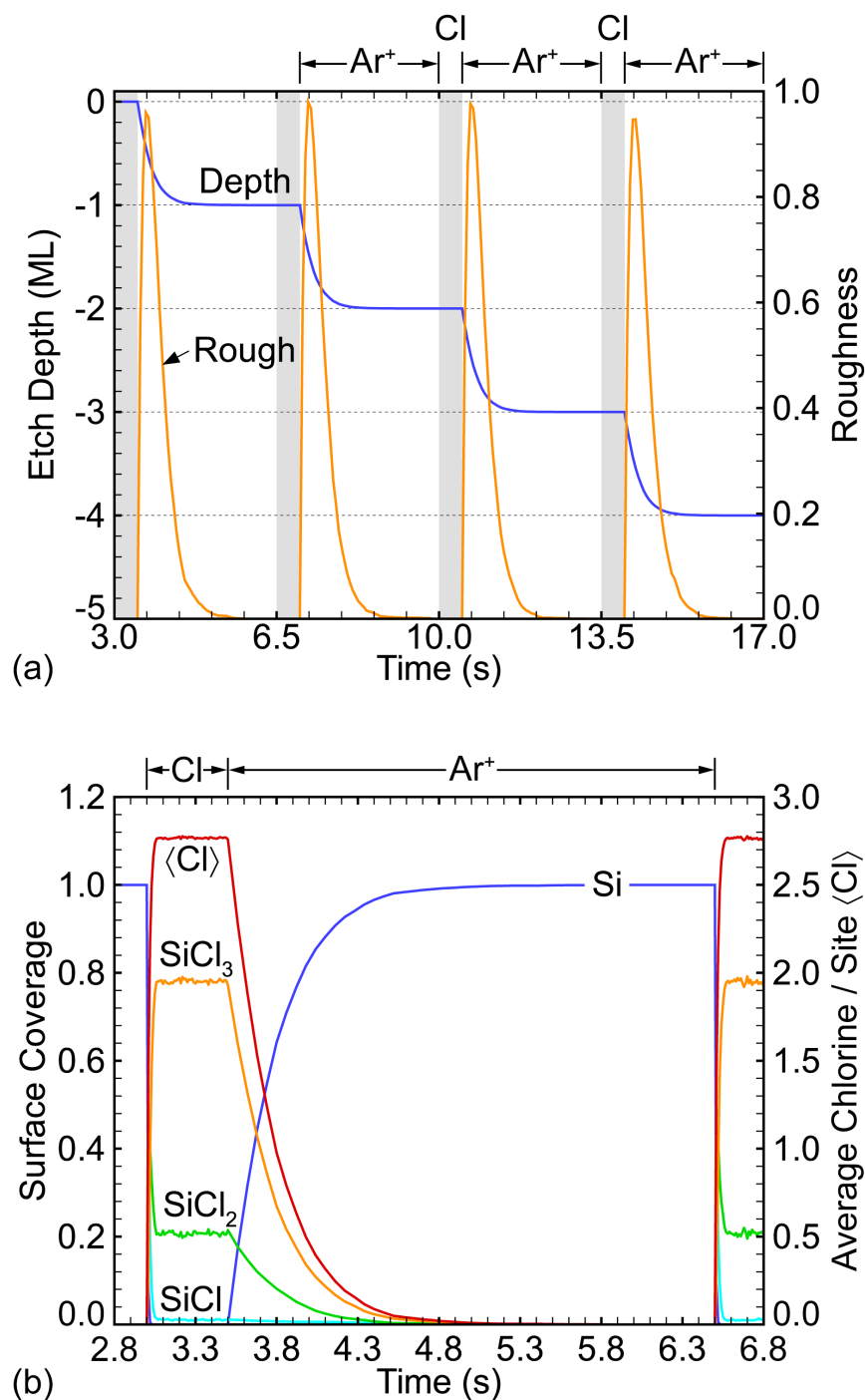
Fig. 5.2 Etch front characteristics during ideal ALE etching. (a) Etch depth and surface roughness as a function of time for the second through fifth ALE pulses. The different sub-cycles (Cl = passivation, Ar + = ion bombardment) are shown at the top for reference, with passivation phases being highlighted by grey bands in the figure. Four pulse periods are shown in total. (b) Surface coverage of Si, SiCl, SiCl 2 , SiCl 3 and average chlorine per site at the etch front as a function of time for the second pulse.
