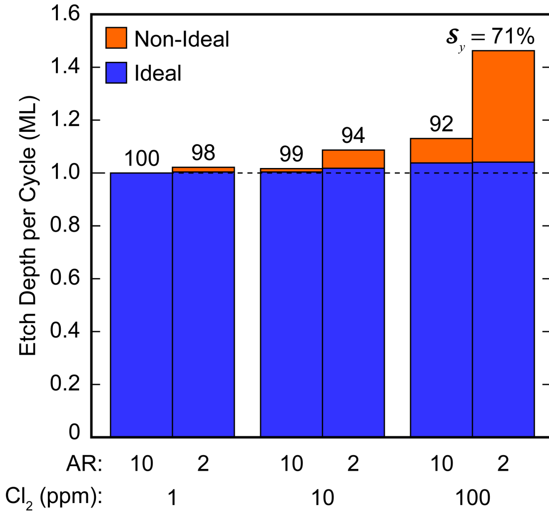
Fig. 5.7 Etch depth per cycle due to ideal (reactions which occur through ALE synergy) and non-ideal (continuous) etching for cases with 1, 10 and 100 ppm Cl 2 in the ion bombardment step, for both AR = 2 and 10 trenches. The dotted line represents ideal ALE, with an etch depth per cycle of 1 ML.
