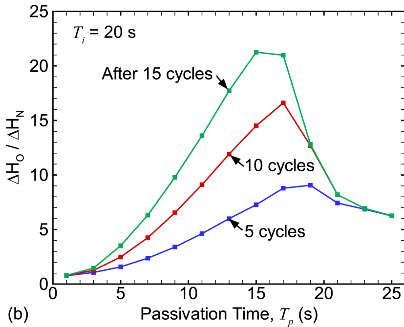
Fig. 7.8 Selectivity of ALE of \text{SiO}_2 over \text{Si}_3\text{N}_4 . (a) Selectivity after 15 cycles as a function of passivation time ( T_p ) for ion bombardment times ( T_i ) of 10, 20 and 30 s. (b) Selectivity as a function of T_p for three different etch durations (5, 10 and 15 cycles) using T_i = 20 s.
