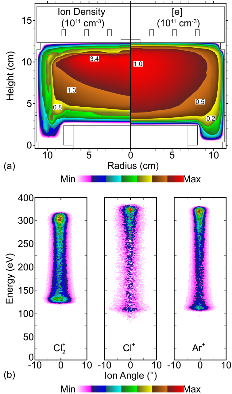
Fig. 4.1 Reactor and plasma properties. (a) Reactor geometry with (left) total positive ion density and (right) electron density, shown on a log scale with a range of two decades. (b) Probability density of ions reaching the wafer surface as a function of ion energy and incident angle (IEAD), shown on a linear scale.
