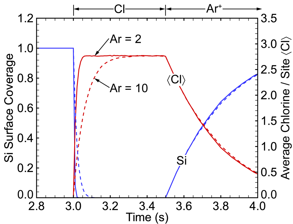
Fig. 5.3 Surface coverage of Si and average chlorine per site at the etch front for ideal ALE as a function of time for the second ALE pulse for AR = 2 and 10 trenches.
