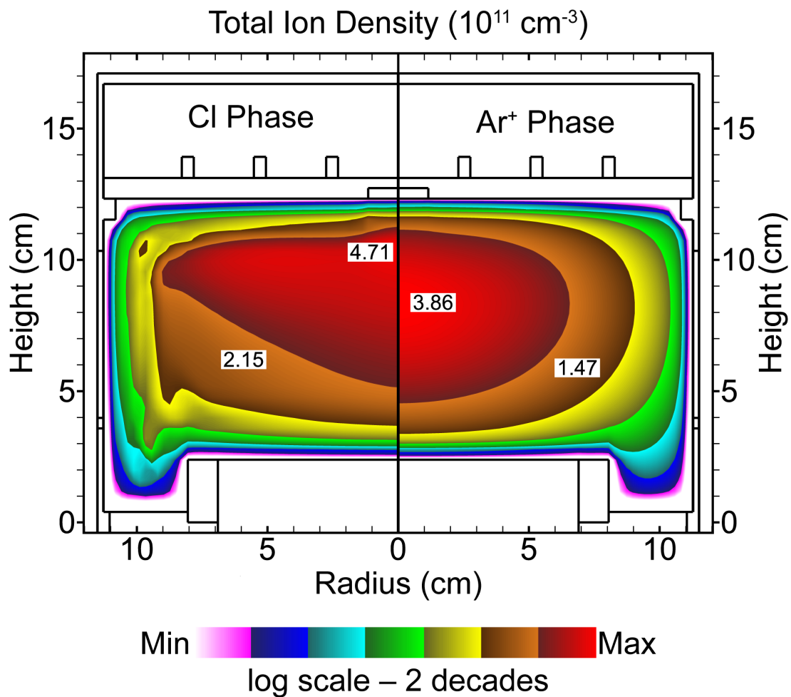
Fig. 5.10 Reactor geometry and total ion densities in the (left) Cl passivation phase and (right) Ar + ion bombardment phase. A log scale showing two decades is used.
