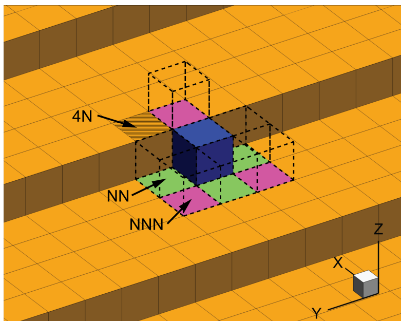
Fig. 2.4 Illustration of possible diffusion locations for a physisorbed particle, shown in blue. The dotted cubes illustrate the allowable diffusion transitions. Nearest neighbor sites are shown in green, next-nearest neighbors in purple, and a next-next-nearest neighbor as hatched. The 4N site is not an allowable direct transition from the current site.
