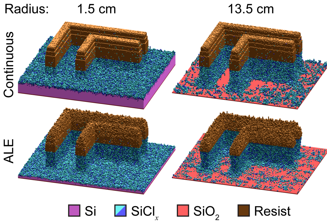
Fig. 6.5 Predicted etch profiles for using antenna A1 for (top) continuous etching and (bottom) ALE at radii of (left) 1.5 cm and (right) 13.5 cm. T_i = 3 s for ALE cases. The two radial positions are etched for the same time, representing the non-uniformity on the wafer just before clearing the feature at the wafer edge.
