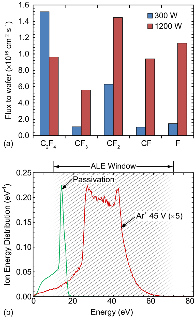
Fig. 7.1 Plasma conditions used in continuous and ALE processing. (a) Ratios of fluxes of \text{C}_4\text{F}_8 dissociation products incident onto the wafer for ICP powers of 300 W and 1200 W. (b) Ion energy distributions reaching the surface during the passivation (VRF = 0 V) and ion bombardment (VRF = 45 V) phases.
