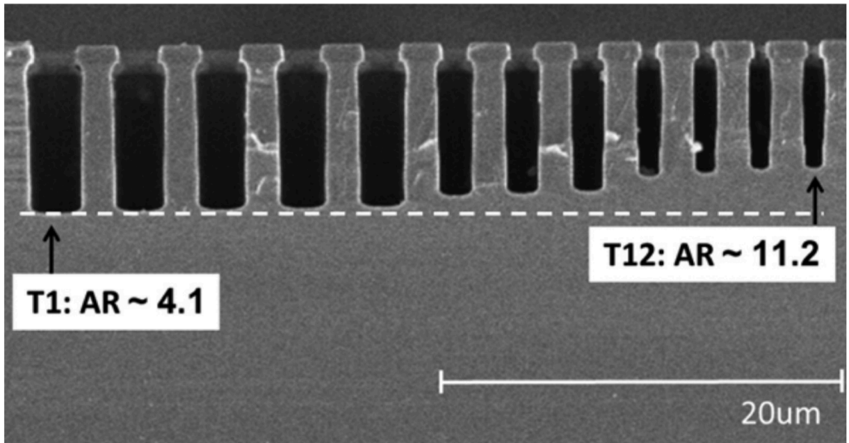
Fig. 1.12 Features with different critical dimensions etched simultaneously. Notice larger features etch faster than smaller ones. Reproduced from Bates et al.[37]
