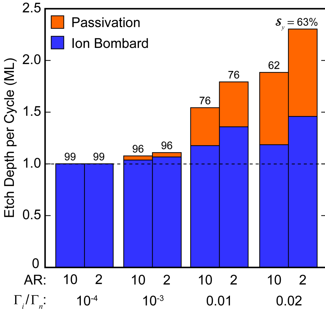
Fig. 5.4 Etch depth per cycle in the passivation and ion bombardment phase for values of \Gamma_i/\Gamma_n = 0.02, 0.01, 10^{-3} and 10^{-4} in the passivation step, for both AR = 2 and 10 trenches. The dotted line represents ideal ALE, with an etch depth per cycle of 1 ML.
