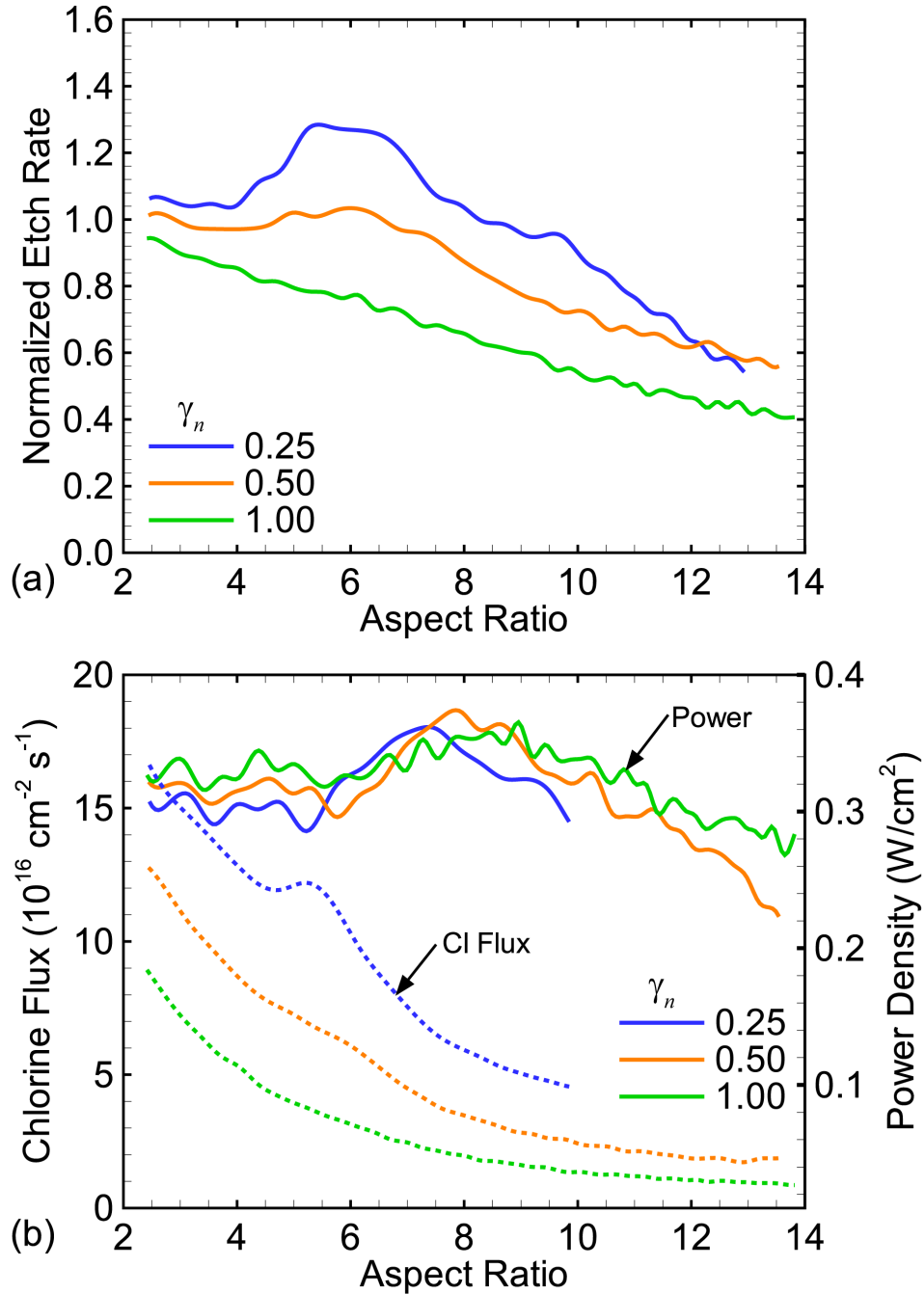
Fig. 4.15 Dependence of (a) etch rate, and (b) chlorine flux and power density on aspect ratio and the angular distribution of neutrals, \gamma_n . Etch rate is normalized to the etch rate in the open field for the base case ( \gamma_n = 1.00 ). Power density and chlorine flux are measured at the etch front as it evolves. Chlorine flux and power density are omitted above an AR of 10 for \gamma_n = 0.25 due to the highly tapered profile interfering with the measurement technique.
