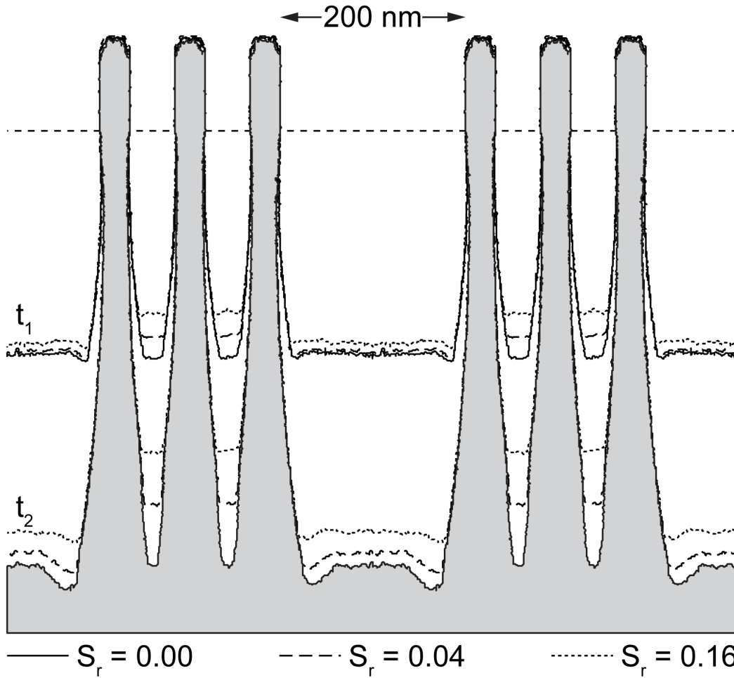
Fig. 4.11 Two dimensional slice through fin profile for several surface recombination probabilities, S_r . The lines labeled t_1 and t_2 represent equal etch times. The slice is taken through the center of the length of the fin.
