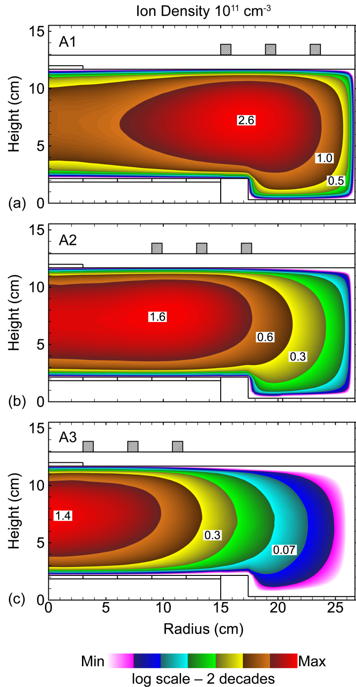
Fig. 6.1 Reactor geometry and total ion density for three different antenna configurations. Antennas, from top to bottom are: (a) A1, (b) A2 and (c) A3. The ion densities are for the argon plasma used in ion bombardment during ALE – \text{Ar}/\text{Cl}_2 = 100/10 ppm, 10 mTorr. Powers were adjusted to provide the same ion flux to the center of the wafer.
