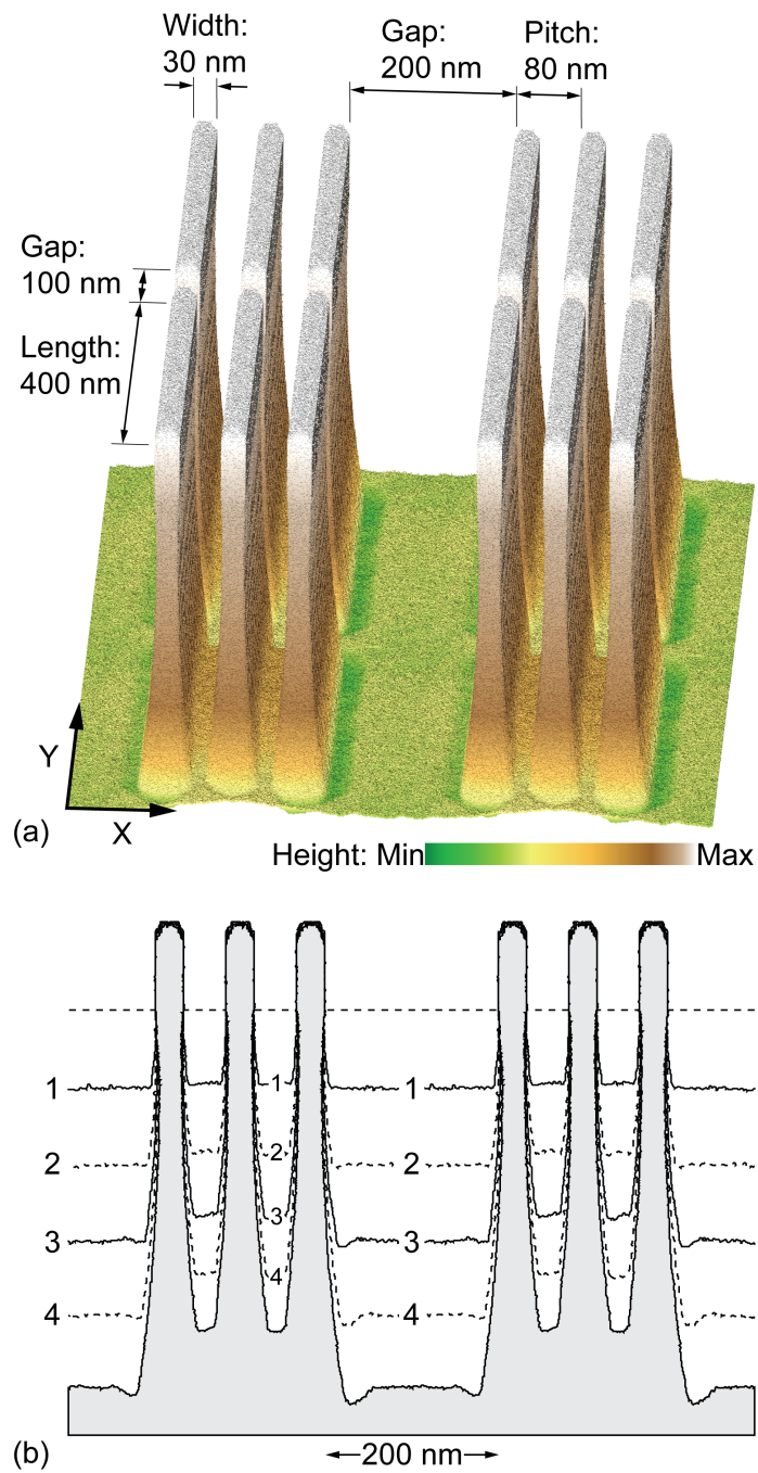
Fig. 4.3 Etched profiles for the FinFET geometry. (a) Color represents height of feature, showing the variation of etch depth in the longitudinal Y-direction between fins. The difference between the total etch depth between the fins and the open field is also visible. (b) Slice through the fins in the X-direction, taken at the center of the fin length. Each line is separated by a constant time interval.
