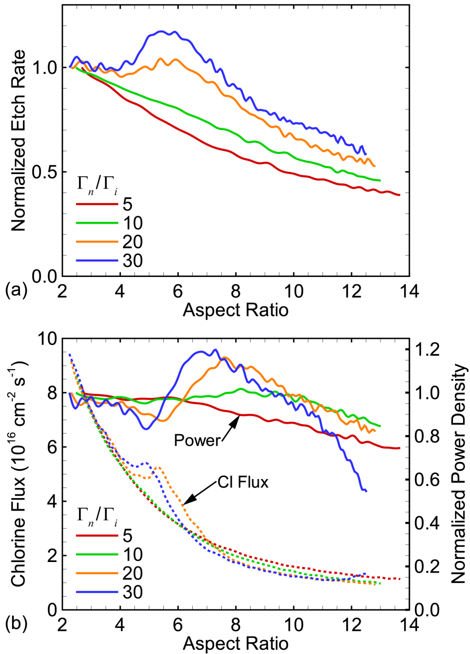
Fig. 4.10 Dependence of etch rate, chlorine flux and power density on aspect ratio and the \Gamma_n/\Gamma_i ratio. Lines are labeled with neutral to ion ratios \Gamma_n/\Gamma_i=5, 10, 20 and 30 . (a) Etch rates normalized to the initial etch rate of each \Gamma_n/\Gamma_i . (b) Power densities (solid) and Cl flux (dotted) are measured in a small window centered in the etch front. Power density is normalized to the initial power density of each respective \Gamma_n/\Gamma_i ratio.
