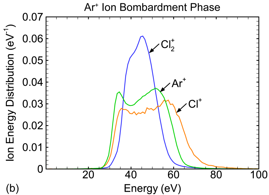
Fig. 5.11 Ion energy distribution for \text{Cl}^+ , \text{Cl}_2^+ and \text{Ar}^+ in the (a) passivation and (b) ion bombardment phases. Each ion energy distribution is a probability density function for that ion, and is normalized such that integrating the function in energy results in a value of 1 regardless of the total flux of that ion.
