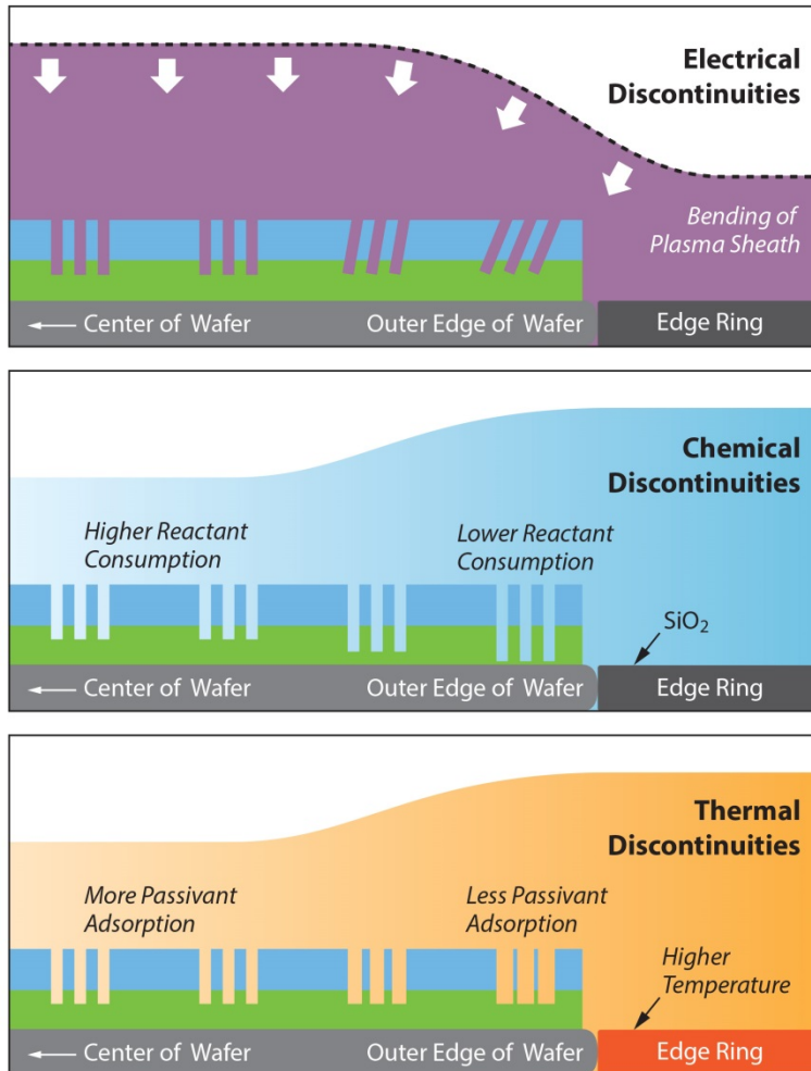
Fig. 1.13 Sources of wafer scale non-uniformity. Reproduced from Hwang and Kanarik.[37]
