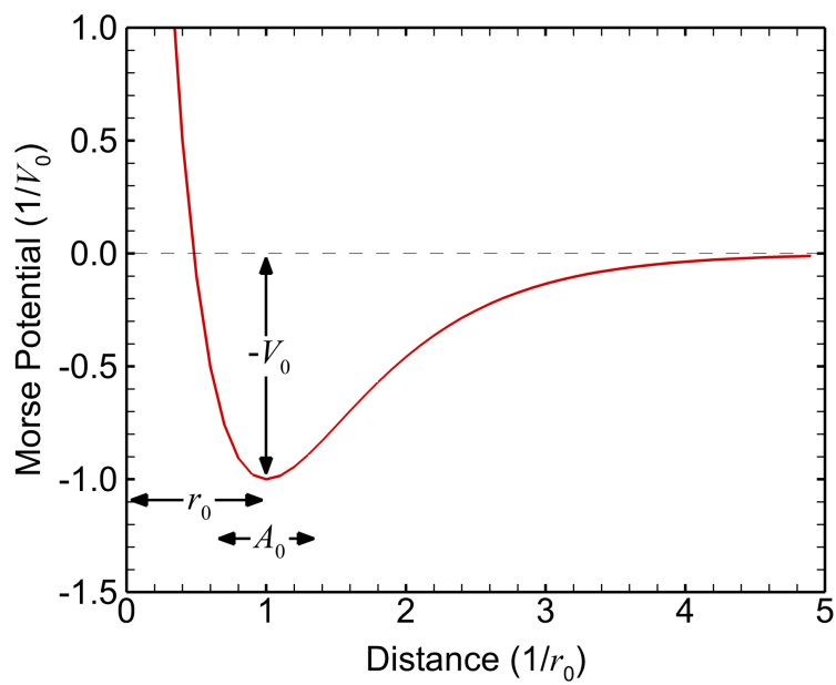
Fig. 2.3 The Morse potential used for the diffusion routine. The distance between cells r is normalized to r_0 and the potential is normalized to V_0 . The A_0 used for this potential is 0.75.
