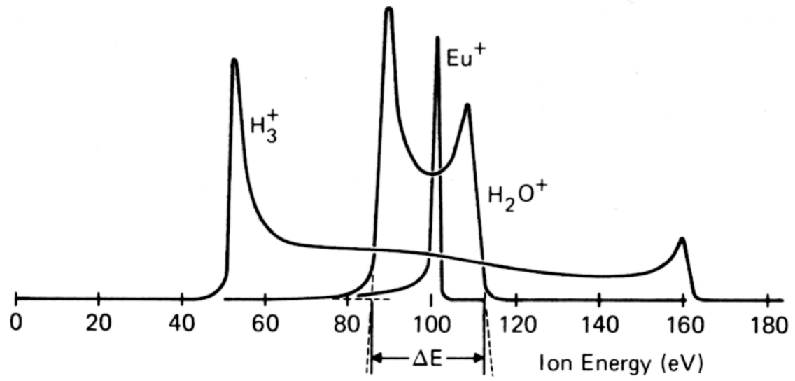
Fig. 1.6 Ion energy distribution for several ions with different masses. Reproduced from Coburn and Kay.[12]
