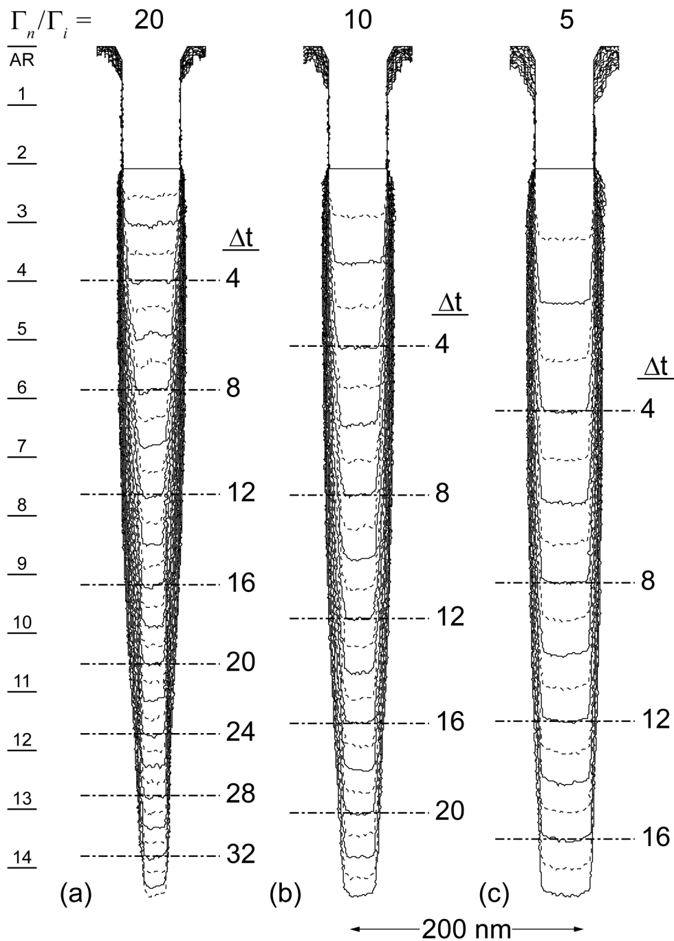
Fig. 4.9 Time evolution of silicon trench profile during Ar/Cl 2 etching for different neutral to ion ratios. The neutral to ion ratios are (a) 20, (b) 10 and (c) 5. Line spacing represents a constant time interval for all profiles. Numbered lines represent similar etch times in each profile.
