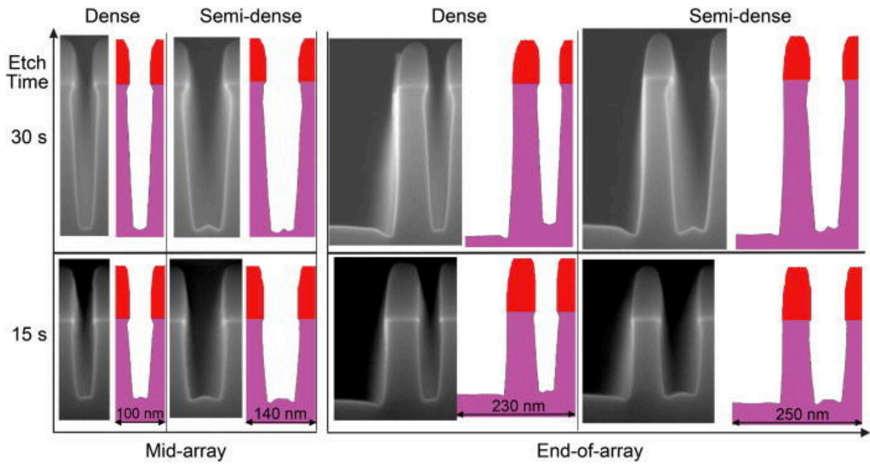
Fig. 2.8 MCFPM validation cases using He/Cl 2 plasma etching. Notice the close match of profile geometry in dense, semi-dense and end of array features at two different etch times.[84]
