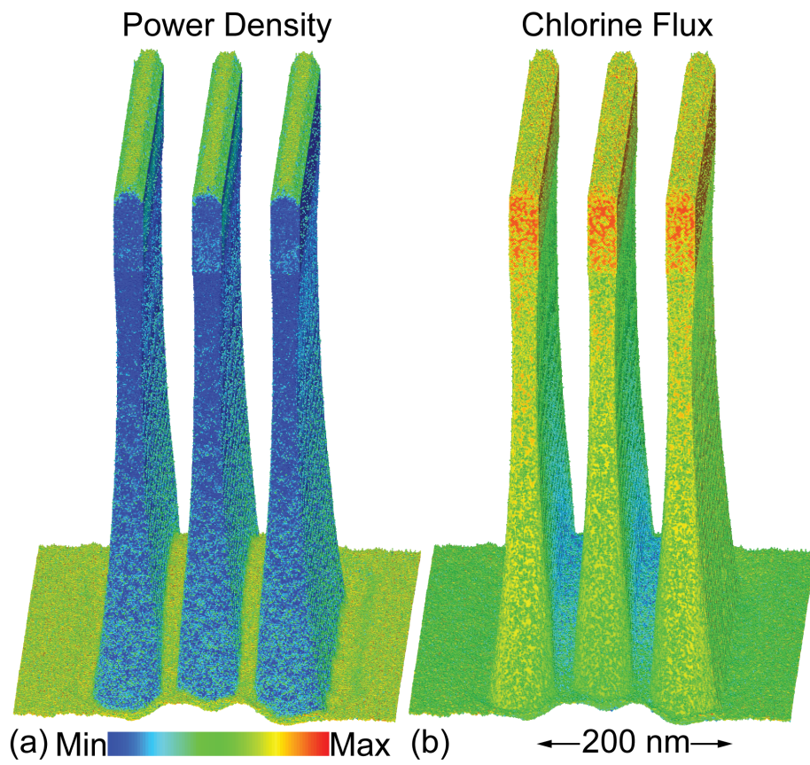
Fig. 4.4 Spatially resolved fluxes to the surface of the etch profile. (a) Power density delivered by ions and (b) chlorine radical flux.
