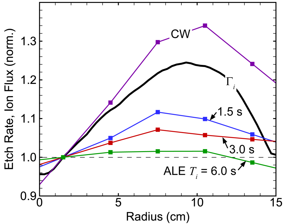
Fig. 6.3 Etch rate and ion flux normalized to their values at a radius of 1.5 cm for different ion bombardment times ( T_i = 1.5, 3.0 and 6.0 s) for antenna A2. “CW” indicates the continuous etching rate.
