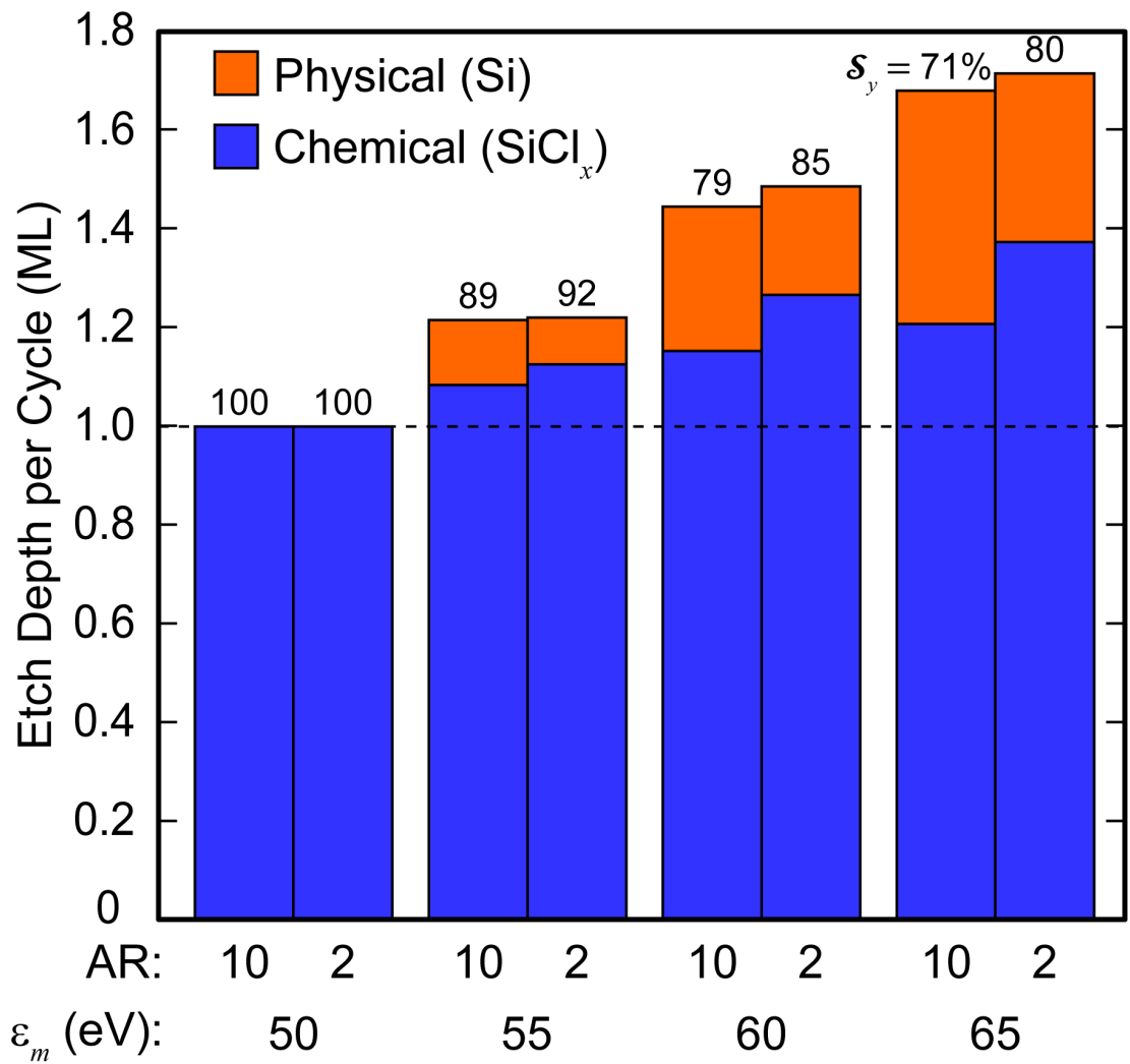
Fig. 5.9 Etch depth per cycle for physical and chemical sputtering processes for values of \epsilon_m = 50, 55, 60 and 65 in the ion bombard step, for both AR = 2 and 10 trenches. The dotted line represents ideal ALE, with an etch depth per cycle of 1 ML.
