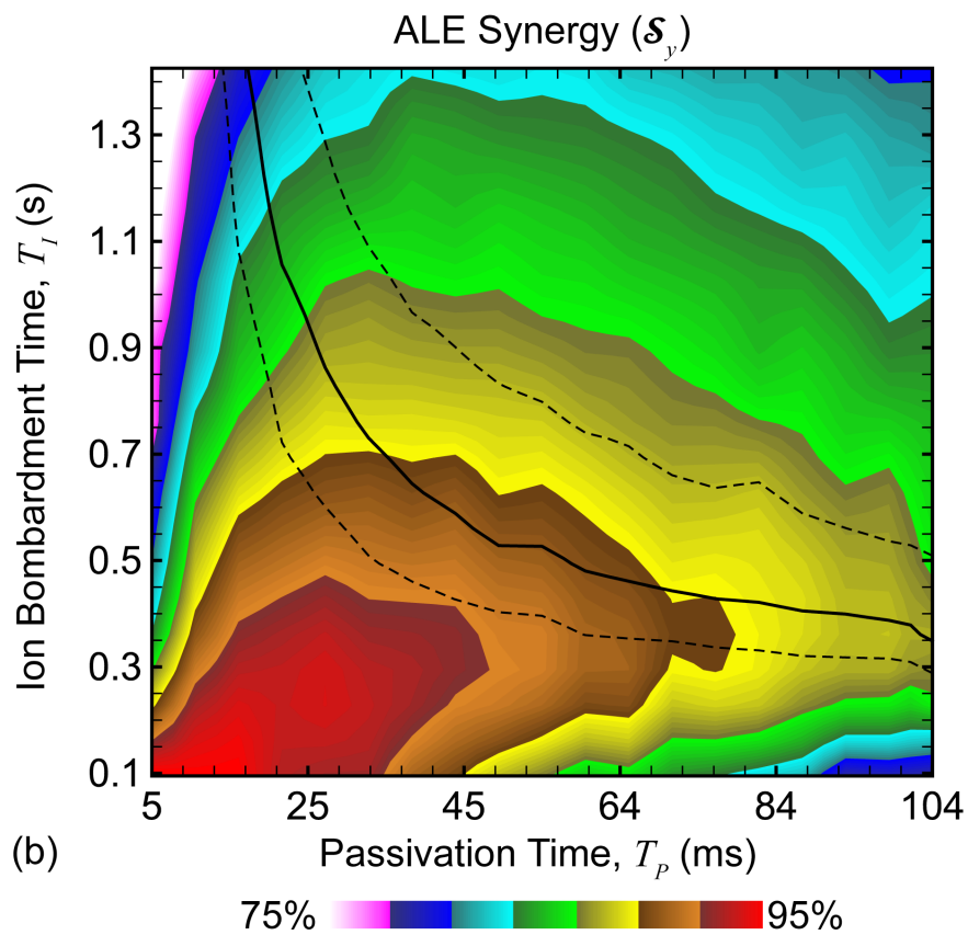
Fig. 5.13 Trends in the ALE synergy ( \mathcal{S}_y ) as a function of pulse times for an AR of 4. (a) \mathcal{S}_y as a function of ion bombardment time ( T_I ) for three values of passivation time ( T_p ). (b) \mathcal{S}_y as a function of T_I and T_p . The solid black line represents EPC = 1 and the dotted lines bound the range 0.9 < EPC < 1.1 .
