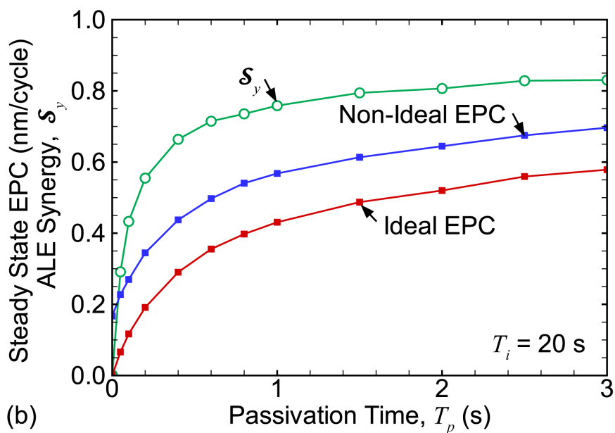
Fig. 7.4 Comparison of non-ideal and ideal \text{SiO}_2 ALE properties. (a) Pulse-periodic steady state etch per cycle (EPC) as a function of T_p , for T_i = 10, 20 and 30 s for ideal (dotted lines) and non-ideal (solid lines) reactive fluxes. (b) ALE synergy and steady state EPC for small values of T_p with T_i = 20 s. Values are shown for ideal and non-ideal fluxes.
