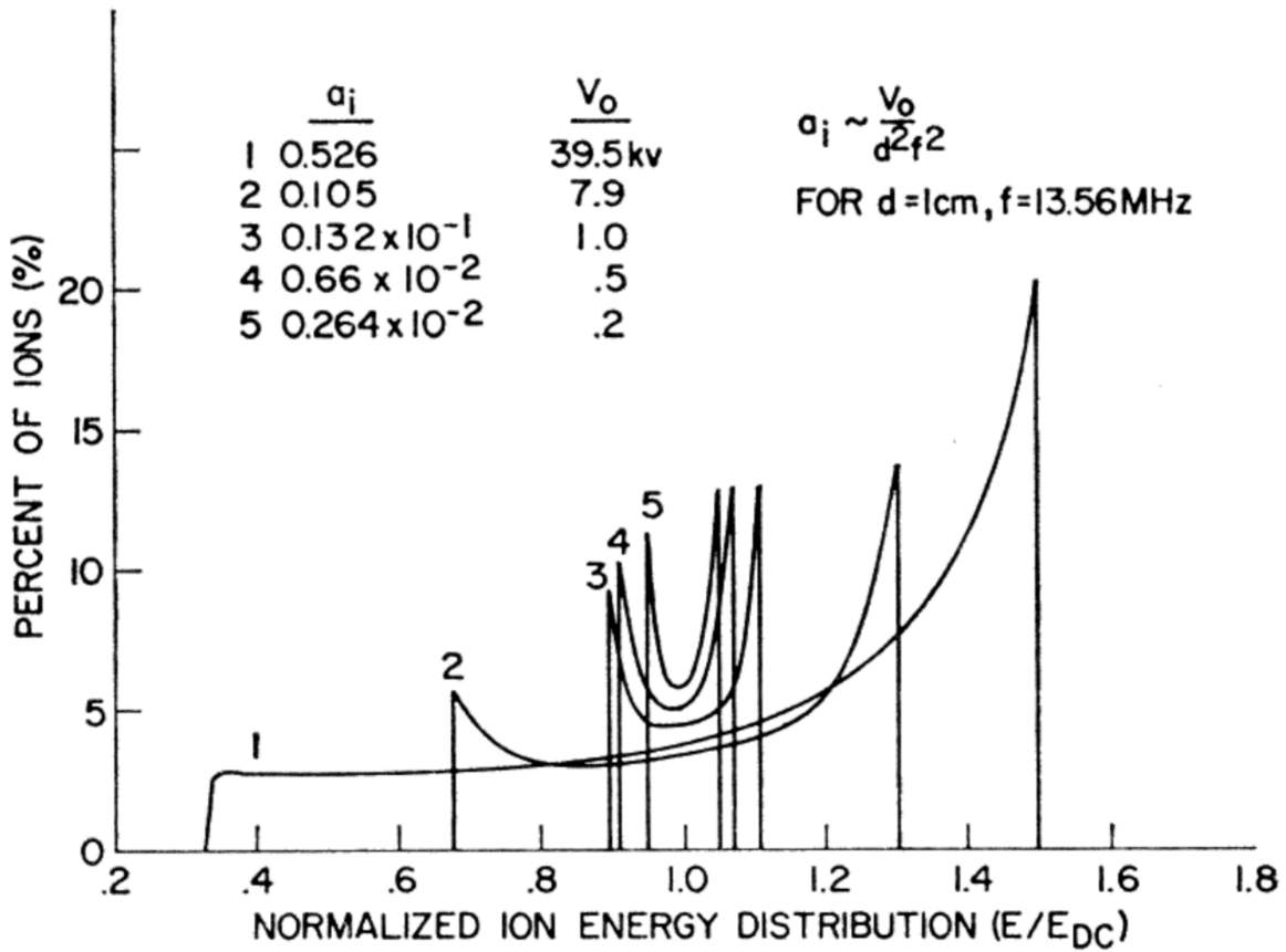
Fig. 1.4 Ion energy distributions for different values of \tau_{ion}/\tau_{rf} . The curve marked 1 is the lowest \tau_{ion}/\tau_{rf} and 5 is the highest. The lack of a low frequency peak is due to an assumption that the sheath width is constant, and is not typical of experiment. Reproduced from Tsui.[11]
