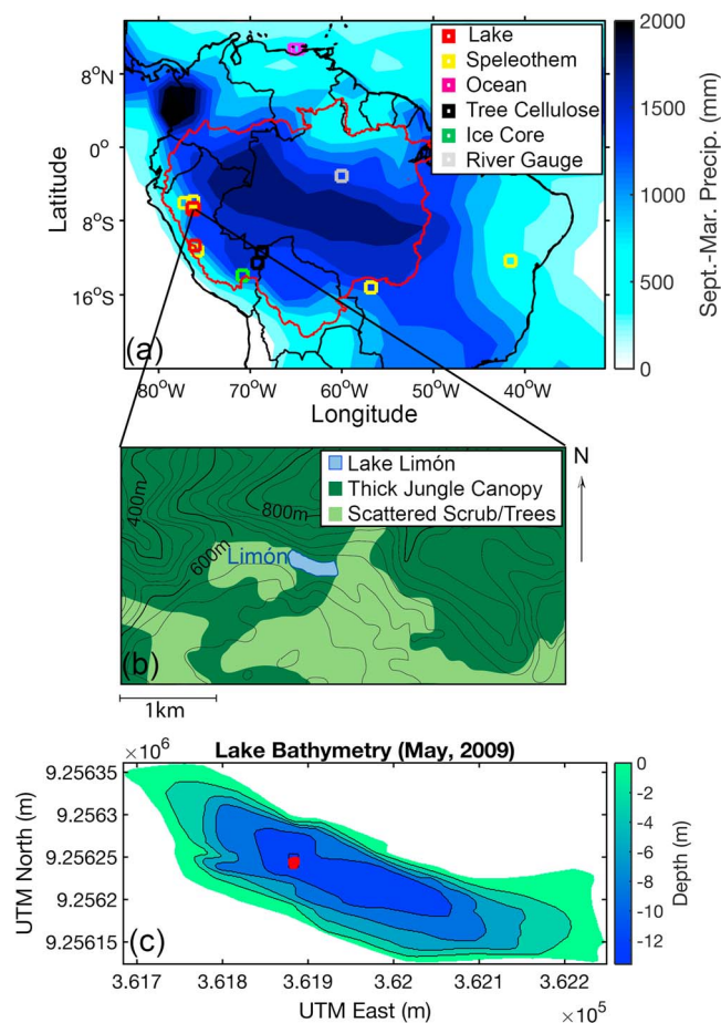
Figure 1. Maps showing regional climatology and paleoclimate record locations, local topography, and Lake Limón bathymetry. (a) Map of satellite-era September to March South American GPCP v2.3 precipitation (Adler et al., 2003) and paleoclimate record locations (citations and other record information in Table 1). Red line outlines Amazon River drainage basin and filled red square indicates Lake Limón location. (b) Contour map of basin around Lake Limón. (c) Bathymetric map (blue shading) of Lake Limón with red circles marking coring locations.
