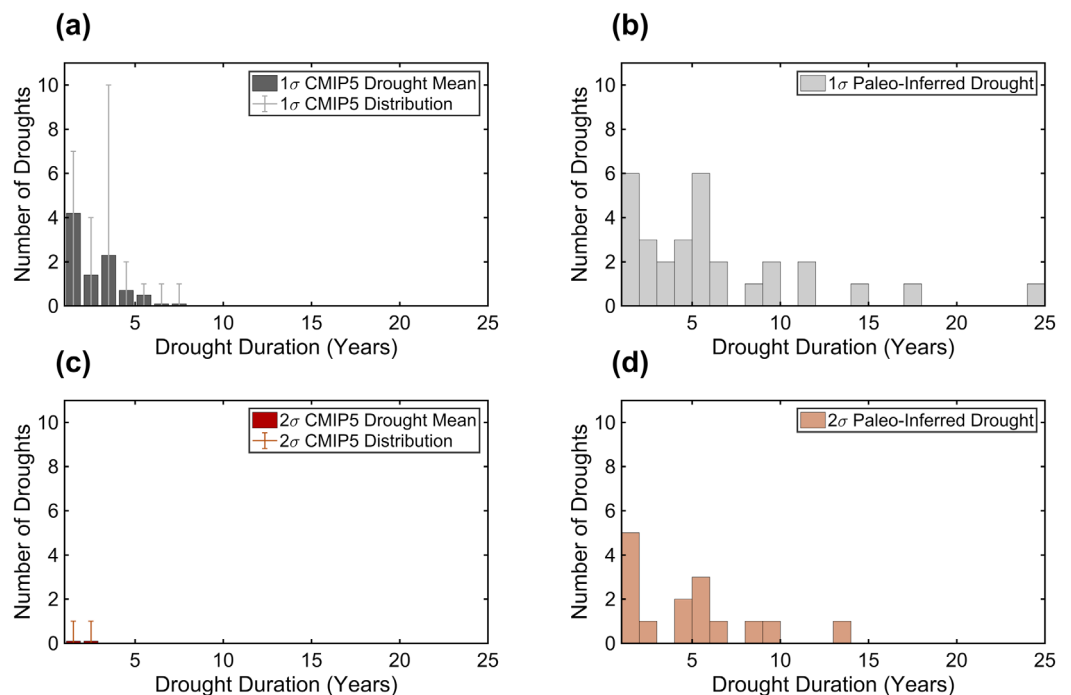
Figure 6. Lake Limón PC1 and simulated western Amazonian drought distributions over the last millennium. (a) CMIP5 precipitation drought distribution 1σ below 850–1850 CE mean. (b) Lake Limón PC1 drought distribution 1σ below mean. (c) CMIP5 precipitation drought distribution 2σ below mean. (d) Lake Limón PC1 drought distribution 2σ below mean (Methods). Individual CMIP5 model minimum and maximum number of drought events shown with vertical lines in (a) and (c).
