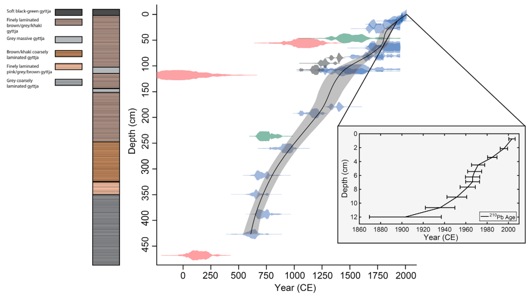
Figure 2. Lake Limón stratigraphy and age model, including radiocarbon and ^{210}\text{Pb} ages. “Best fit” age model produced in clam with a 2\text{-}\sigma age envelope. Dates in blue were used to create the final age model. Dates in tan were excluded due to small size. Dates in green were considered outliers and thus excluded. Dates in dark gray were taken on bulk sediment and were thus excluded. Inset shows ^{210}\text{Pb} dates with 1\text{-}\sigma error bars.
