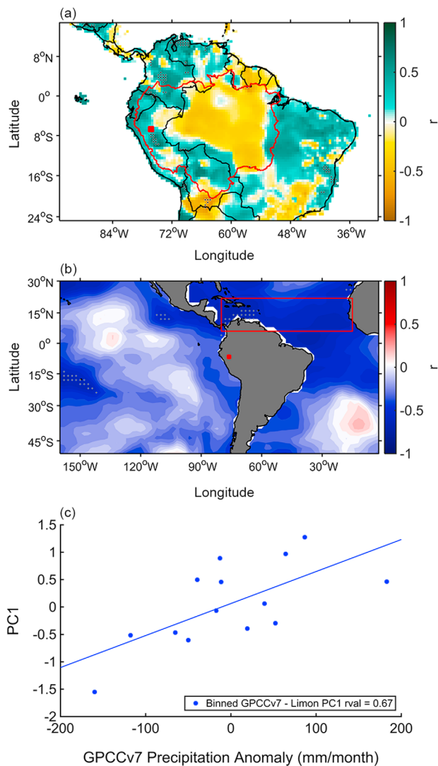
Figure 4. Correlations between Lake Limón PC1 and observations of precipitation and sea-surface temperatures. (a) Correlation coefficient between Lake Limón PC1 and September–March GPCCv7 (Schneider et al., 2014) precipitation (5-year bins). (b) Correlation coefficient between Lake Limón PC1 and annual mean NOAA ERSSTv4 (Huang et al., 2015) sea-surface temperatures (5-year bins). Stippling in both panels marks regions with significant correlations ( p < 0.05 ). Correlations calculated during the time periods 1901–1972 CE (GPCCv7) and 1854–1972 CE (ERSSTv4). Red square in South America indicates the location of Lake Limón. Red line (a) outlines the Amazon drainage basin, and red box (b) outlines tropical North Atlantic region used for correlation with Lake Limón PC1. Scatter plot (c) shows the relationship between the 5-year binned Lake Limón PC1 and 5-year binned GPCCv7 precipitation anomalies (see Table 1 for region used to make GPCCv7 precipitation time series).
