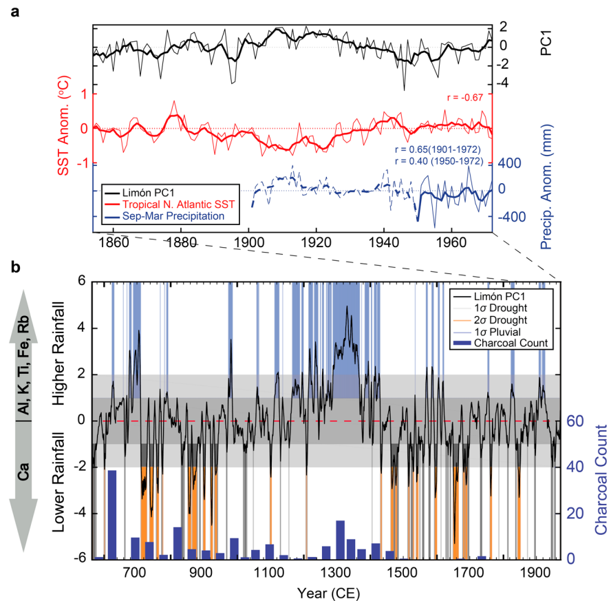
Figure 5. Lake Limón first principal component of elemental variation, Lake Limón charcoal count, tropical Atlantic SST, and local wet-season precipitation. (a) First principal component of Lake Limón hydroclimatic variability, plotted in black (5-year bins), tropical North Atlantic SST plotted in red (6–22°N and 80–15°W, 5-year bins), and wet-season precipitation plotted in blue (8°–7°S, 77°–76°E, 5-year bins, September–March, dashed line indicates poor data coverage before 1950 CE). Correlation coefficients between Lake Limón and 5-year bins of each time series shown above associated time series. (b) First principal component of Lake Limón hydroclimatic variability, plotted in black as a 5-year moving average, ~564 to 1972 CE. Long-term mean shown as dotted line at zero. Dark and light shaded boxes outline one and two standard deviations above and below the mean. Vertical shaded gray lines show dry periods below one standard deviation, vertical shaded brown lines show dry periods below two standard deviations, and vertical blue shaded lines show wet periods above one standard deviation in western Amazonia. Arrows indicate major elemental contributions to Lake Limón principal component. Lake Limón principal component and instrumental observations shown as 5-year bins to account for lake age model uncertainty. Charcoal concentration data (blue vertical bars; see Materials and Methods) shown in 40-year bins to account for age uncertainty associated with cross-core correlation within Lake Limón.
