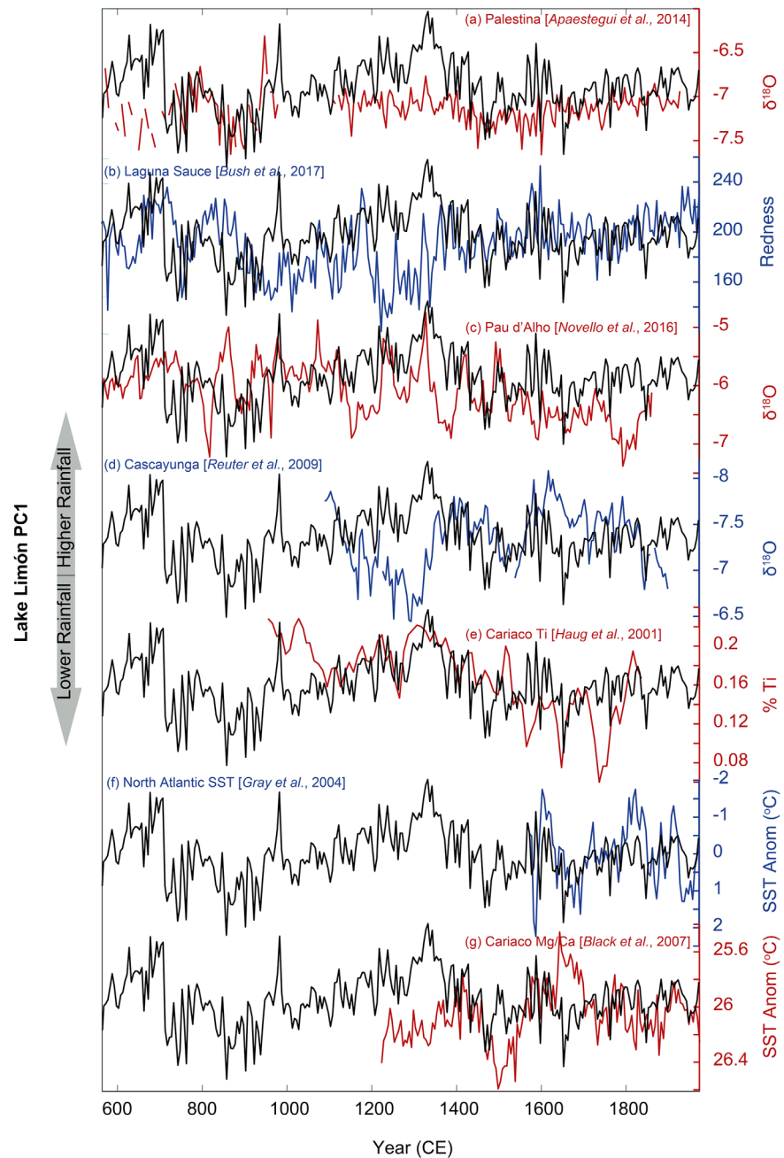
Figure 8. Lake Limón PC1 (black lines) and other tropical South American paleoclimate records (colored lines). (a) Palestina speleothem \delta^{18}\text{O} (Apaestegui et al., 2014), (b) Laguna Sauce sediment redness (Bush et al., 2017), (c) Pau d'Alho speleothem \delta^{18}\text{O} (Novello et al., 2016) (d) Cascayunga speleothem \delta^{18}\text{O} (Reuter et al., 2009), (e) Cariaco Basin %Ti record (Haug et al., 2001), (f) NATL SST tree-ring reconstruction (Gray et al., 2004), and (g) Cariaco Basin Mg/Ca SST anomalies (Black et al., 2007). Note reversed axes on panels d, f, and g.
