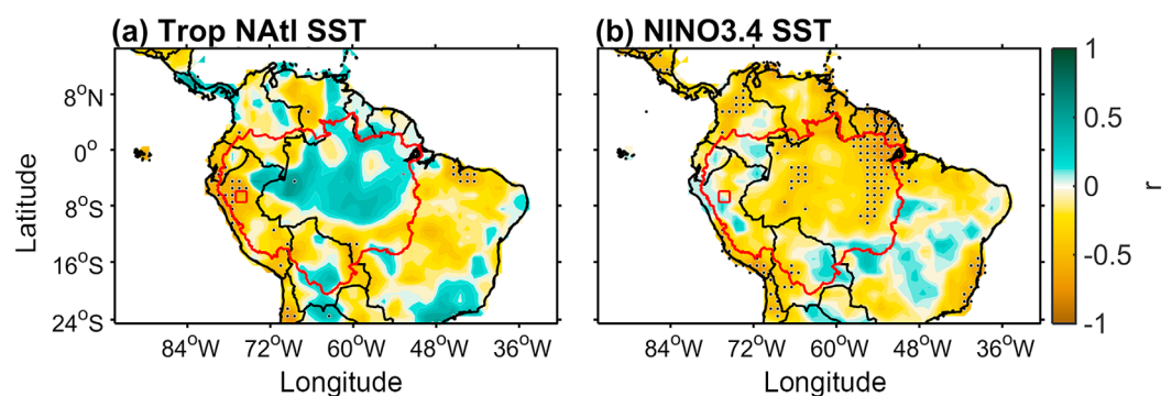
Figure 3. Correlation between sea-surface temperature and September–March interannual precipitation 1901–2014 CE. (a) Tropical North Atlantic (NAtl) SST and September–March precipitation and (b) Niño3.4 SST and September–March precipitation 1901–2014CE. Red box marks location of Lake Limón, red line outlines the Amazon River drainage basin, and black dots indicate correlations at the 95% significance level. All correlations calculated using 5-year bins to match with proxy-observation correlation analysis.
