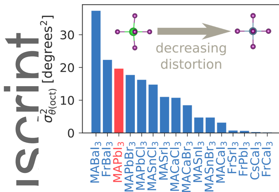
Figure 6. Bond-angle variance of several inorganic and hybrid halide perovskites. The calculations were done using LDA assuming the cubic phase.
