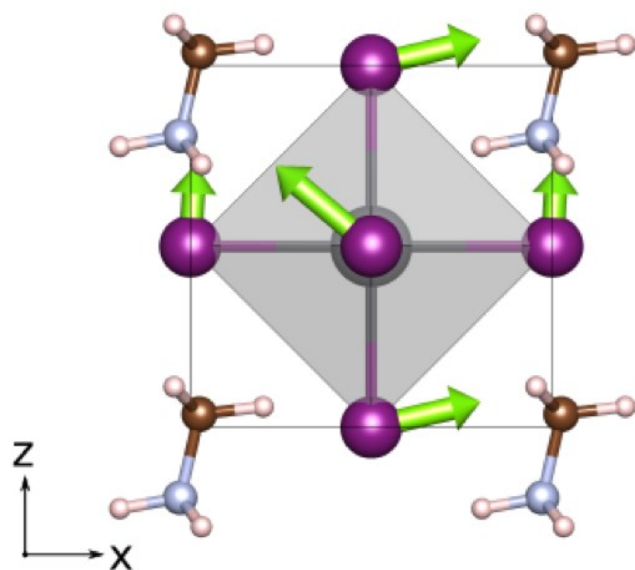
Figure 1. 12-atom unit cell of \text{MAPbI}_3 where the I atoms are at the ideal face-center positions. The arrows indicate displacement of the I atoms upon relaxation within a cubic cell shape. For clarity the length of the displacement vector is enhanced by a factor of five.
