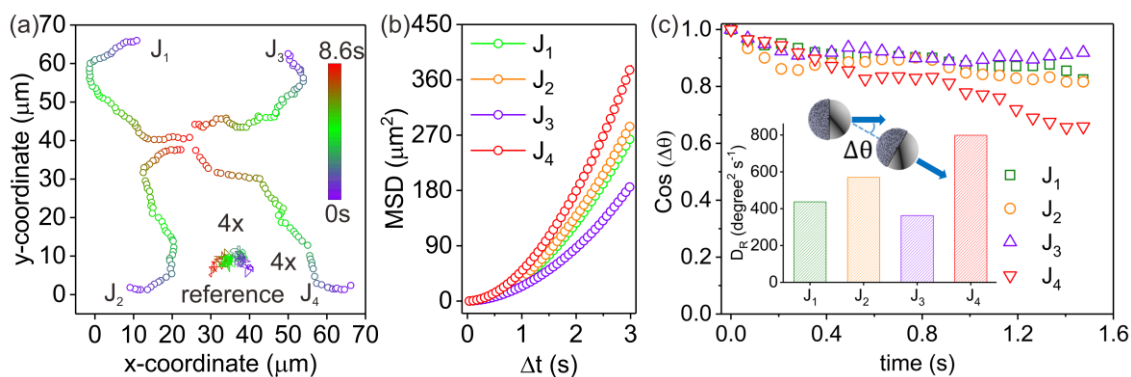
Figure 3. (a) Trajectories of four single Janus PS/Ag/AgCl particles ( J_1 - J_4 ) taken over 8.6 s under blue light illumination [ (106 \pm 1) \mu\text{W} / \text{mm}^2 ]. The trajectory of a reference Janus PS/Ag/AgCl particle under green light illumination [ (8 \pm 1) \mu\text{W} / \text{mm}^2 ] is shown as well (video S1). (b) The experimental MSD curves of single Janus particles: J_1 ( 1193 \mu\text{m}^2 , green symbols), J_2 ( 1460 \mu\text{m}^2 , orange symbols), J_3 ( 940 \mu\text{m}^2 , purple symbols), and J_4 ( 2899 \mu\text{m}^2 , red symbols) (video S1). (c) Time evolution of the experimental autocorrelation values, \text{Cos}(\Delta\theta) , of the angle \Delta\theta , capturing the change of the orientation of the main symmetry axis of the metallic cap of a colloid between two neighboring frames in the tracking video files for the single Janus PS/Ag/AgCl particles ( J_1 - J_4 ). The upper inset shows schematics on how the angle \Delta\theta is defined. The lower inset summarizes the rotational diffusion coefficients, D_R , for four single Janus particles (video S2).
