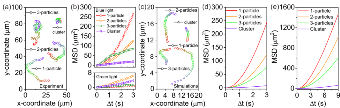
Figure 5. (a) Trajectories and (b) the corresponding experimental MSD curves of different Janus particle assemblies (one, two, three particles, and a cluster consisting of around 30 particles) taken over about 3 s under blue light illumination [(106 \pm 1) \mu\text{W}/\text{mm}^2] . (c) Simulated trajectories and the corresponding simulated MSD curves for different Janus particle assemblies (one, two, three particles, and a small cluster) taken over (d) 3 s and (e) 9 s.
