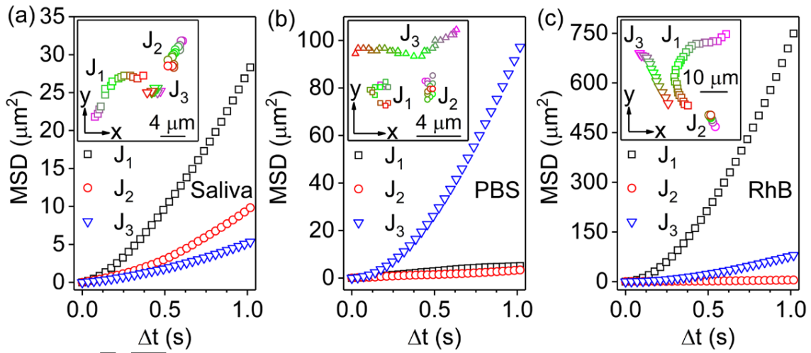
Figure 6. Trajectories (insets; taken for 1 s) and the corresponding experimental MSD curves of different Janus particle assemblies (J 1 : single Janus particle; J 2 : 2-particles assembly; and J 3 : big cluster of Janus particles) in (a) human saliva solution (100 times diluted) (video S5), (b) PBS solution (0.01 mM) (video S6), and (c) RhB solution (100 mM) (video S7), under blue light illumination [(106 ± 1) \mu\text{W}/\text{mm}^2 ].
