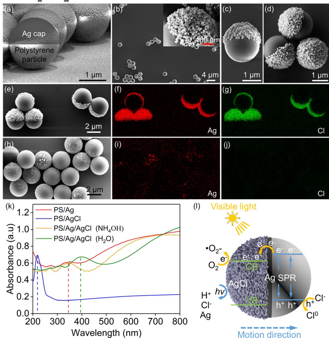
Figure 1. Scanning electron microscopy (SEM) images of (a) as prepared PS/Ag capped particles, (b) PS/Ag/AgCl Janus particle assemblies. The insert in panel (b) shows a high-resolution SEM image of the Ag/AgCl surface. Zoom on a location with (c) a single Janus particle, (d) cluster of 3-Janus particles, and (e) clusters of 2- and 3-Janus particles. The EDX mapping of (f) Ag and (g) Cl elements for the sample shown in panel (e). (h) SEM image of PS/Ag/AgCl Janus particles processed in ammonia solution and the corresponding EDX mapping of (i) Ag and (j) Cl elements. (k) UV-vis absorption spectra of PS/Ag (red curve), PS/pure AgCl (blue curve), PS/Ag/AgCl (green curve), and
