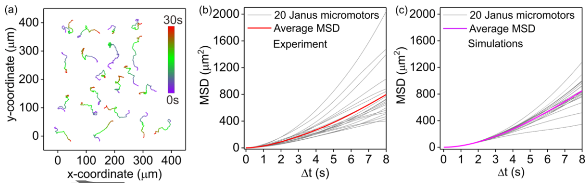
Figure 2. (a) Trajectories of 20 single Janus PS/Ag/AgCl particles taken over 30 s under blue light illumination [ (106 \pm 1) \mu\text{W} / \text{mm}^2 ]. (b) The individual (grey) and averaged (red) experimental MSD curves of 20 single Janus particles. (c) Representative individual (grey) and averaged (magenta) simulated MSD curves of 20 single Janus particles.
