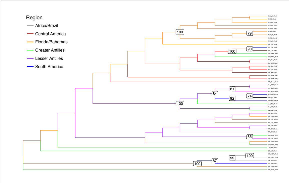
Supplemental Figure 2. RAxML trees using chloroplast data for white mangroves ( Laguncularia racemosa ; top) and red mangroves ( Rhizophora mangle ; bottom). Bootstrap percentages greater than 70% are indicated at each node.
