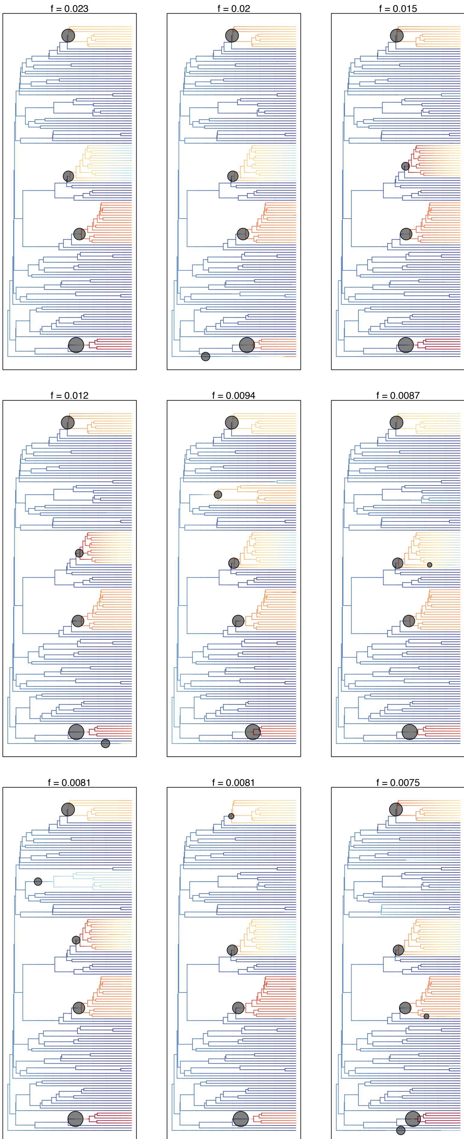
Appendix S15. Set of nine shift configurations with the highest posterior probability from BAMM analysis. Significant shifts in diversification are identified by gray dots, with warm colors denoting relatively high rates of diversification and cool colors relatively low rates of diversification. The phylogenies are ladderized to match the clade orientation in Fig. 3. f = frequency of configurations among the post burn-in posterior.
