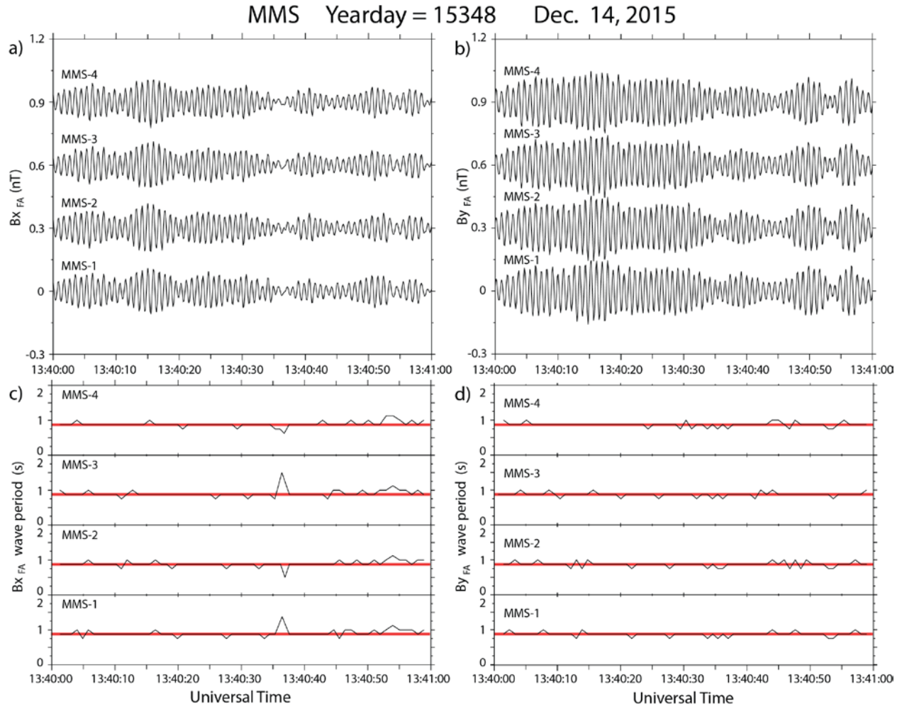
Figure 10. Waveforms and wave periods of EMIC waves observed by the four MMS spacecraft between 1340 and 1341 UT December 14, 2015, as in Figure 8. A bandpass filter between 0.8 and 2.0 Hz has been applied to the FGM data.
