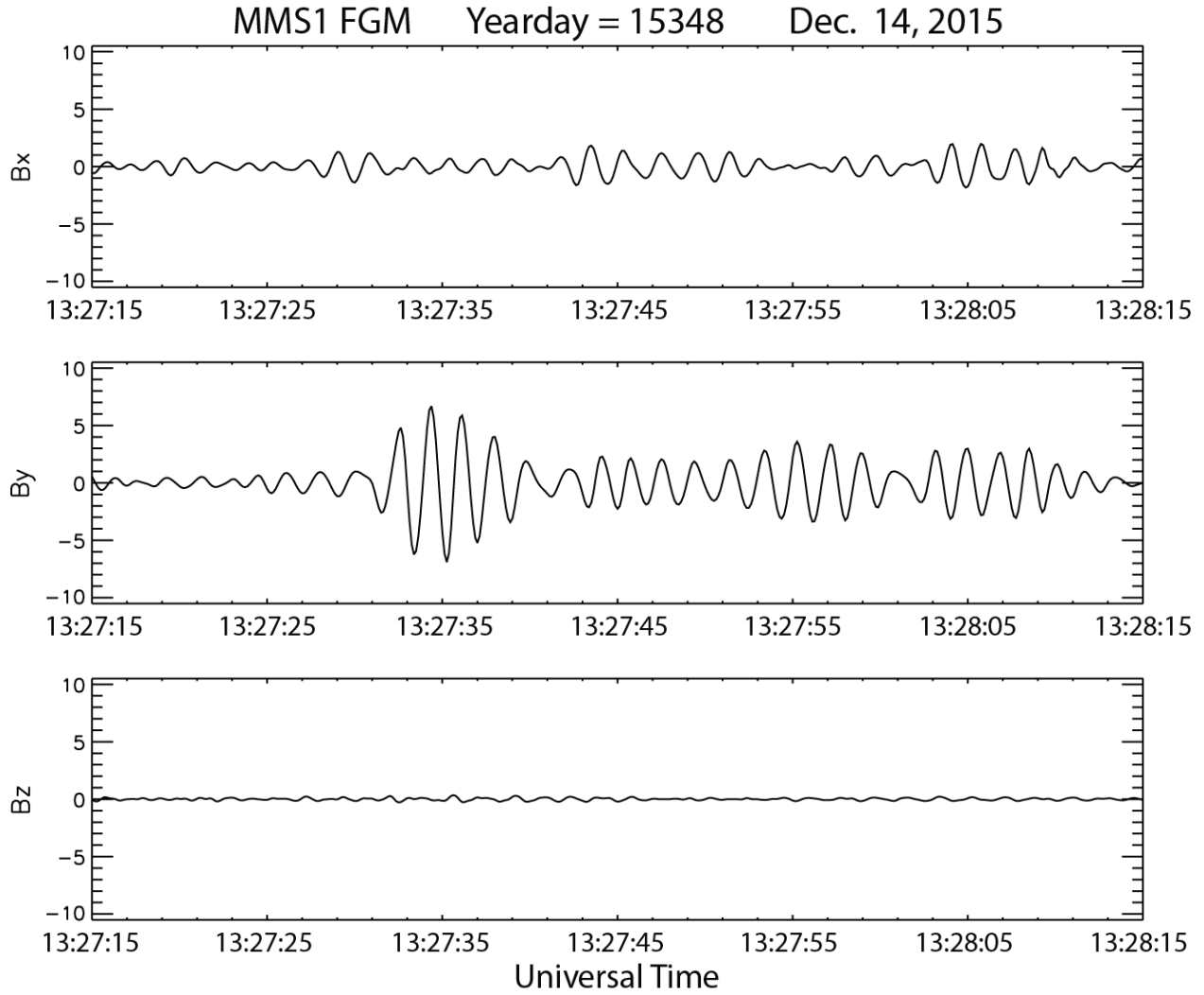
Figure 7. Three-axis plot of MMS 1 magnetic field data rotated into local field-aligned coordinates and bandpass filtered from 0.4 to 2.0 Hz, with uniform scale, from 1327:15 to 1328:15 UT December 14, 2015.
