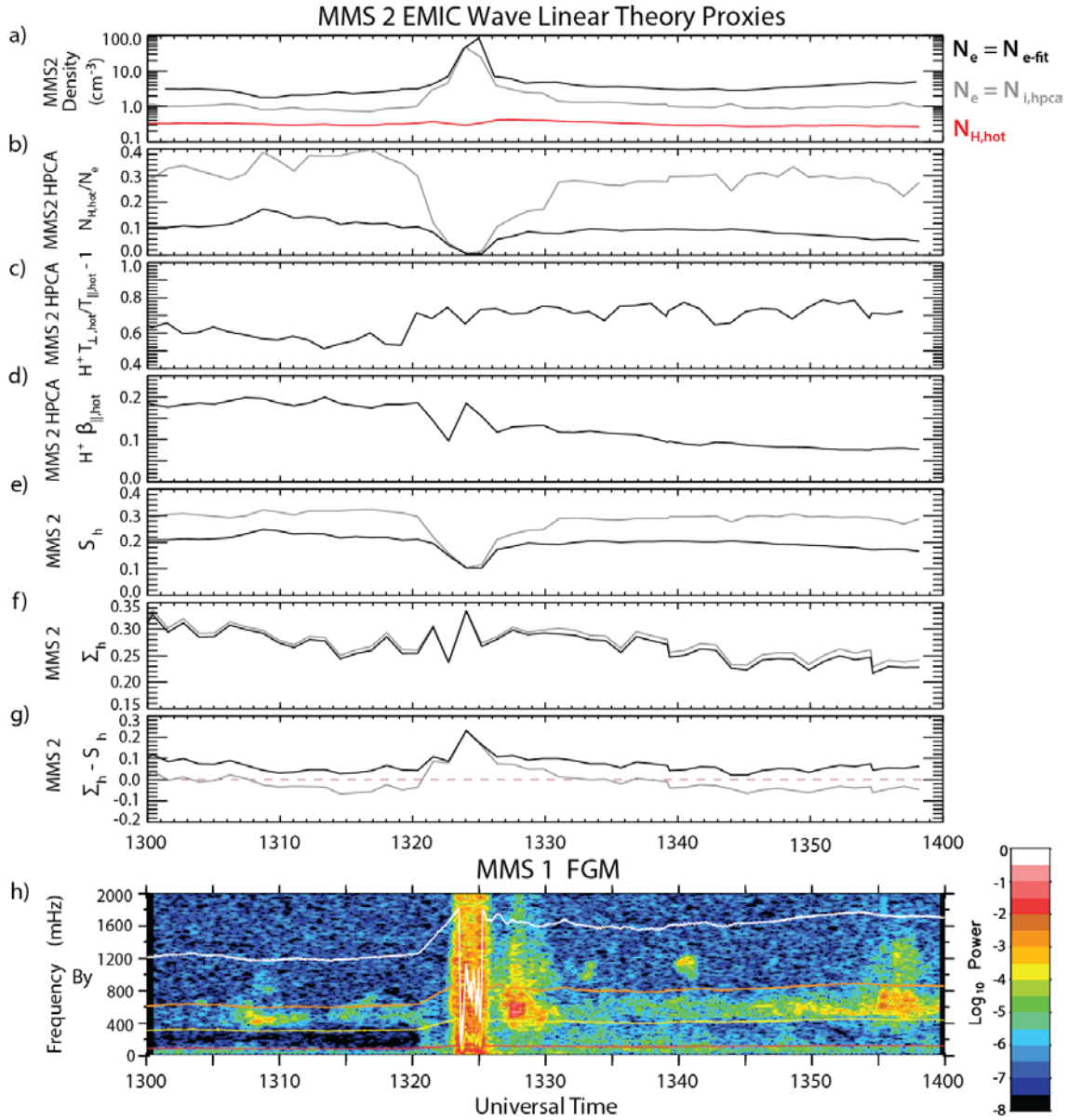
Figure 13. EMIC linear theory proxies calculated from MMS 2 data. Panel a: Total plasma densities determined using the spacecraft potential (black line) and the total ion density measured by HPCA (grey line), and hot plasma density (red line). Panel b: Ratios of hot proton density to total plasma density, calculated using total plasma densities determined from the spacecraft potential (black) and the total ion density measured by HPCA (grey). Panel c: Anisotropy of hot protons (10 keV – 40 keV) measured by the HPCA instrument on MMS 2. Panel d: Plasma beta of hot ions parallel to the magnetic field. Panel e: Theoretical Blum et al. (2009) instability
