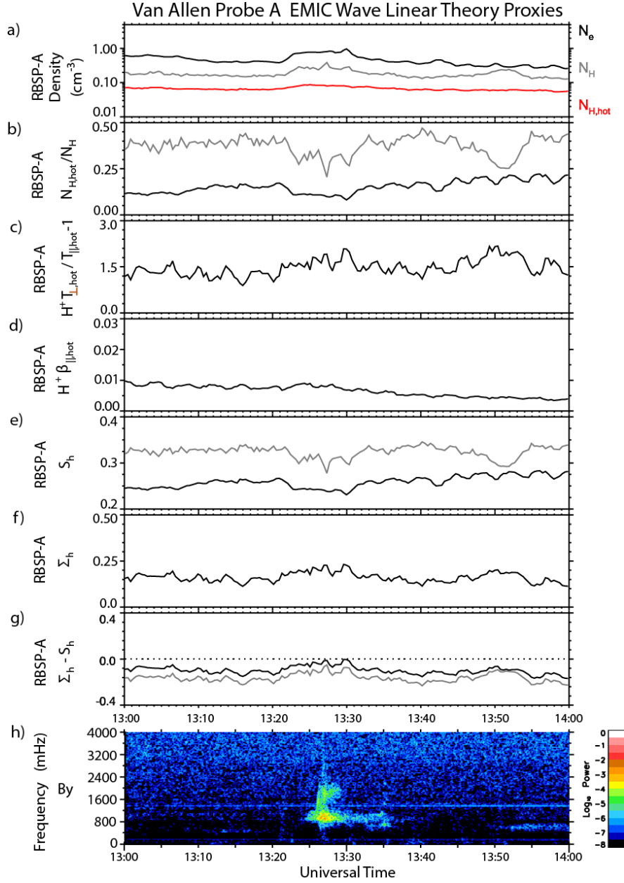
Figure 16. EMIC linear theory proxies calculated from Van Allen Probes A (RBSP-A) data. Panel a: Total plasma densities determined using the HOPE electron density (black line) and HOPE proton density (grey line), and hot plasma density ((3 to 30 keV, red line). Panel b: Ratios of hot proton density to total proton densities measured by HOPE (electrons, black line and protons, grey line). Panel c: Anisotropy of 10 eV - 30 keV protons measured by HOPE.
