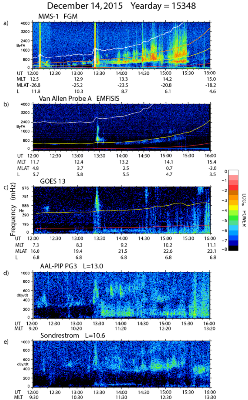
Figure 4. Fourier spectrograms of differenced magnetic field data from MMS 1, Van Allen Probe A, GOES 13, AAL-PIP PG3, and Sondrestrom, Greenland from 12:00 to 16:00 UT December 14, 2015. Panels a and b show the transverse azimuthal component of satellite fluxgate magnetometer data rotated into field-aligned coordinates, panel c shows the radial (He) component of satellite fluxgate magnetometer data, and panels d and e show the east-west
