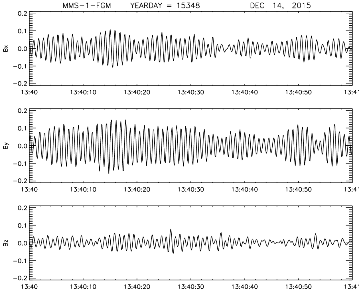
Figure 9. Three-axis plot of MMS 1 magnetic field data rotated into local field-aligned coordinates and bandpass filtered from 0.8 to 2.0 Hz, with uniform scale, from 1340 to 1341 UT December 14, 2015.
