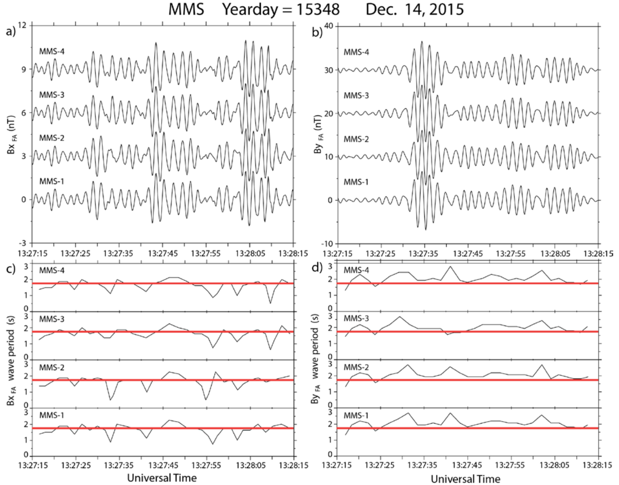
Figure 8. Waveforms and wave periods of EMIC waves observed by the four MMS spacecraft between 1327:15 and 1328:15 UT December 14, 2015. A bandpass filter between 0.4 and 2.0 Hz has been applied to the FGM data. Panels a and b show the Bx (transverse radial) and By (transverse azimuthal) components of the magnetic field in local field-aligned coordinates, respectively, offset by 3 nT and 10 nT in the vertical direction. Panels c and d show the corresponding wave periods of the Bx and By components, respectively, at each of the four spacecraft. Shaded lines are drawn at 1.75 Hz in panel c and panel d.
