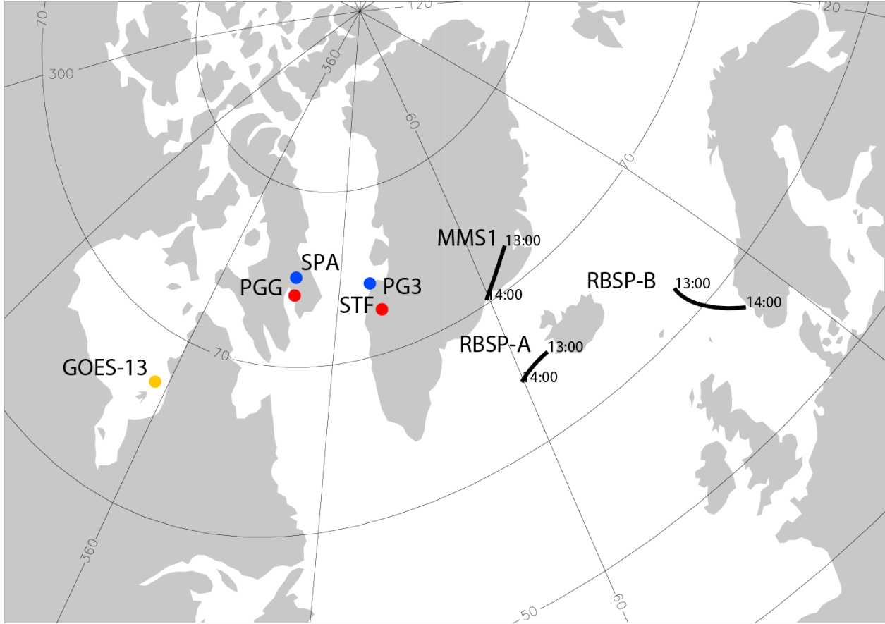
Figure 2. The black lines show the northern hemisphere footpoints of the magnetic field lines traversed by MMS 1 and Van Allen Probes A and B between 1300 and 1400 UT December 14, 2015, and the orange dot shows the northern hemisphere footpoint of GOES-13. Red dots indicate the locations of northern hemisphere ground magnetometers at Sondrestromfjord, Greenland (STF) and Pangnirtung, Canada (PGG); blue dots indicate the northern hemisphere locations conjugate to South Pole Station (SPA) and AAL-PIP station PG3 in Antarctica.
