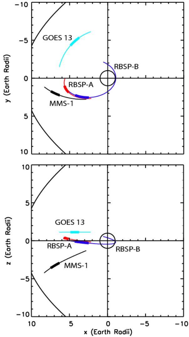
Figure 1. Segments of the orbits of MMS 1 (black), Van Allen Probes-A (red) and -B (dark blue), all traveling inbound, and GOES 13 (light blue), shortly after local noon between 1200 and 1600 UT on December 14, 2015, in the SM (solar magnetic coordinate system) XY and XZ
