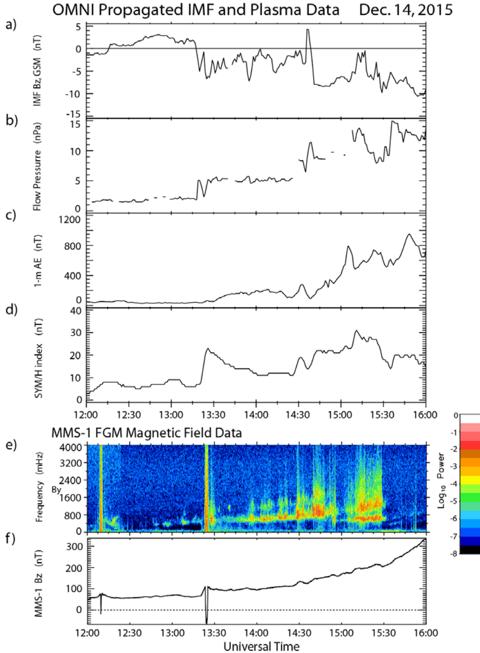
Figure 3. Panels a-d show data from the OMNI database from 1200 to 1600 UT December 14, 2015. Panel a shows the north-south component of the IMF ( B_z ) and panel b the solar wind flow pressure ( P_{sw} ), both propagated in time to the bow shock. Panel c shows the 1-min AE index,
