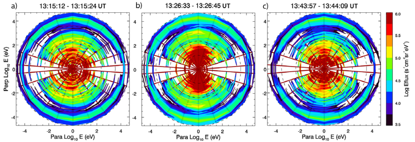
Figure 15. Proton data from the HOPE instrument on Van Allen Probe A on December 14, 2015. Panels a-c show two-dimensional distributions of the proton flux at 1315 UT, before the magnetospheric compression (panel a); at 1326 UT, near the time of the peak compression of the magnetic field and during the EMIC wave event (panel b); and at 1343 UT, after the compression (panel c).
