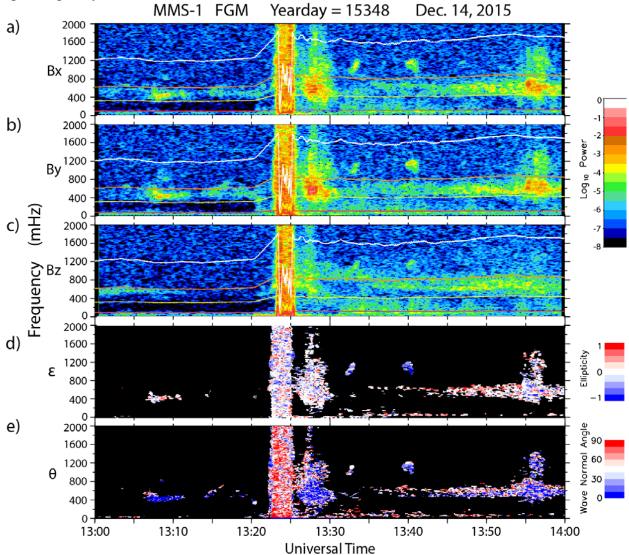
Figure 5. Fourier spectrograms of differenced magnetic field data from MMS 1 from 1300 to 1400 UT December 14, 2015. Panels a, b, and c show the wave power as a function of frequency (in mHz) in local field-aligned coordinates ( B_x radial, B_y azimuthal, and B_z parallel to the total field), respectively. Panel d shows the ellipticity (-1 for left-handed circularly
