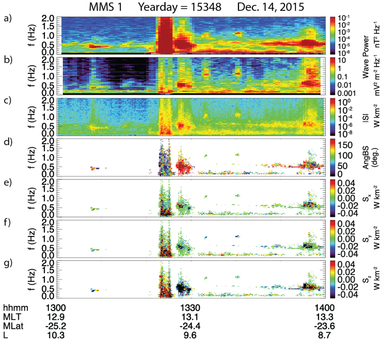
Figure 6. Frequency vs. time spectrograms from 1300 to 1400 UT December 14, 2015 of total wave power in the magnetic field B (panel a), electric field E (panel b), and the magnitude of the Poynting vector S (panel c). Panel d shows the angle between the Poynting vector and the background magnetic field, and panels e-f show the components of the Poynting flux S in the field-aligned coordinate X, Y, and Z directions.
