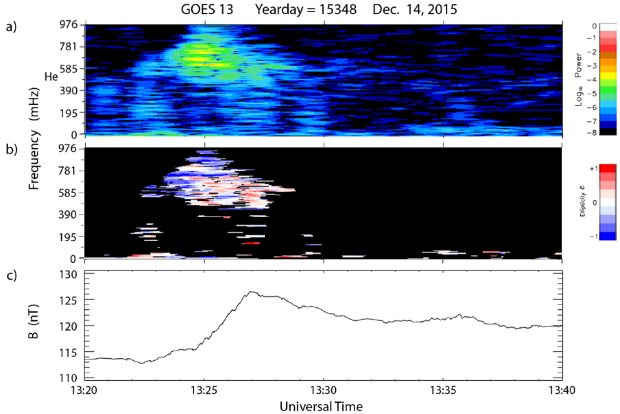
Figure 17. GOES 13 magnetic field data from 1320 to 1340 UT December 14, 2015. Panel a: frequency vs. time spectrogram of He (earthward) component magnetic field data. Panel b: wave ellipticity. Panel c: total magnetic field.
