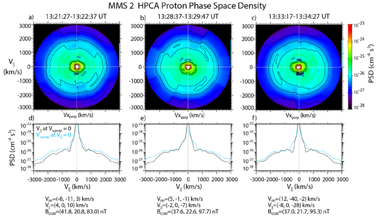
Figure 12. Proton phase space density distributions measured by the MMS 2 HPCA instrument before the magnetosheath intrusion (13:21:27-13:22:37 UT), 2 min after the retreat of the magnetosheath and during the most intense EMIC wave activity (13:28:37-13:29:47 UT), and ~5 min later, from 13:33:17 to 13:34:27 UT. Panels a-c show color-coded 2D distributions as a function of velocity parallel to the magnetic field (vertical axis) and perpendicular to it (horizontal axis), and panels d-f show 1D traces of the PSD in these two directions.
