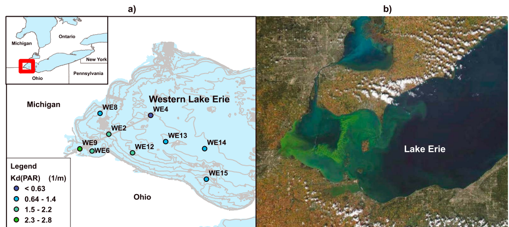
Figure 1. (a) Map of the western Lake Erie study area and weekly monitoring stations, showing mean k_{d(\text{PAR})} by station from this study, 1-m bathymetry contours, and (b) satellite image showing typical spatial variation in water quality during summer in western Lake Erie (NASA MODIS imagery and NOAA CoastWatch, taken 30 September 2014).
