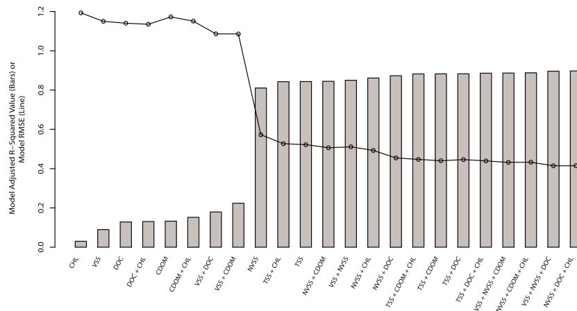
Figure 7. Performance ranking of linear regression models for k_d(PAR) . Models were ranked by adjusted R -squared (bars) and 10-fold cross-validation RMSE (line) values.
