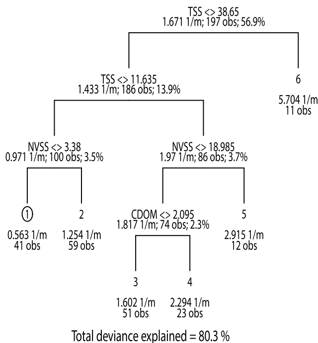
Figure 6. Regression tree analysis results showing relative influence of TSS, VSS, NVSS, DOC, CDOM, and CHL on k_d(\text{PAR}) , showing significant impacts of TSS, NVSS, and CDOM.
