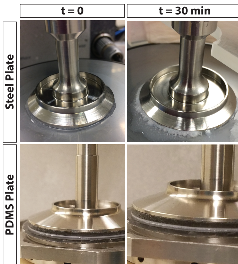
Figure 3S-4. Comparison of O 2 bubble nucleation from H 2 O 2 decomposition in steel fixtures and PDMS modified fixtures. O 2 bubbles nucleate and grow in steel fixtures. With PDMS modified steel fixtures, O 2 can diffuse into PDMS film, which helps prevent the development of O 2 bubbles.
