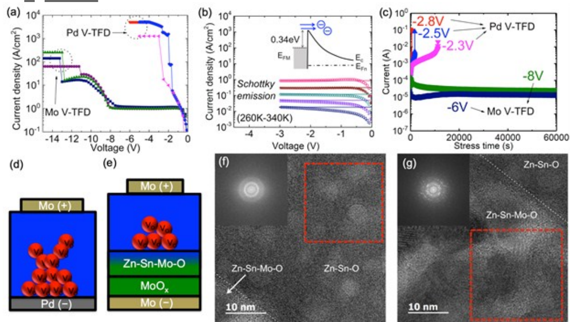
Figure 3. (a) Breakdown voltage (BV) > 10 V measured on Mo V-TFDs with various electrode sizes (diameter of 30 \mu\text{m} , 50 \mu\text{m} , and 100 \mu\text{m} ). BV measured on Pd V-TFDs with the same sizes are also shown for comparison. (b) Temperature-varying reverse J - V measurements (symbols) of Mo V-TFDs. The bias-independent reverse current obeys Schottky emission over a potential barrier of 0.34 eV without image force lowering (solid lines). The charge transport analysis on forward current is shown in Figure S4 in Supporting Information. (c) Reverse bias stress in Mo V-TFD and Pd V-TFD. Unlike the Pd V-TFD, which was tested at < 3 V magnitude, the Mo V-TFD were tested at a higher reverse voltages, 6 V and 8 V, and still did not show any increase in leakage current. After the stress test, the Mo V-TFD still maintained its rectifying behavior as shown in the Figure S5 in Supporting Information. (b) and (c) are from 100 \mu\text{m} -diameter diodes. (d) In Pd V-TFD, oxygen vacancy defects ( V_{\text{O}} in red circles) accumulate near the Pd layer, which causes an increase in leakage current and premature breakdown, as shown in (c). (e) In the Mo V-TFD, the Zn-Sn-Mo-O layer prevents V_{\text{O}} defects from accumulating near the \text{MoO}_x Schottky layer, preventing an increase in leakage current and resulting in a higher BV, as shown in (c). (f) and (g) show HRTEM images near Zn-Sn-O/Zn-Sn-Mo-O interface. The interface is marked with a white dotted line. The regions for FFT analysis are marked with red dashed lines and the corresponding FFT patterns are shown in the insets. Zn-Sn-O shows an amorphous morphology in (f) while Zn-Sn-Mo-O is polycrystalline (g).
