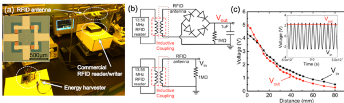
Figure 6. (a) Wireless energy harvesting experimental setup. A commercial HF (13.56 MHz) RFID antenna and reader with 200 mW output power were placed in parallel. The power from the reader was wirelessly harvested using the antenna while the distance between them was varied. The antenna was attached via SMA connection to an FWR wire-bonded onto a PCB with surface-mount loads. The DC output voltage of the FWR was measured with an oscilloscope. The inset shows a microscope image of a FWR with four 100\ \mu\text{m} \times 100\ \mu\text{m} V-TFDs. (b) Circuit diagrams showing the wireless energy harvesting measurement setup (top). To compare the measured V_{out} with V_{in} , V_{in} was measured as the voltage across a 1\ \text{M}\Omega resistor attached to the antenna, without the rectifier included (bottom). The maximum peak-to-peak V_{in} obtained at a distance of 0 mm was \sim 8.7\ \text{V} , which gives P_{out} = V_{rms}^2/50\ \Omega \approx 190\ \text{mW} , close to the maximum output power of the reader. (c) The magnitude of V_{in} and V_{out} as a function of separation distance. V_{out} exceeds over V_{in} when the distance is < 10\ \text{mm} , which is attributed to resonance due to mutual inductance. The inset shows V_{in} and V_{out} measured over time with the antenna and reader separated by a distance of 21 mm.
