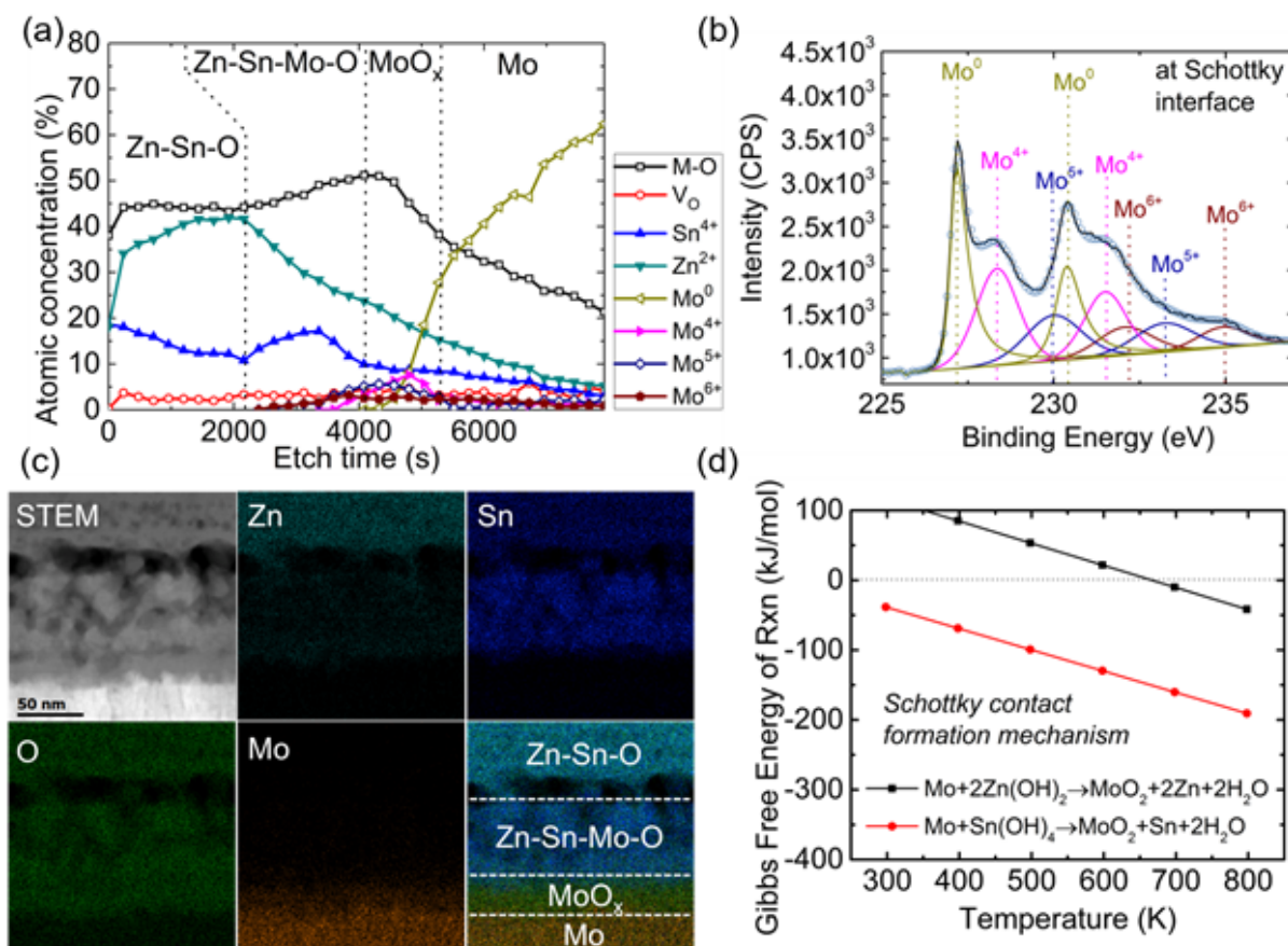
Figure 2. (a) XPS depth profile of bottom Mo/ a -Zn-Sn-O deposited on Si substrate. In between the Mo and a -Zn-Sn-O, layers of MoO x and Zn-Sn-Mo-O appear. (b) XPS Mo 3d core level analysis of the MoO x layer, which corresponds to an etch time of 4800 s in (a). Hollow circles indicate the summation of the de-convoluted peaks, which overlaps with the measured curve. Details of XPS core-level analysis methods are described in Section S1 in Supporting Information. (c) Cross-sectional STEM dark-field image and EDS elemental mapping of Zn (cyan), Sn (blue), O (green), and Mo (orange) elements obtained near Mo/ a -Zn-Sn-O junction. A STEM image of the entire film stack is shown in Figure S1 in Supporting Information. Two additional interfacial layers (i.e., MoO x and Zn-Sn-Mo-O) appear between metallic Mo and Zn-Sn-O, which accords with the XPS depth profile shown in (a). (d) Standard Gibbs free energy of Mo oxidation during solution process of Zn-Sn-O, showing negative values at the film anneal temperature (793 K).
