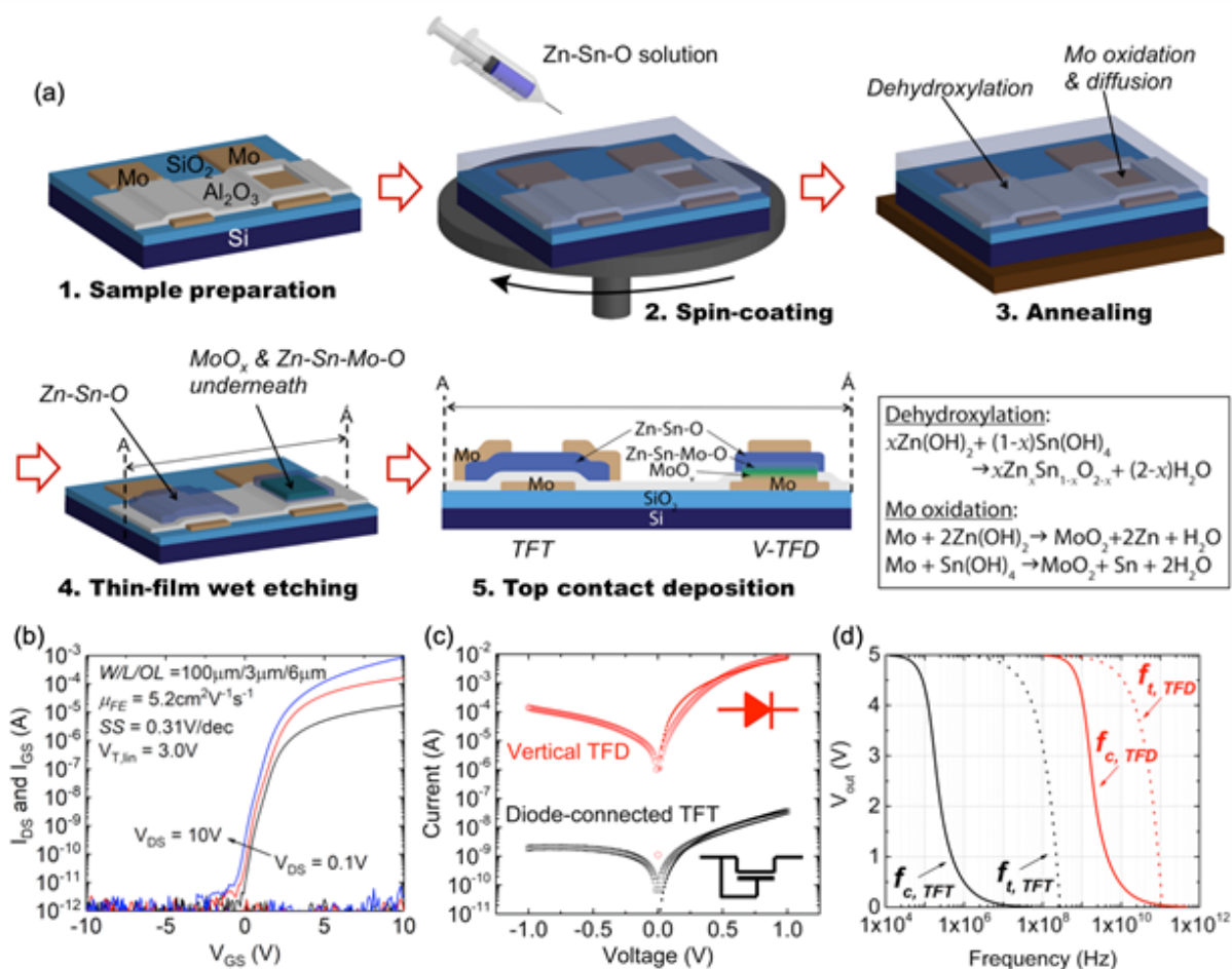
Figure 5. (a) Simplified schematic of simultaneous fabrication of V-TFD and TFT on a single substrate. Thin films with different chemical composition are grown via different chemical evolution during solution deposition of Zn-Sn-O. Specifically, Zn-Sn-O is grown via dehydroxylation on top of \text{Al}_2\text{O}_3 , while Mo oxidation and diffusion occur on top of bottom Mo, creating \text{MoO}_x and Zn-Sn-Mo-O layers in specific regions. A two-dimensional cross-sectional view ( A \leftrightarrow \hat{A} ) of completed devices is shown in step 5. (b) Transfer curves obtained from a TFT with device dimensions of 100\mu\text{m} in width, 3\mu\text{m} in channel length, and 6\mu\text{m} in overlap length, which leads to 100\mu\text{m} \times 100\mu\text{m} in overall size, including source and drain contacts. Output curves are shown in Figure S7c in Supporting Information. (c) Comparison of I - V curves obtained from TFT in (b) with its gate and drain connected, and from V-TFD with 100\mu\text{m} \times 100\mu\text{m} size. Hollow circles and squares are measured data and dotted lines are from the on-current model used to calculate f_{c,TFT} and f_{c,TFD} in (d). (d) Maximum operating frequencies, calculated based on transit time ( f_i ) and measured on-current ( f_c ).
