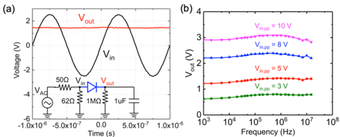
Figure 4. (a) The measurement configuration of the diode in a half-wave rectifier circuit is shown in the inset. An AC input voltage ( V_{AC} ) was generated by a function generator, operated in 50\ \Omega mode and used in parallel with a 62\ \Omega input resistor. In (a), V_{in} (in black) indicates the 1 MHz, 5 V sinusoidal peak-to-peak voltage across the 62\ \Omega input resistor, measured using an oscilloscope. V_{out} (in red) shows the DC output voltage measured across the load. (b) The frequency response of the output voltage measured up to 15 MHz, which is the maximum frequency of the function generator, is shown for different V_{in} peak-to-peak values. Because the diode has BV > 10\ \text{V} , the rectifier can rectify up to peak-to-peak voltage of 10 V. The devices tested here have diameter of 100\ \mu\text{m} .
