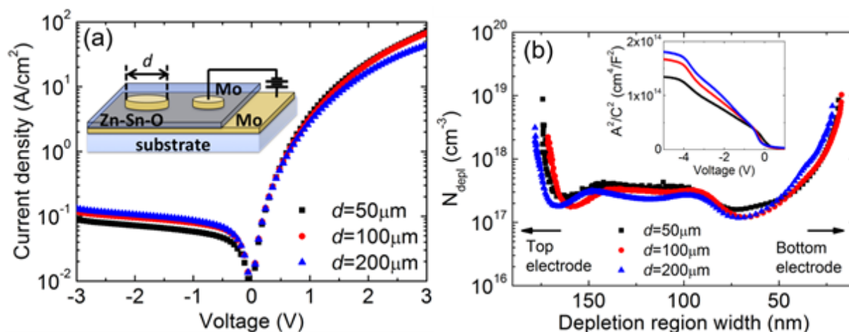
Figure 1. (a) Typical J - V characteristics obtained from Mo: a -Zn-Sn-O diodes with various sizes. The inset shows a schematic of the V-TFDs, where d is the diameter of the top electrode. (b) Depletion concentration ( N_{\text{depl}} ) profile for various size diodes. The corresponding C - V measurements are shown in the inset. C - V characteristics were measured at 1 MHz, across a DC sweep from +1 V to -5 V, with 50 mV of AC voltage, in parallel RC model. Full depletion is achieved at -5 V, which corresponds to a film thickness of 180 nm.
