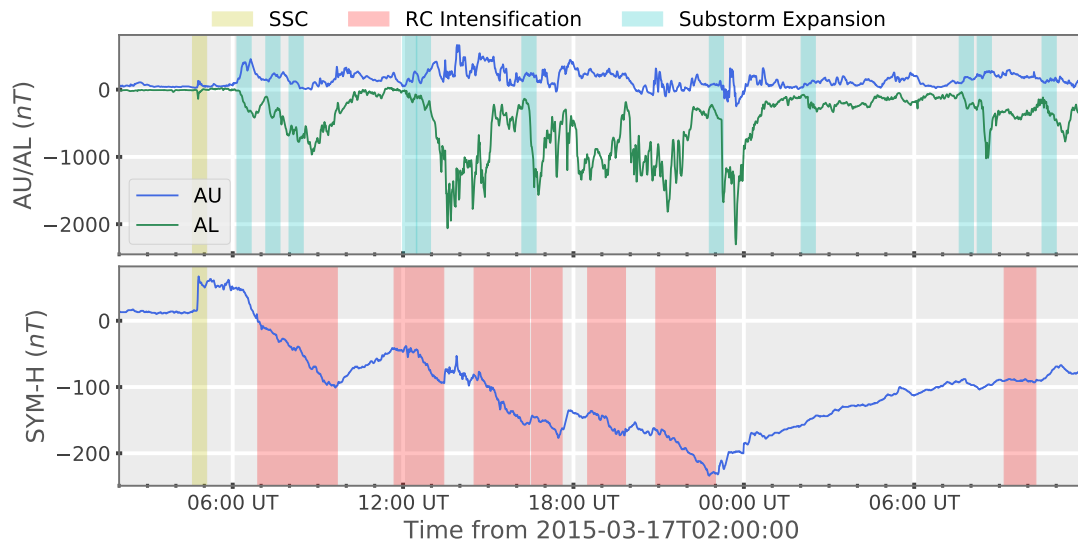
310 Figure 4. AU/AL (top frame) and SYM-H (bottom frame) indexes for validation event 7. Storm sudden 311 commencements, ring current intensifications, and substorm periods are marked by yellow, red, and cyan 312 boxes, respectively.
