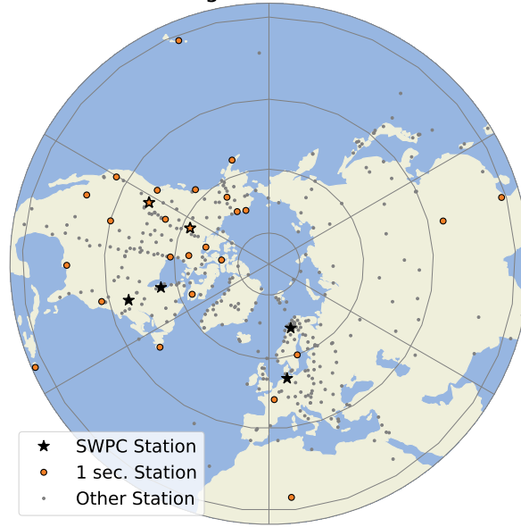
Figure 1. Locations of magnetometer stations used in the original validation suite (black-bordered stars), stations with 1 s data available (orange dots and orange stars), and other stations (grey dots).
