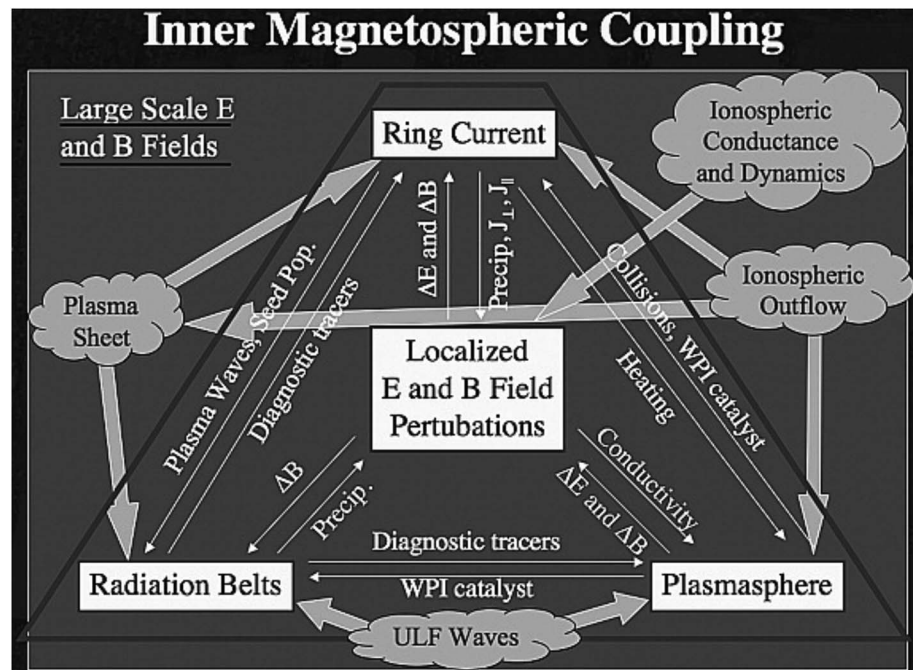
Figure 1. The schematics of inner magnetosphere coupling physics, showing the connection between the electric/magnetic fields with particles, together with other effects (adopted from Liemohn, 2006).
