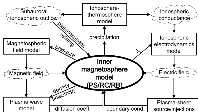
Figure 2. The schematics of the modeling framework for the inner magnetosphere coupling processes. The center is the primary inner magnetosphere model for plasmasphere (PS), ring current (RC), and radiation belt (RB). The surrounding model components represent processes being coupled with the inner magnetosphere populations.
